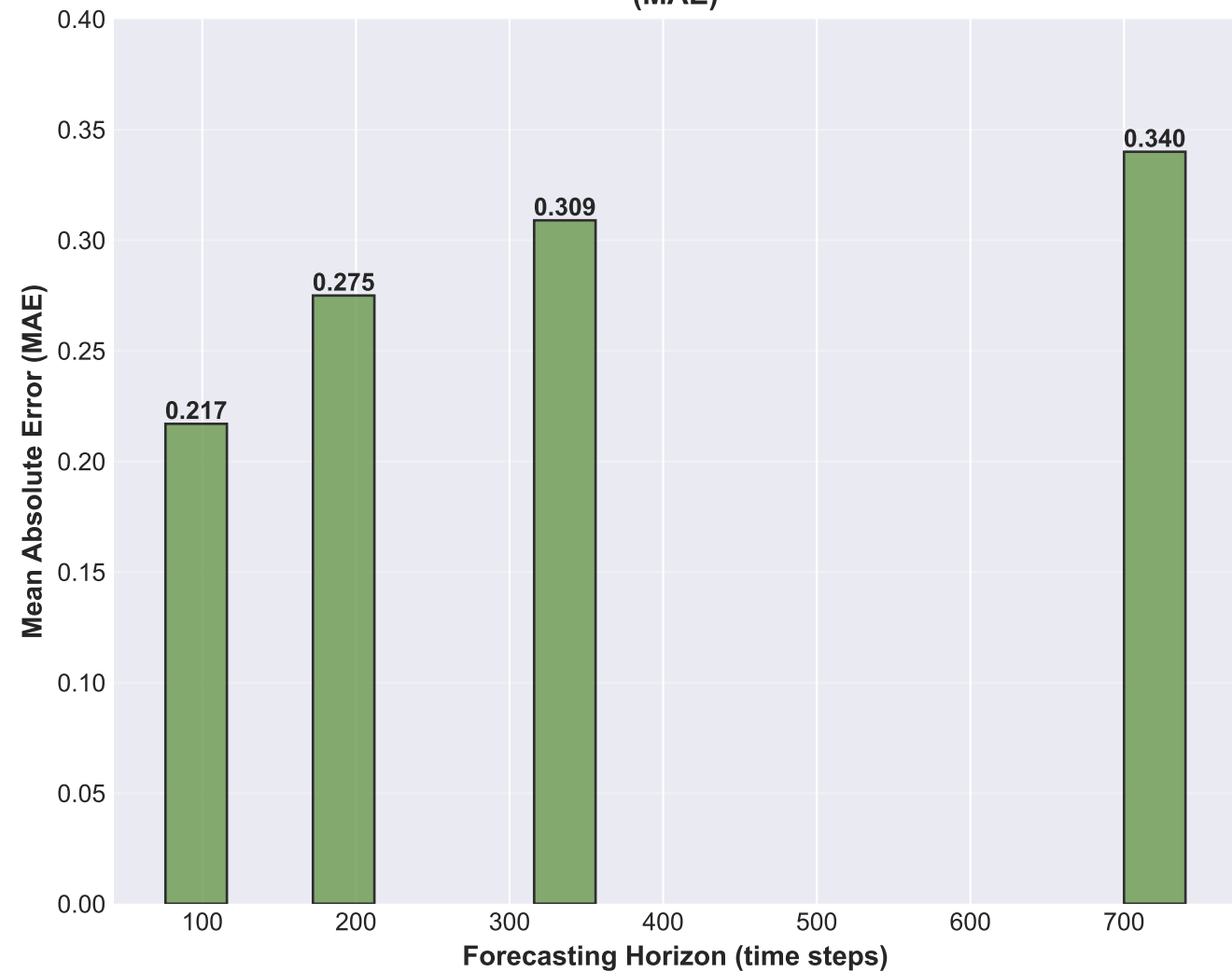
PatchXFormer Performance on USA Kansas Dataset (MAE)
