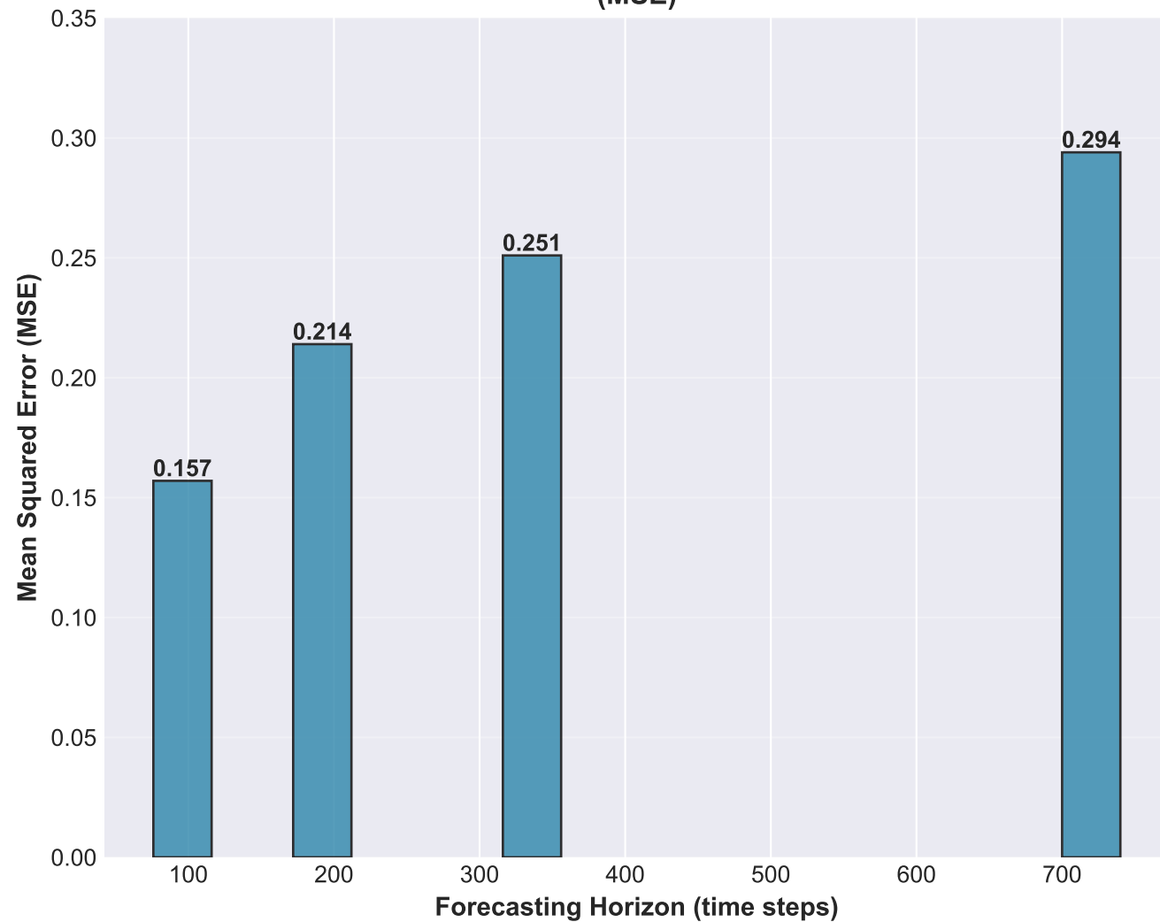
PatchXFormer Performance on USA Kansas Dataset (MSE)
