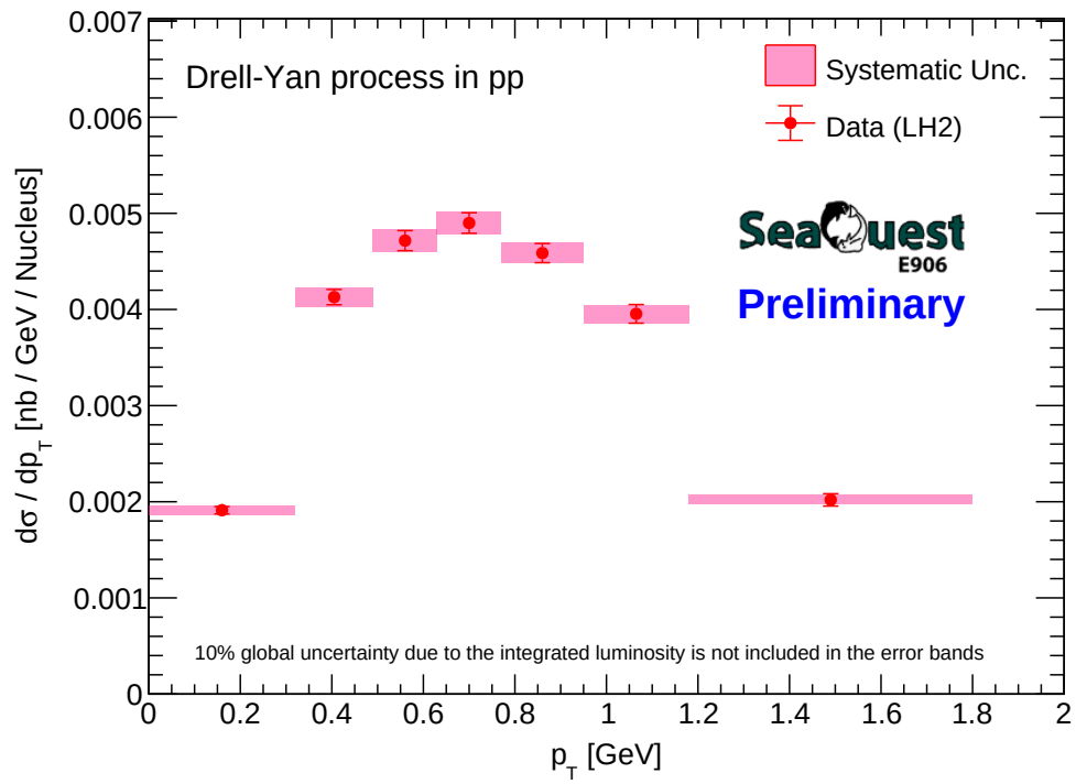
Figure 33: CrossSection_LH2_vs_pT_with_logo
