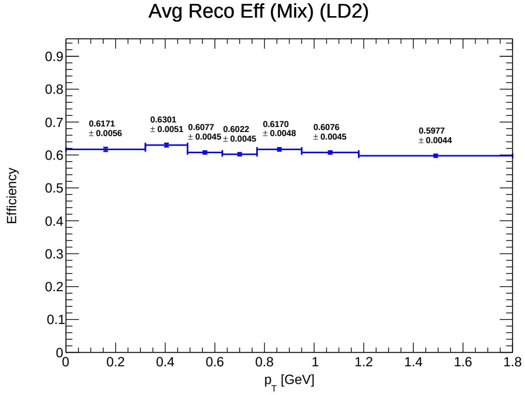
Figure 14: E_mix_reco_LD2
