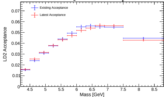
LD2 Existing vs Latest: Mass in x_F Bin 8
