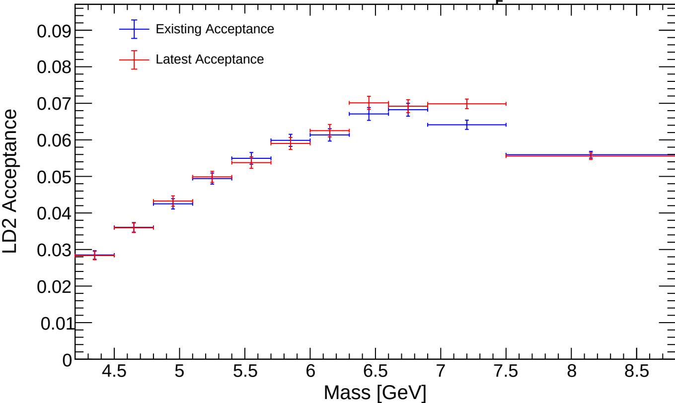
LD2 Existing vs Latest: Mass in x_E Bin 13
