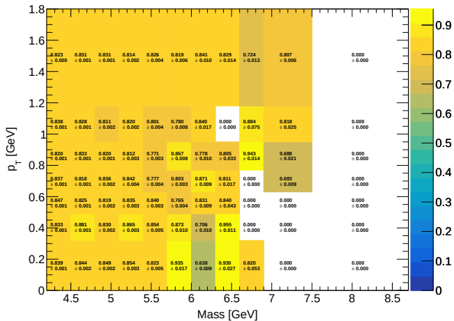
Avg Hodo Eff (Mix) (LH2)
