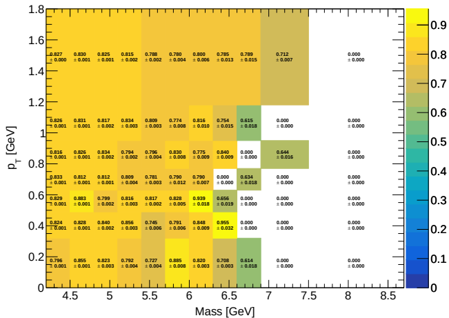
Avg Hodo Eff (Mix) (LD2)
