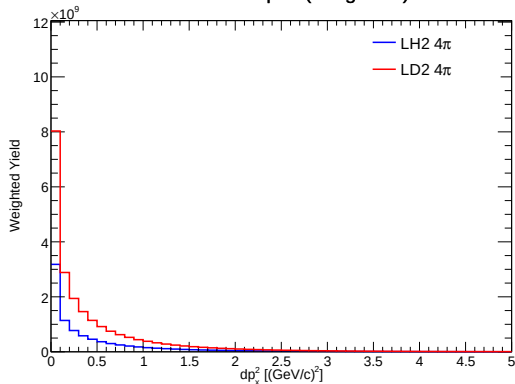
4\pi Yield of dp_x^2 (Integrated)
