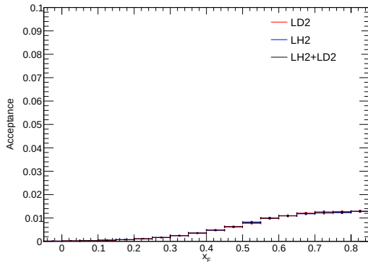
Integrated Acceptance vs x_F
