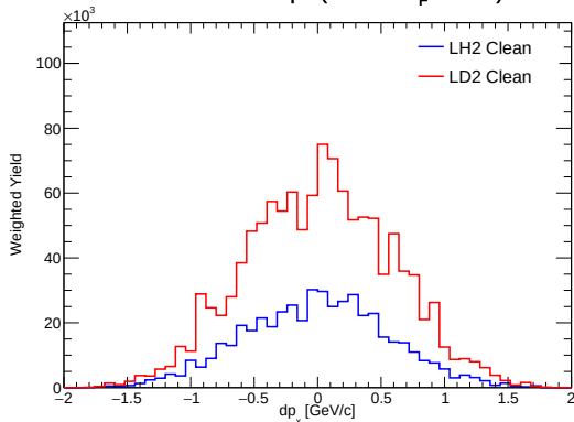
Clean Yield of dp_x ( 0.15 \leq x_F < 0.20 )
