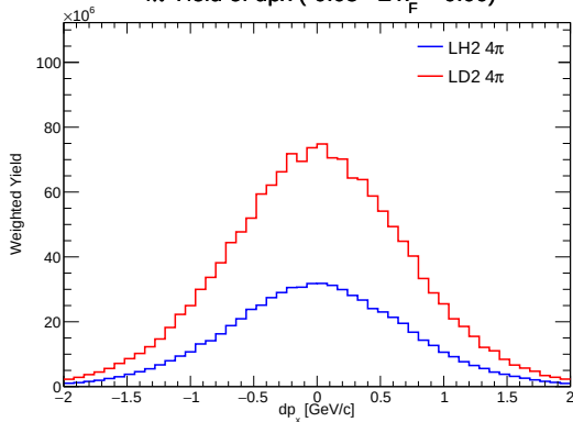
4 \pi Yield of dp_x ( -0.05 \leq x_F < 0.00 )
