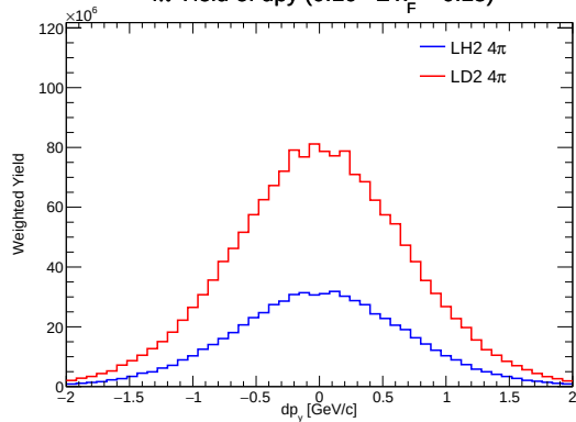
4\pi Yield of dp_y ( 0.10 \leq x_F < 0.15 )
