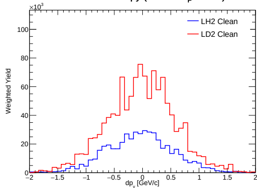
Clean Yield of dp_y ( 0.15 \leq x_F < 0.20 )
