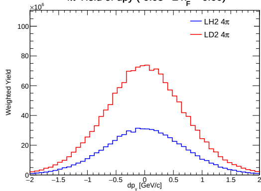
4 \pi Yield of dp_y ( -0.05 \leq x_F < 0.00 )
