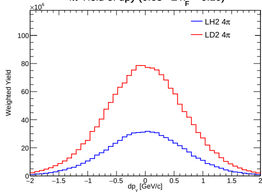
4 \pi Yield of dp_y ( 0.05 \leq x_F < 0.10 )
