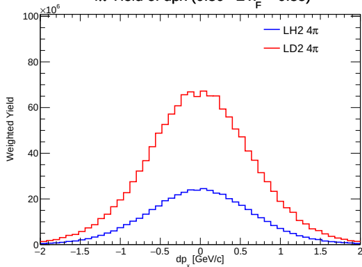
4 \pi Yield of dp x ( 0.30 \leq x_F < 0.35 )
