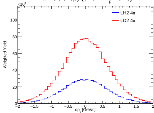
4\pi Yield of dp_y ( 0.20 \leq x_F < 0.25 )
