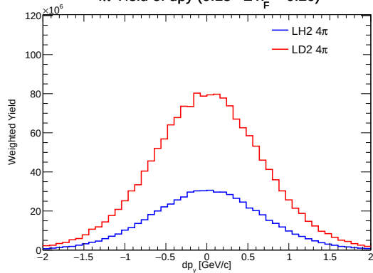
4\pi Yield of dp_y ( 0.15 \leq x_F < 0.20 )
