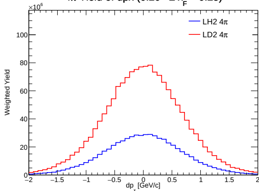
4\pi Yield of dp_x ( 0.20 \leq x_F < 0.25 )
