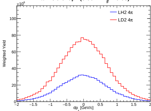
4\pi Yield of dp_x ( 0.00 \leq x_F < 0.05 )
