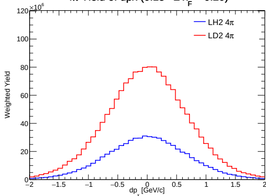
4\pi Yield of dp_x ( 0.15 \leq x_F < 0.20 )
