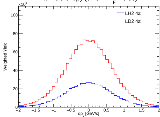
4 \pi Yield of dp y ( 0.25 \leq x_F < 0.30 )
