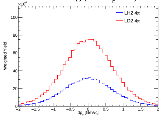
4\pi Yield of dp_y ( 0.00 \leq x_F < 0.05 )
