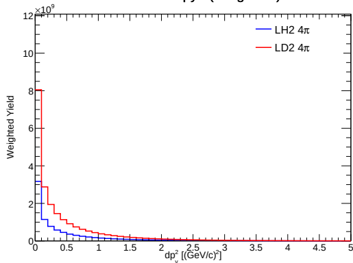
4\pi Yield of dp_y^2 (Integrated)
