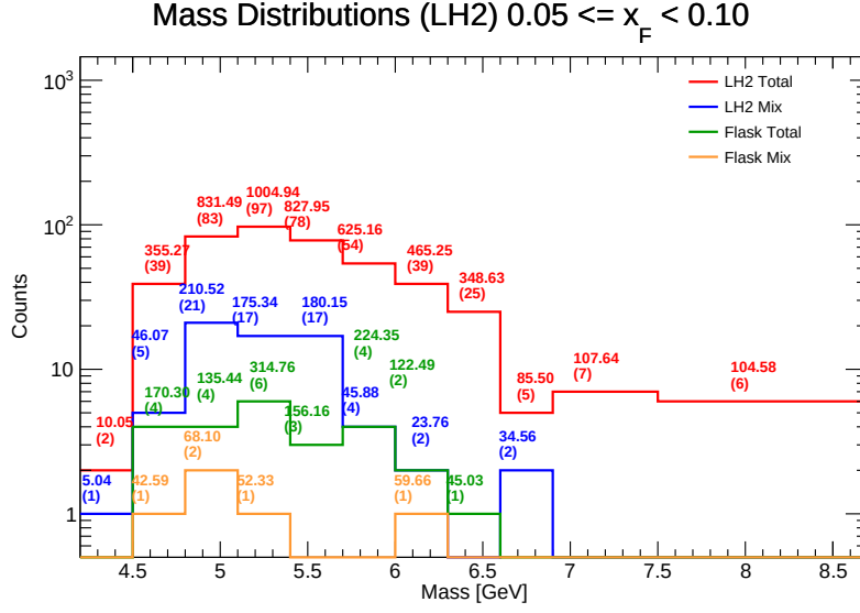
Figure 76: Invariant Mass distributions for LH 2 in the range x_F \in [0.05, 0.10] . Components shown include target total (red), target mix (blue), flask total (green), and flask mix (orange). The values listed above each bin represent the efficiency-weighted corrected mass \sum M/\epsilon and the raw counts ( N ).
