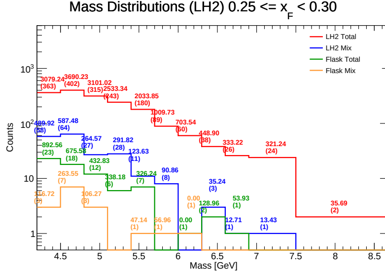
Figure 84: Invariant Mass distributions for LH 2 in the range x_F \in [0.25, 0.30) . Components shown include target total (red), target mix (blue), flask total (green), and flask mix (orange). The values listed above each bin represent the efficiency-weighted corrected mass \sum M/\epsilon and the raw counts ( N ).
