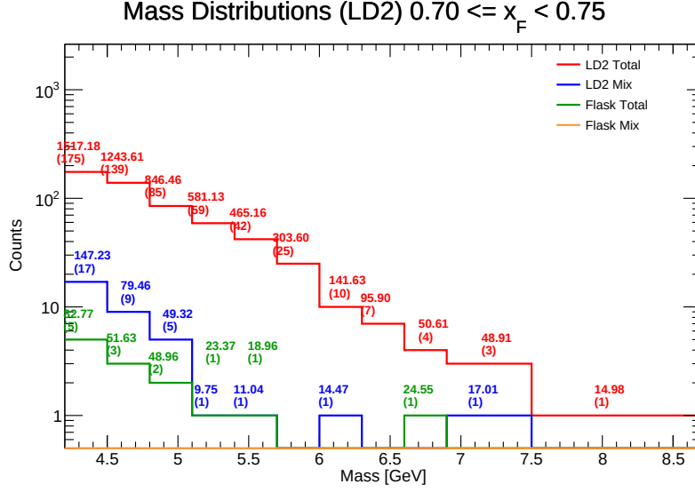
Figure 103: Invariant Mass distributions for LD 2 in the range x_F \in [0.70, 0.75] . Components shown include target total (red), target mix (blue), flask total (green), and flask mix (orange). The values listed above each bin represent the efficiency-weighted corrected mass \sum M/\epsilon and the raw counts ( N ).
