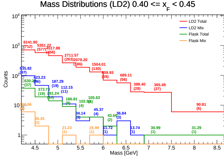
Figure 91: Invariant Mass distributions for LD 2 in the range x_F \in [0.40, 0.45] . Components shown include target total (red), target mix (blue), flask total (green), and flask mix (orange). The values listed above each bin represent the efficiency-weighted corrected mass \sum M/\epsilon and the raw counts ( N ).
