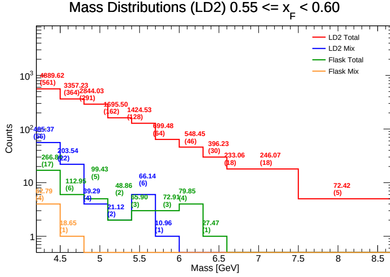
Figure 97: Invariant Mass distributions for LD 2 in the range x_F \in [0.55, 0.60] . Components shown include target total (red), target mix (blue), flask total (green), and flask mix (orange). The values listed above each bin represent the efficiency-weighted corrected mass \sum M/\epsilon and the raw counts ( N ).
