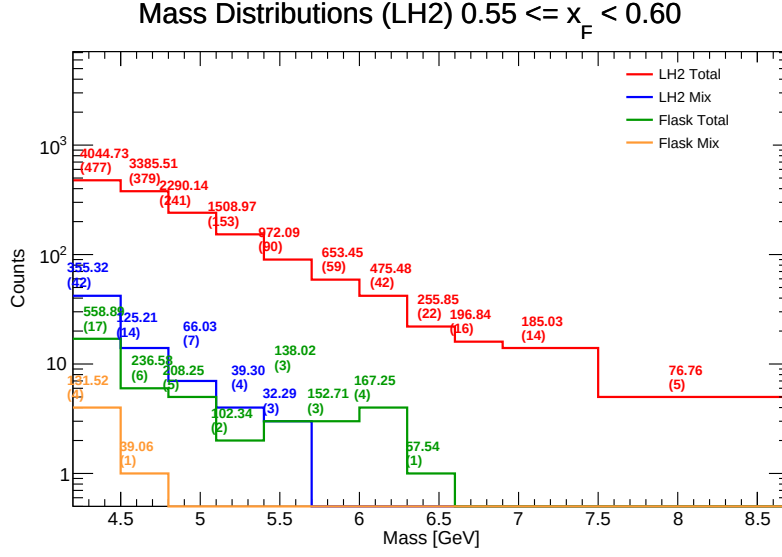
Figure 96: Invariant Mass distributions for LH 2 in the range x_F \in [0.55, 0.60] . Components shown include target total (red), target mix (blue), flask total (green), and flask mix (orange). The values listed above each bin represent the efficiency-weighted corrected mass \sum M/\epsilon and the raw counts ( N ).
