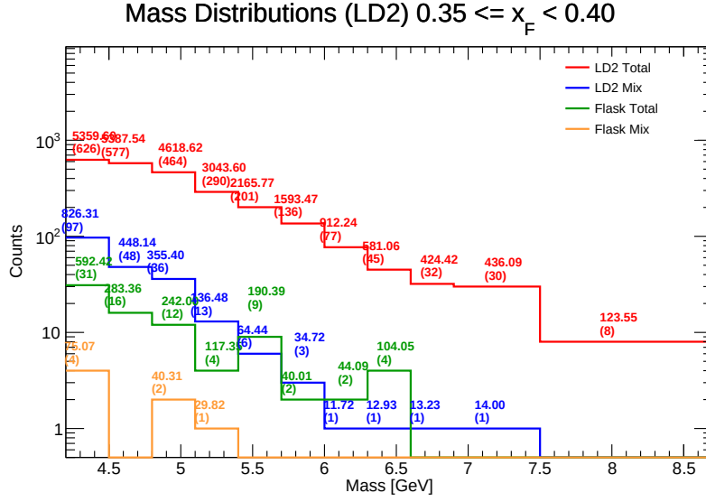
Figure 89: Invariant Mass distributions for LD 2 in the range x_F \in [0.35, 0.40) . Components shown include target total (red), target mix (blue), flask total (green), and flask mix (orange). The values listed above each bin represent the efficiency-weighted corrected mass \sum M/\epsilon and the raw counts ( N ).
