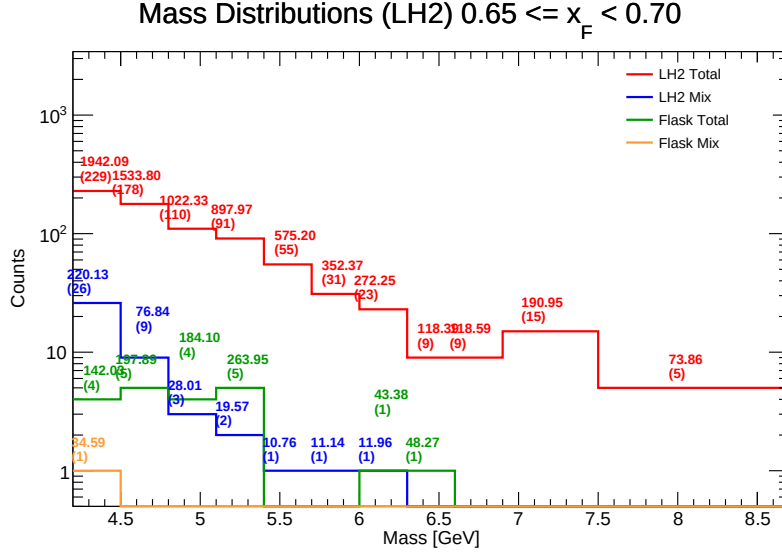
Figure 100: Invariant Mass distributions for LH 2 in the range x_F \in [0.65, 0.70) . Components shown include target total (red), target mix (blue), flask total (green), and flask mix (orange). The values listed above each bin represent the efficiency-weighted corrected mass \sum M/\epsilon and the raw counts ( N ).
