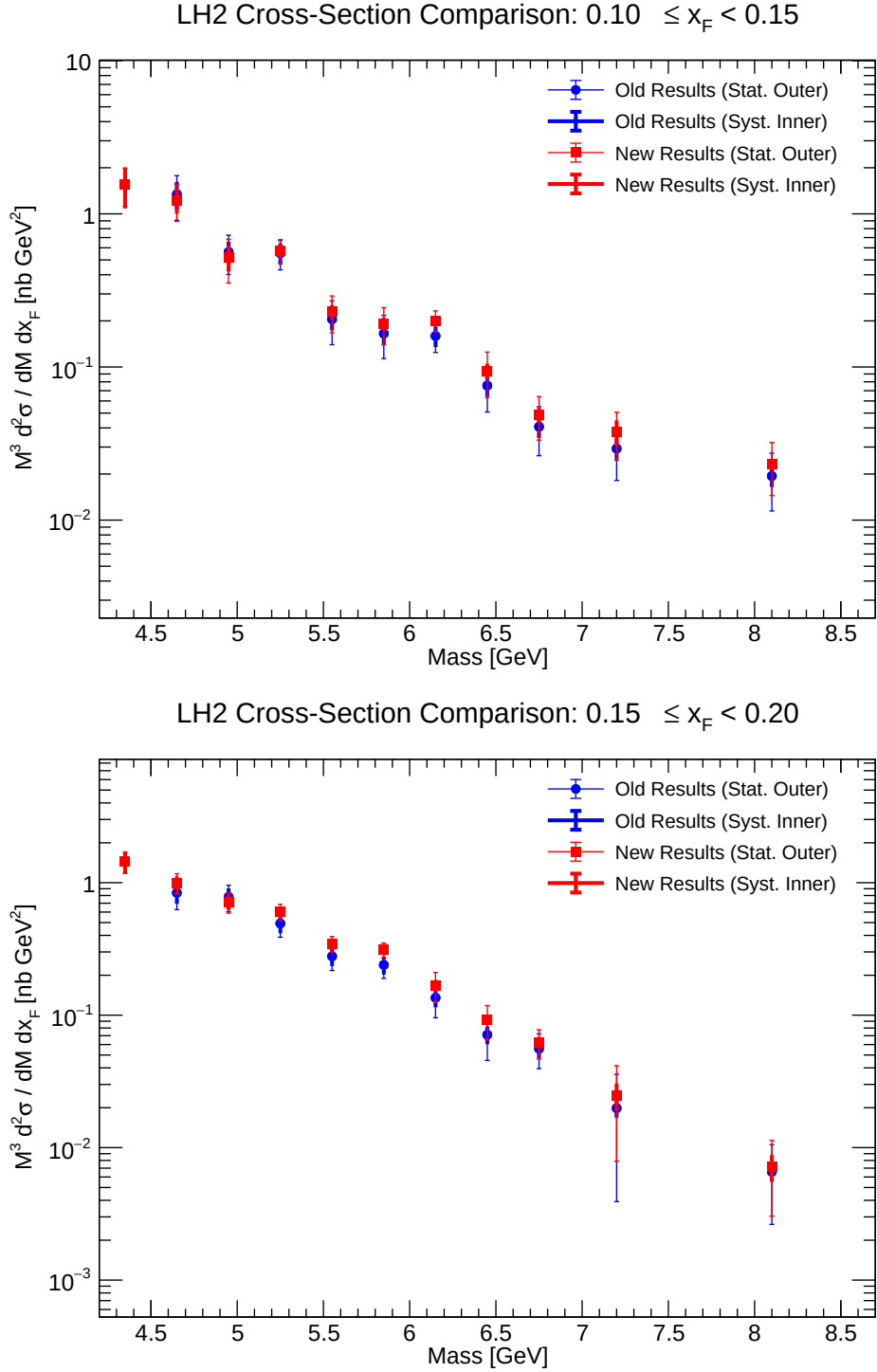
Figure 47: Comparison of double-differential cross-section for LH2 ( x_F bins 0.10-0.20).
