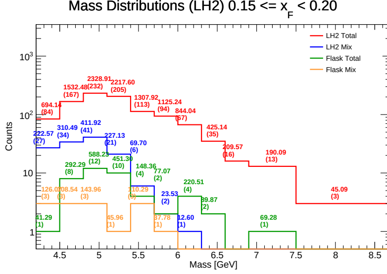
Figure 80: Invariant Mass distributions for LH 2 in the range x_F \in [0.15, 0.20) . Components shown include target total (red), target mix (blue), flask total (green), and flask mix (orange). The values listed above each bin represent the efficiency-weighted corrected mass \sum M/\epsilon and the raw counts ( N ).
