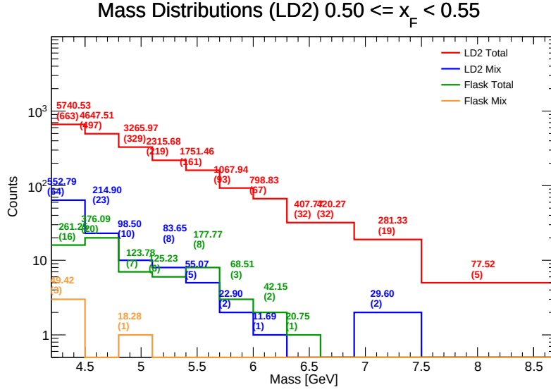
Figure 95: Invariant Mass distributions for LD 2 in the range x_F \in [0.50, 0.55] . Components shown include target total (red), target mix (blue), flask total (green), and flask mix (orange). The values listed above each bin represent the efficiency-weighted corrected mass \sum M/\epsilon and the raw counts ( N ).
