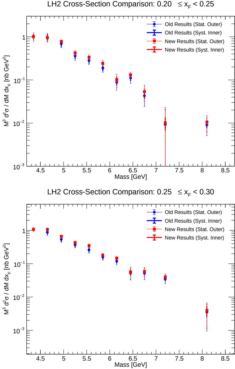
Figure 48: Comparison of double-differential cross-section for LH2 ( x_F bins 0.20-0.30).
