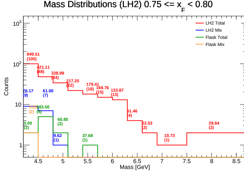
Figure 104: Invariant Mass distributions for LH 2 in the range x_F \in [0.75, 0.80) . Components shown include target total (red), target mix (blue), flask total (green), and flask mix (orange). The values listed above each bin represent the efficiency-weighted corrected mass \sum M/\epsilon and the raw counts ( N ).
