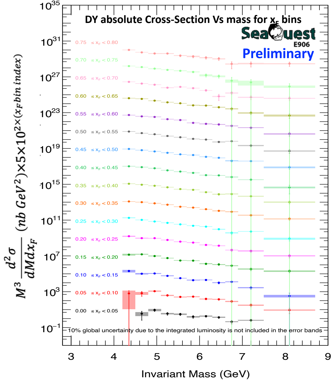
Figure 45: Cross-section summary plots for both LD2 target.
