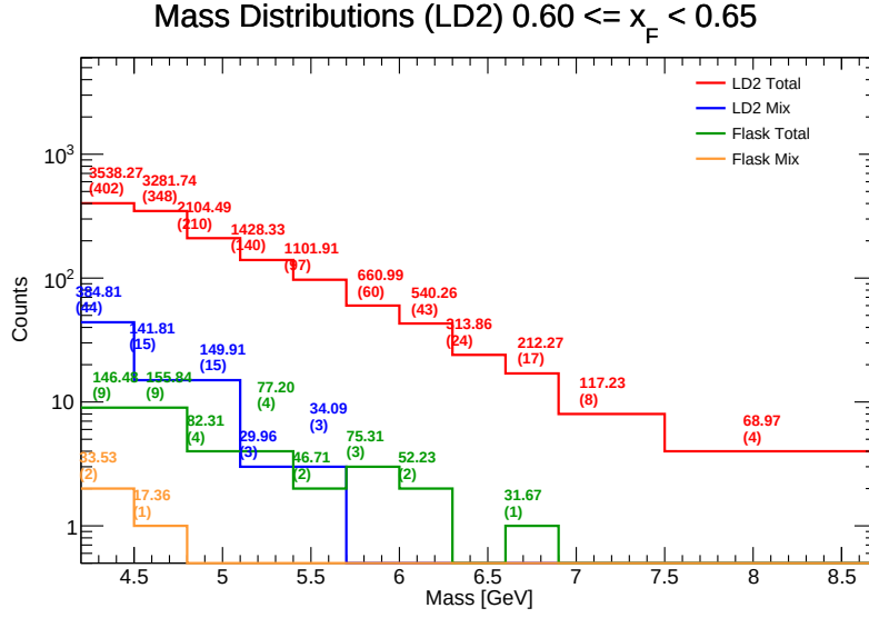
Figure 99: Invariant Mass distributions for LD 2 in the range x_F \in [0.60, 0.65) . Components shown include target total (red), target mix (blue), flask total (green), and flask mix (orange). The values listed above each bin represent the efficiency-weighted corrected mass \sum M/\epsilon and the raw counts ( N ).
