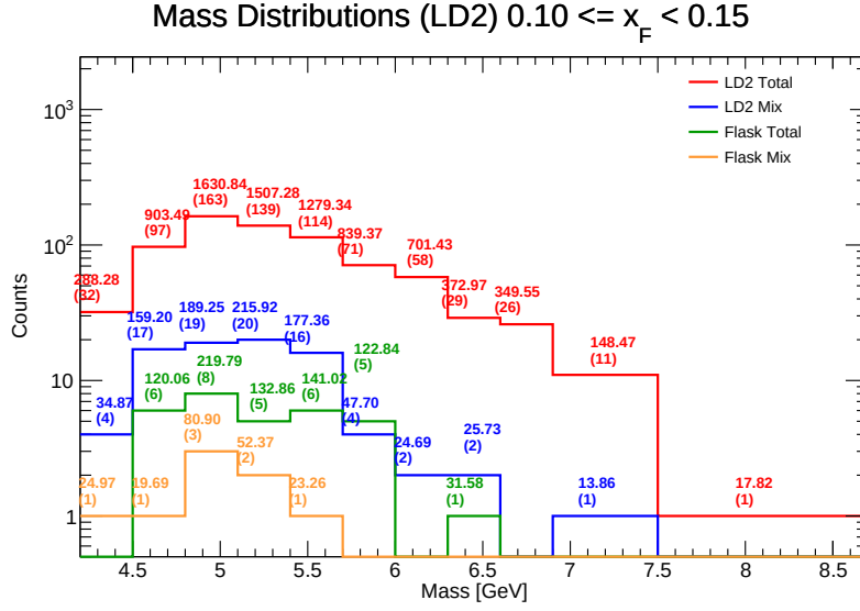
Figure 79: Invariant Mass distributions for LD 2 in the range x_F \in [0.10, 0.15] . Components shown include target total (red), target mix (blue), flask total (green), and flask mix (orange). The values listed above each bin represent the efficiency-weighted corrected mass \sum M/\epsilon and the raw counts ( N ).
