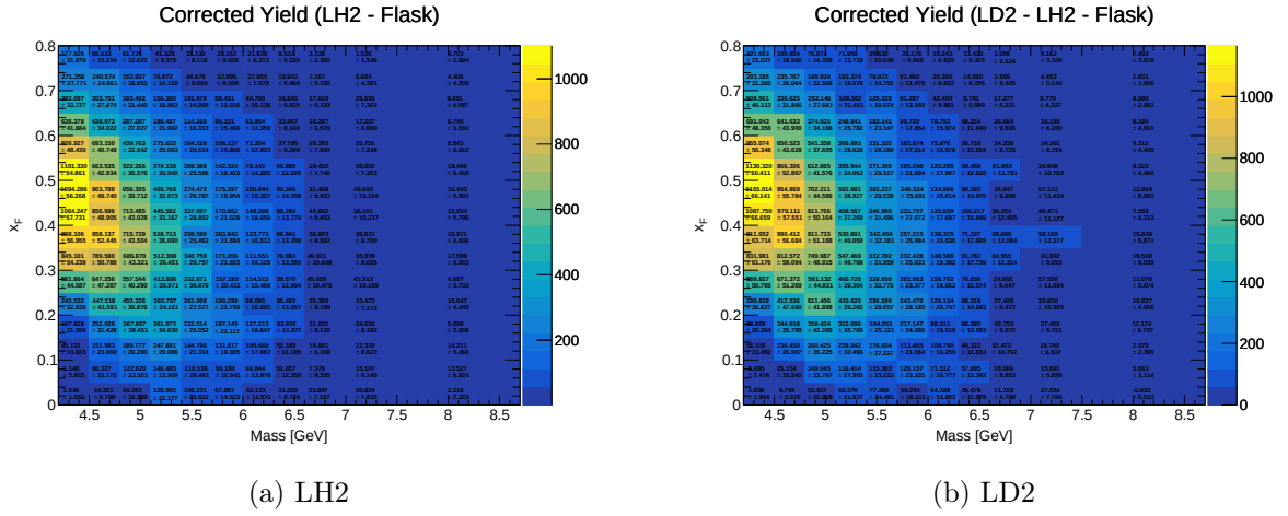
Figure 11: Corrected yields for LH2 (a) and LD2 (b) after correcting for efficiencies, with propagated uncertainties.
