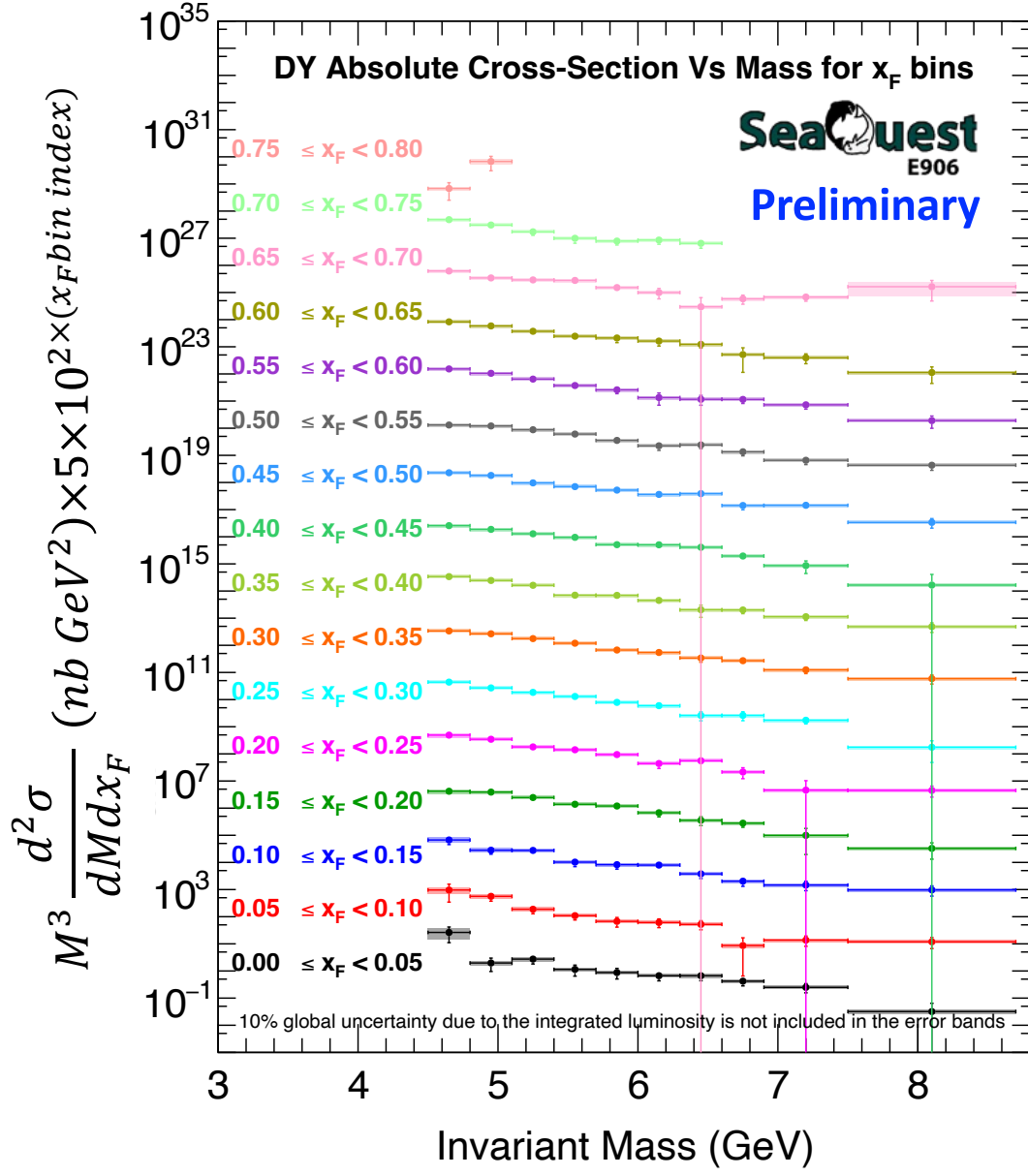
Figure 44: Cross-section summary plots for both LH2 target.
