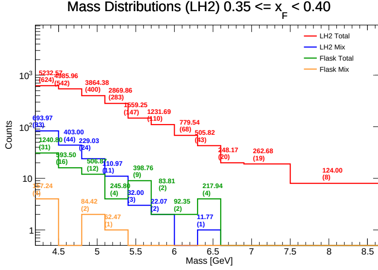
Figure 88: Invariant Mass distributions for LH 2 in the range x_F \in [0.35, 0.40] . Components shown include target total (red), target mix (blue), flask total (green), and flask mix (orange). The values listed above each bin represent the efficiency-weighted corrected mass \sum M/\epsilon and the raw counts ( N ).
