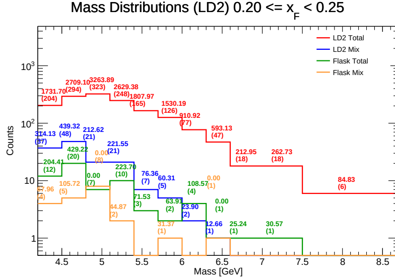
Figure 83: Invariant Mass distributions for LD 2 in the range x_F \in [0.20, 0.25] . Components shown include target total (red), target mix (blue), flask total (green), and flask mix (orange). The values listed above each bin represent the efficiency-weighted corrected mass \sum M/\epsilon and the raw counts ( N ).
