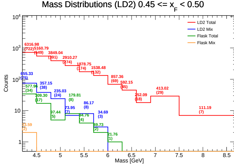
Figure 93: Invariant Mass distributions for LD 2 in the range x_F \in [0.45, 0.50] . Components shown include target total (red), target mix (blue), flask total (green), and flask mix (orange). The values listed above each bin represent the efficiency-weighted corrected mass \sum M/\epsilon and the raw counts ( N ).
