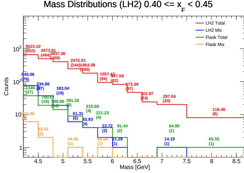
Figure 90: Invariant Mass distributions for LH 2 in the range x_F \in [0.40, 0.45] . Components shown include target total (red), target mix (blue), flask total (green), and flask mix (orange). The values listed above each bin represent the efficiency-weighted corrected mass \sum M/\epsilon and the raw counts ( N ).
