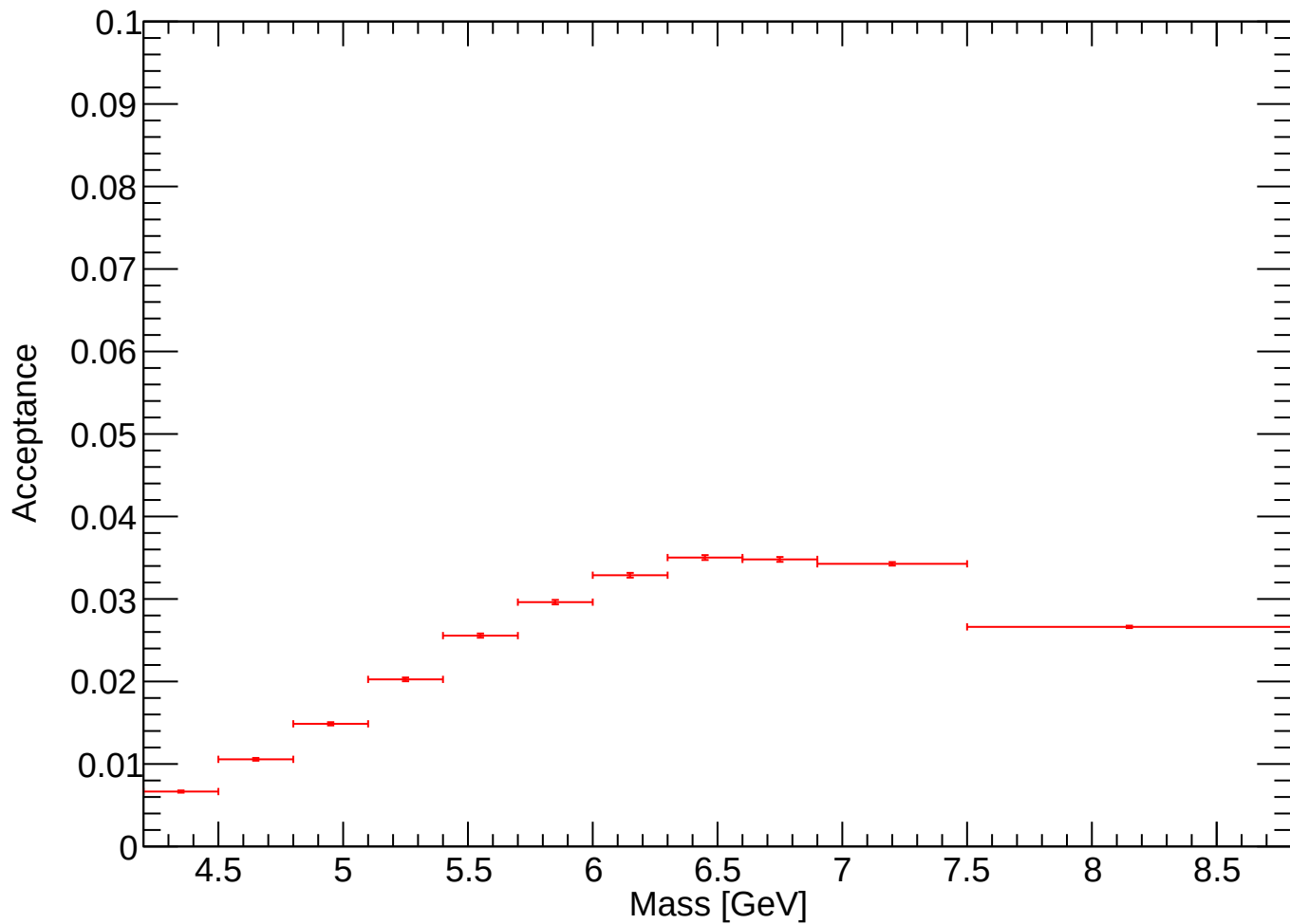
Integrated Acceptance vs mass
