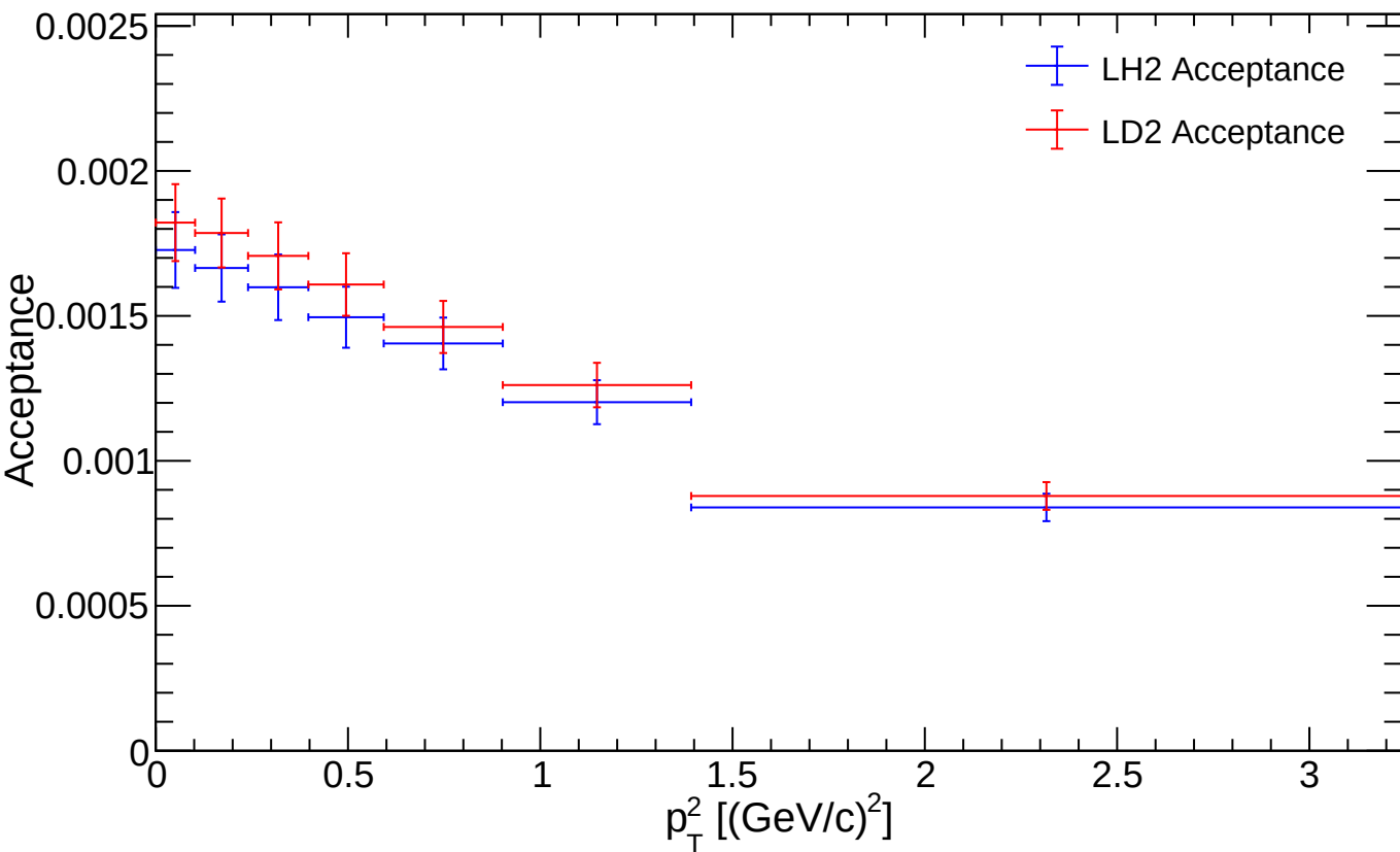
p_T^2 Acceptance (All Mass, x_F )
