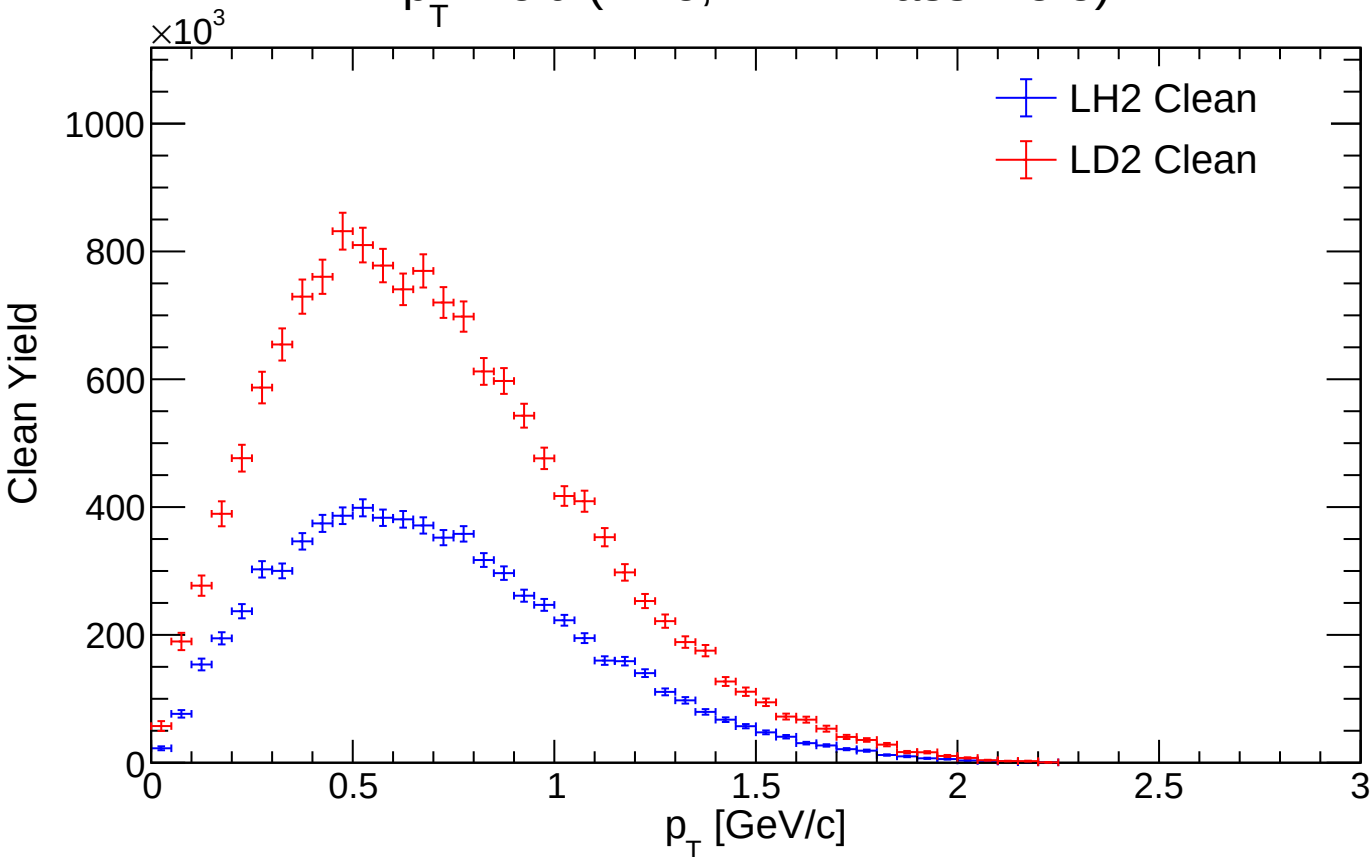
p_T Yield (Fine, 4.2 < \text{Mass} < 5.5 )
