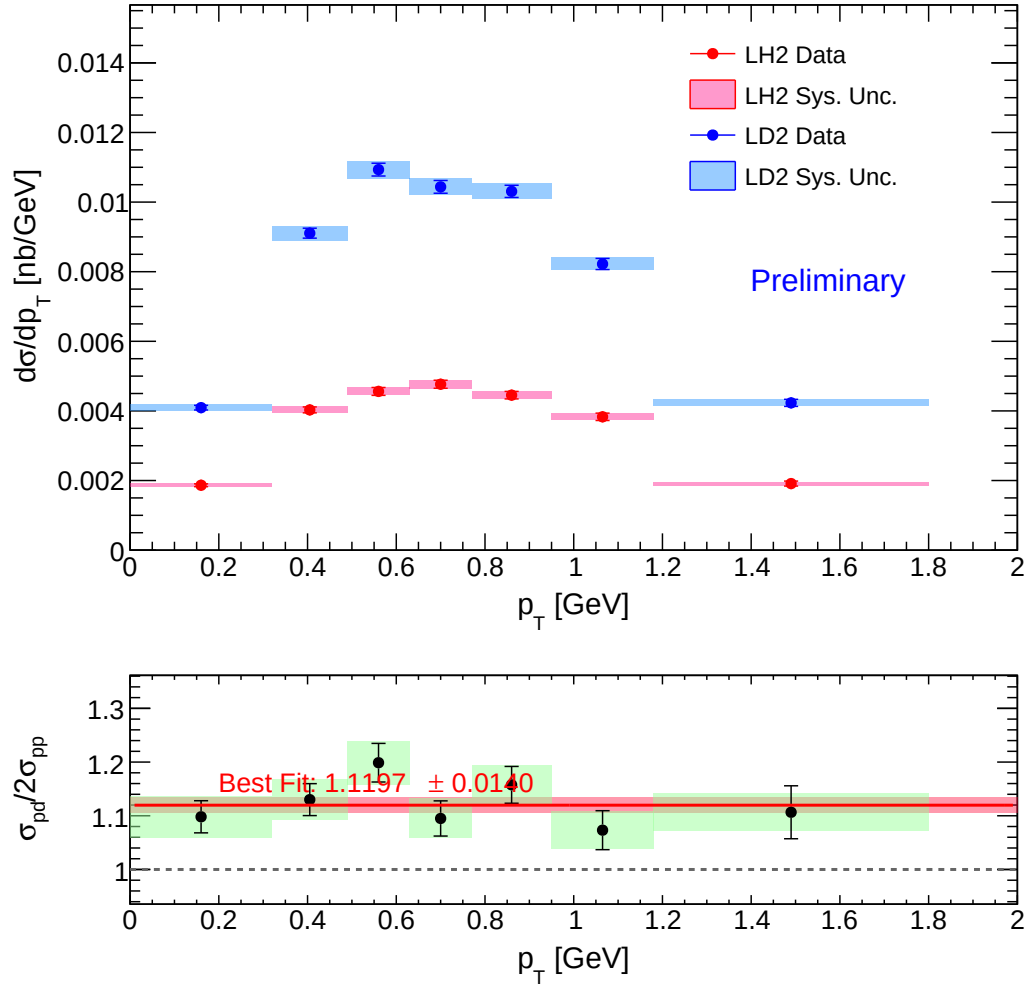
Figure 39: Combined_XSec_Ratio_vs_pT_geom
