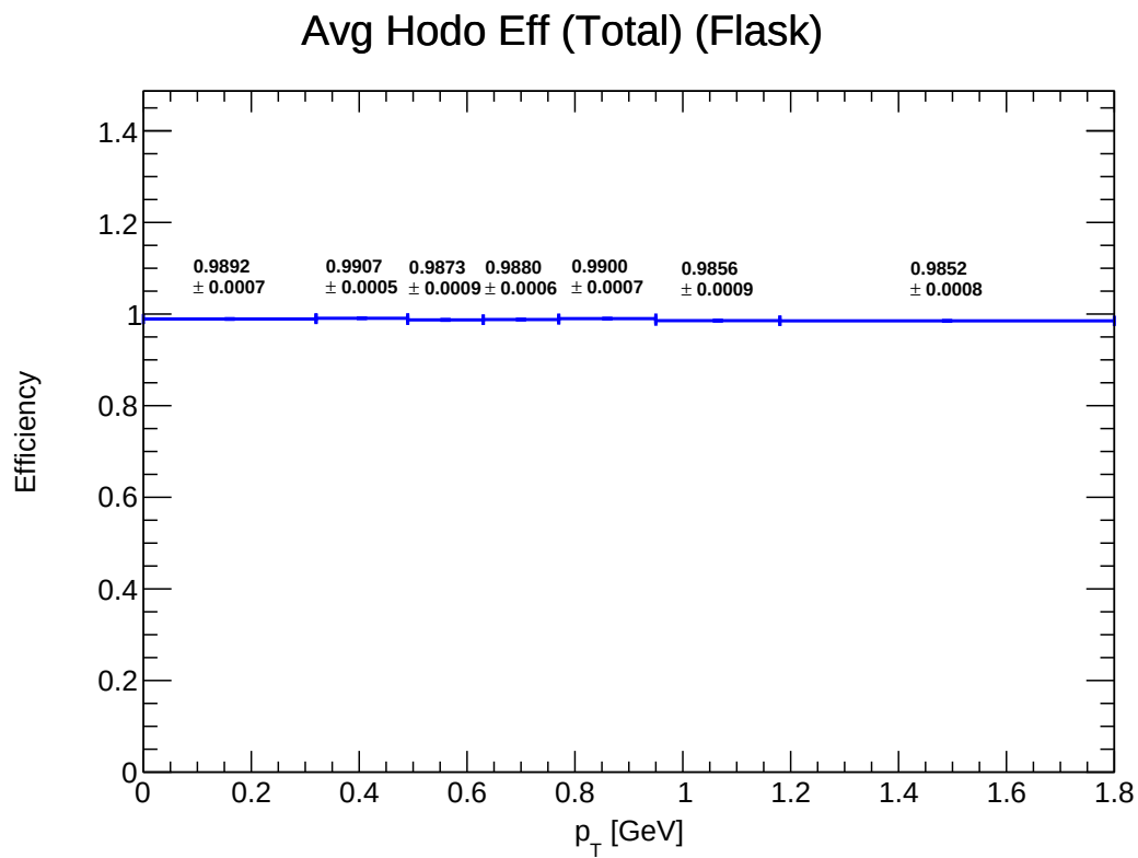
Figure 15: E_total_hodo_Flask
