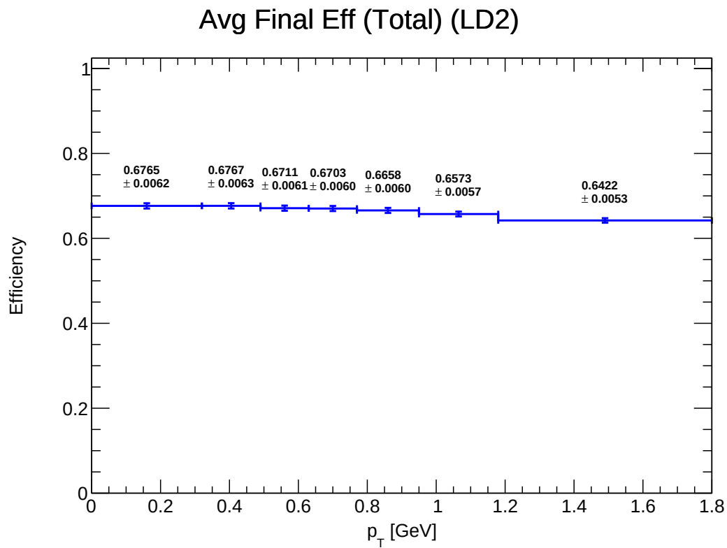
Figure 20: E_total_final_LD2
