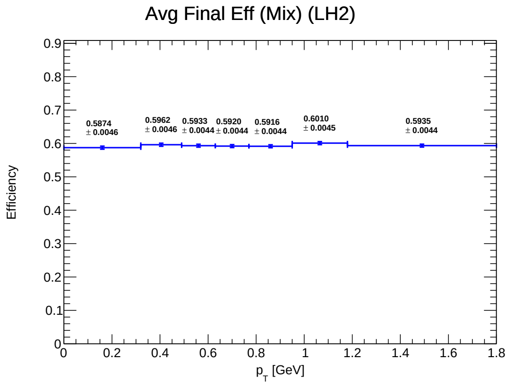
Figure 22: E_mix_final_LH2
