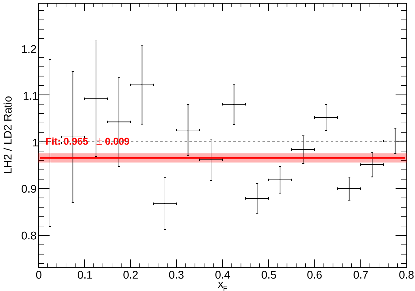
LH2/LD2 Integrated Acceptance vs x_F
