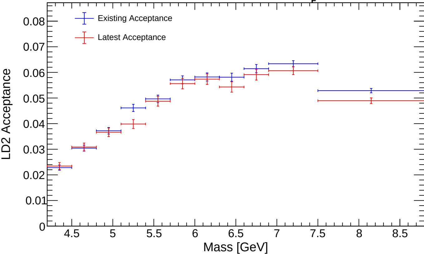
LD2 Existing vs Latest: Mass in x_E Bin 10
