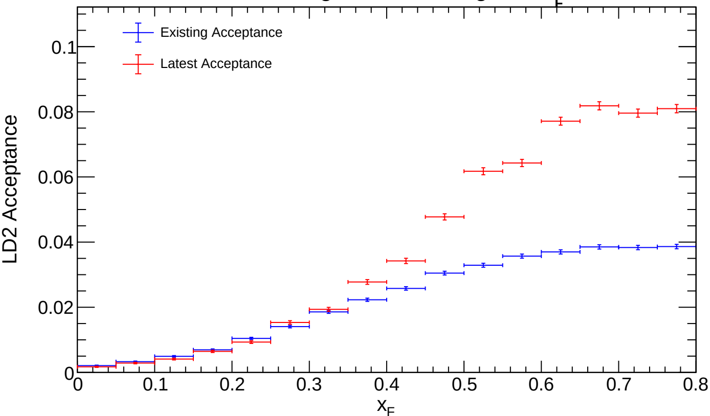
LD2 Existing vs Latest: Integrated x_F
