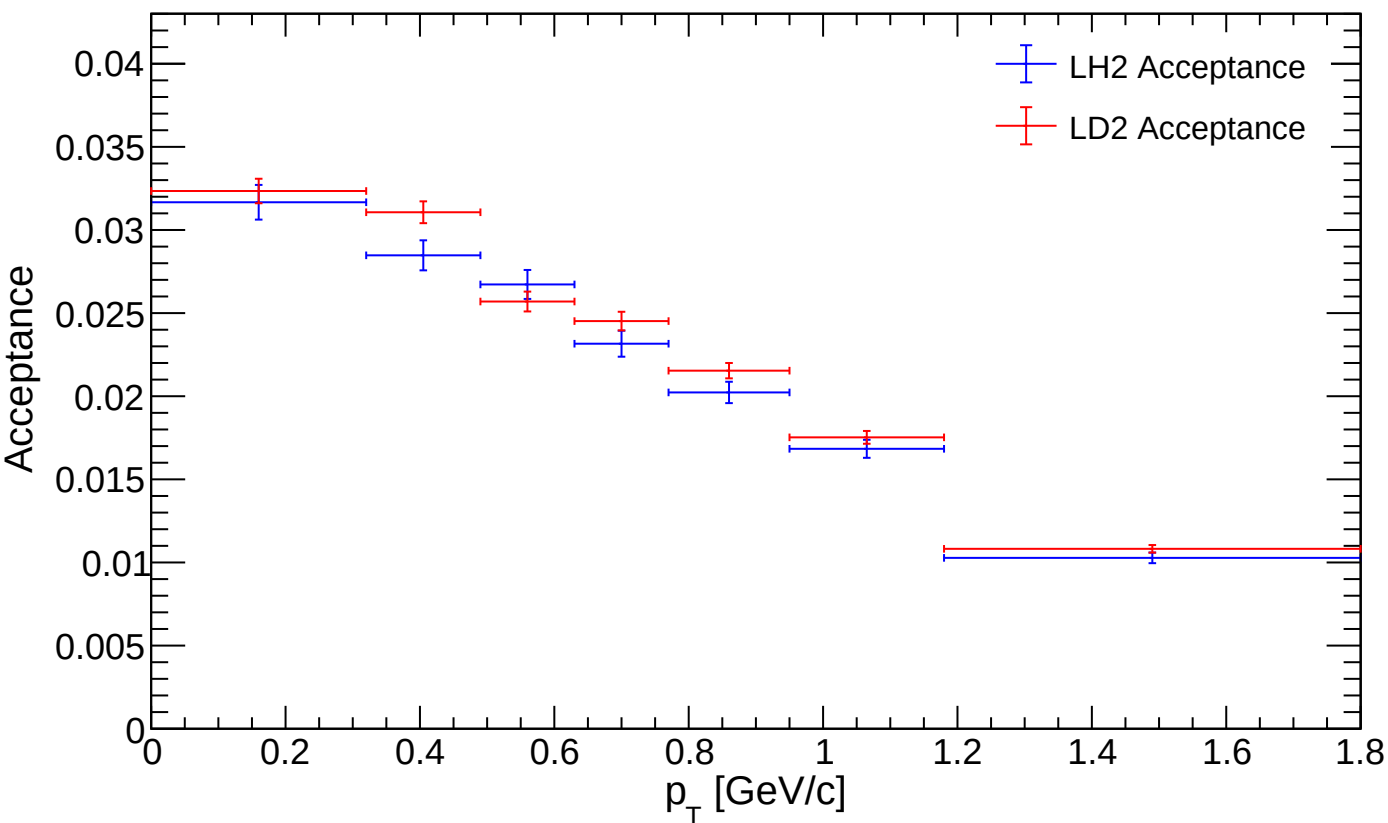
p_T Acceptance (All Mass, x_F )
