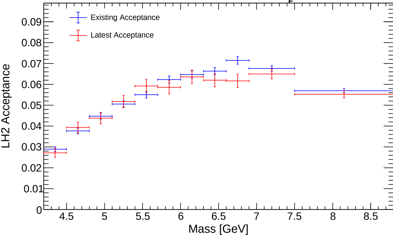
LH2 Existing vs Latest: Mass in x_E Bin 14
