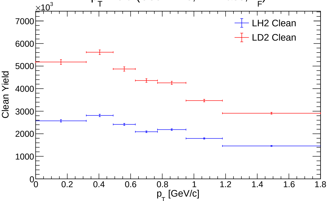
p_T Yield (User Bins, All Mass, x_F )
