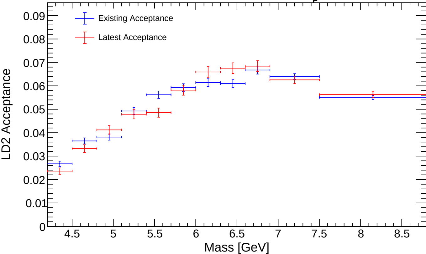
LD2 Existing vs Latest: Mass in x_E Bin 12
