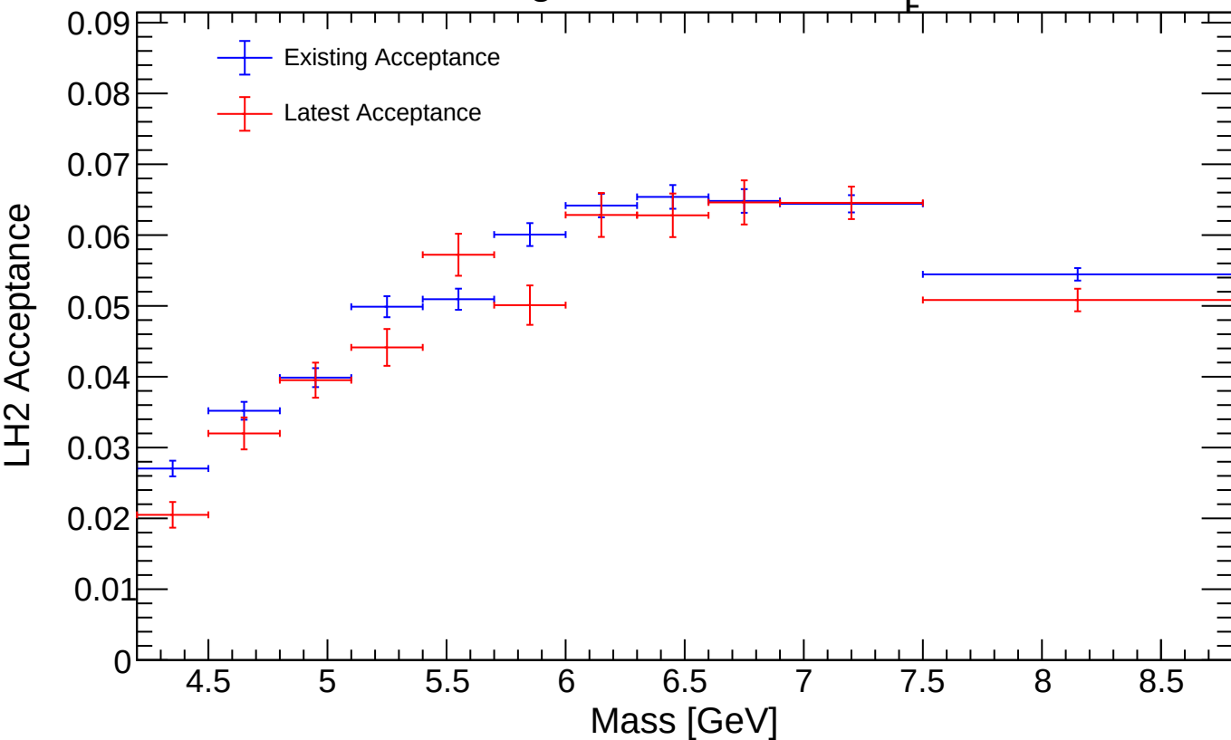
LH2 Existing vs Latest: Mass in x_E Bin 11
