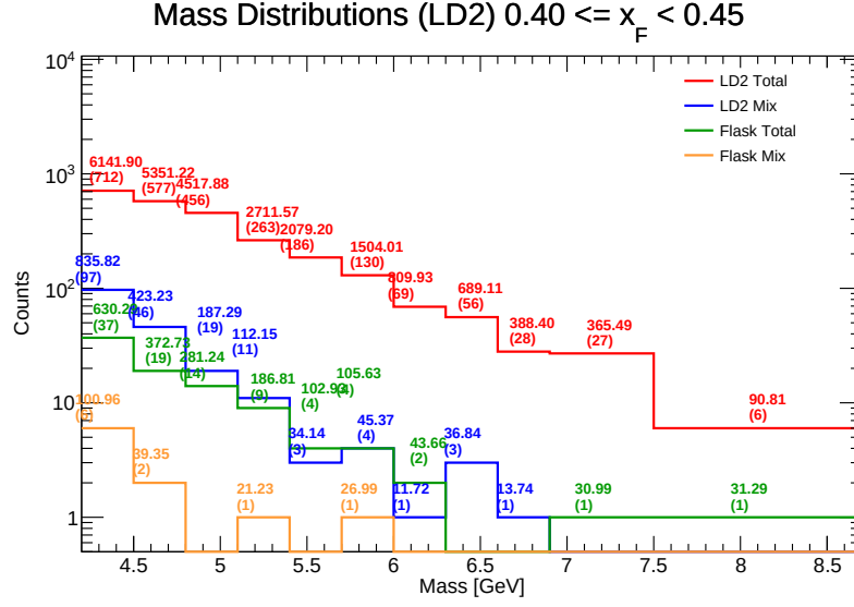
Figure 89: Invariant Mass distributions for LD 2 in the range x_F \in [0.40, 0.45) . Components shown include target total (red), target mix (blue), flask total (green), and flask mix (orange). The values listed above each bin represent the efficiency-weighted corrected mass \sum M/\epsilon and the raw counts ( N ).
