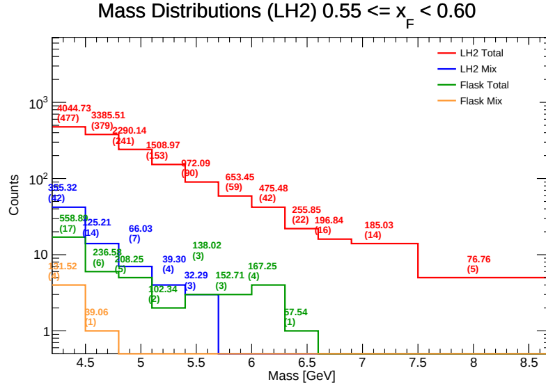
Figure 94: Invariant Mass distributions for LH 2 in the range x_F \in [0.55, 0.60] . Components shown include target total (red), target mix (blue), flask total (green), and flask mix (orange). The values listed above each bin represent the efficiency-weighted corrected mass \sum M/\epsilon and the raw counts ( N ).
