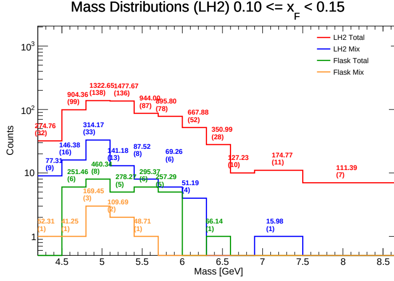
Figure 76: Invariant Mass distributions for LH 2 in the range x_F \in [0.10, 0.15) . Components shown include target total (red), target mix (blue), flask total (green), and flask mix (orange). The values listed above each bin represent the efficiency-weighted corrected mass \sum M/\epsilon and the raw counts ( N ).
