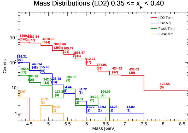
Figure 87: Invariant Mass distributions for LD 2 in the range x_F \in [0.35, 0.40) . Components shown include target total (red), target mix (blue), flask total (green), and flask mix (orange). The values listed above each bin represent the efficiency-weighted corrected mass \sum M/\epsilon and the raw counts ( N ).
