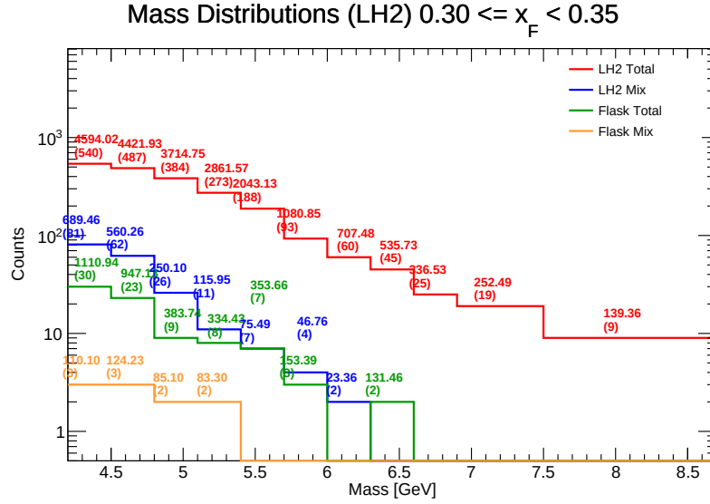
Figure 84: Invariant Mass distributions for LH 2 in the range x_F \in [0.30, 0.35] . Components shown include target total (red), target mix (blue), flask total (green), and flask mix (orange). The values listed above each bin represent the efficiency-weighted corrected mass \sum M/\epsilon and the raw counts ( N ).
