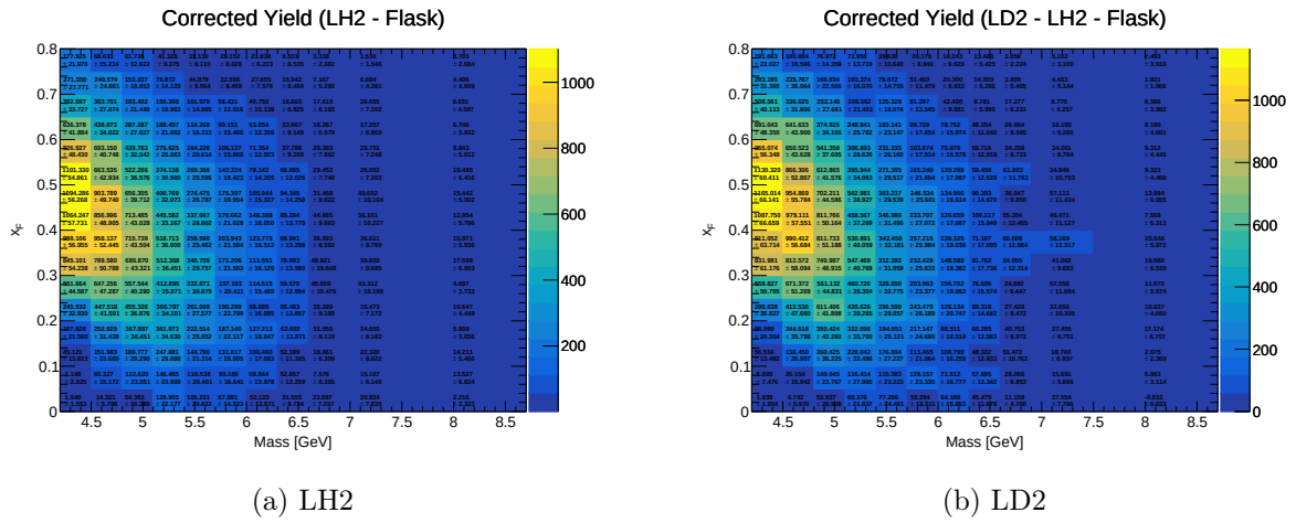
Figure 9: Corrected yields for LH2 (a) and LD2 (b) after correcting for efficiencies, with propagated uncertainties.
