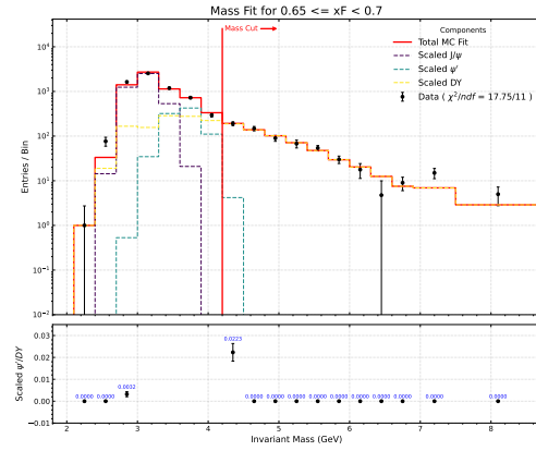
(b) 0.65 \leq x_F < 0.7
