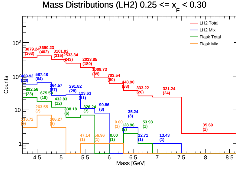
Figure 82: Invariant Mass distributions for LH 2 in the range x_F \in [0.25, 0.30) . Components shown include target total (red), target mix (blue), flask total (green), and flask mix (orange). The values listed above each bin represent the efficiency-weighted corrected mass \sum M/\epsilon and the raw counts ( N ).
