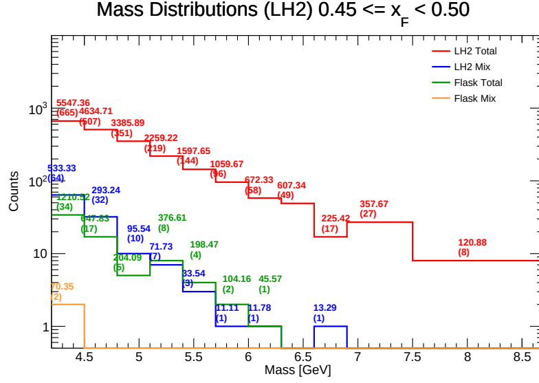
Figure 90: Invariant Mass distributions for LH 2 in the range x_F \in [0.45, 0.50) . Components shown include target total (red), target mix (blue), flask total (green), and flask mix (orange). The values listed above each bin represent the efficiency-weighted corrected mass \sum M/\epsilon and the raw counts ( N ).
