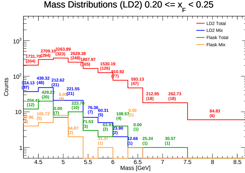
Figure 81: Invariant Mass distributions for LD 2 in the range x_F \in [0.20, 0.25) . Components shown include target total (red), target mix (blue), flask total (green), and flask mix (orange). The values listed above each bin represent the efficiency-weighted corrected mass \sum M/\epsilon and the raw counts ( N ).
