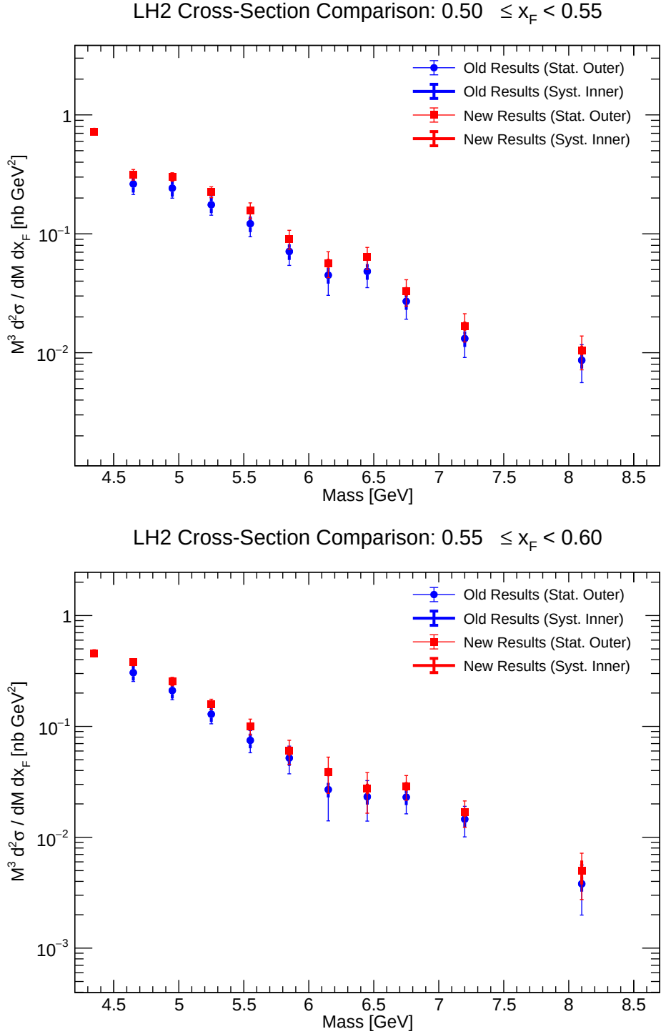
Figure 49: Comparison of double-differential cross-section for LH2 ( x_F bins 0.50-0.60).
