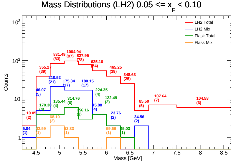
Figure 74: Invariant Mass distributions for LH 2 in the range x_F \in [0.05, 0.10) . Components shown include target total (red), target mix (blue), flask total (green), and flask mix (orange). The values listed above each bin represent the efficiency-weighted corrected mass \sum M/\epsilon and the raw counts ( N ).
