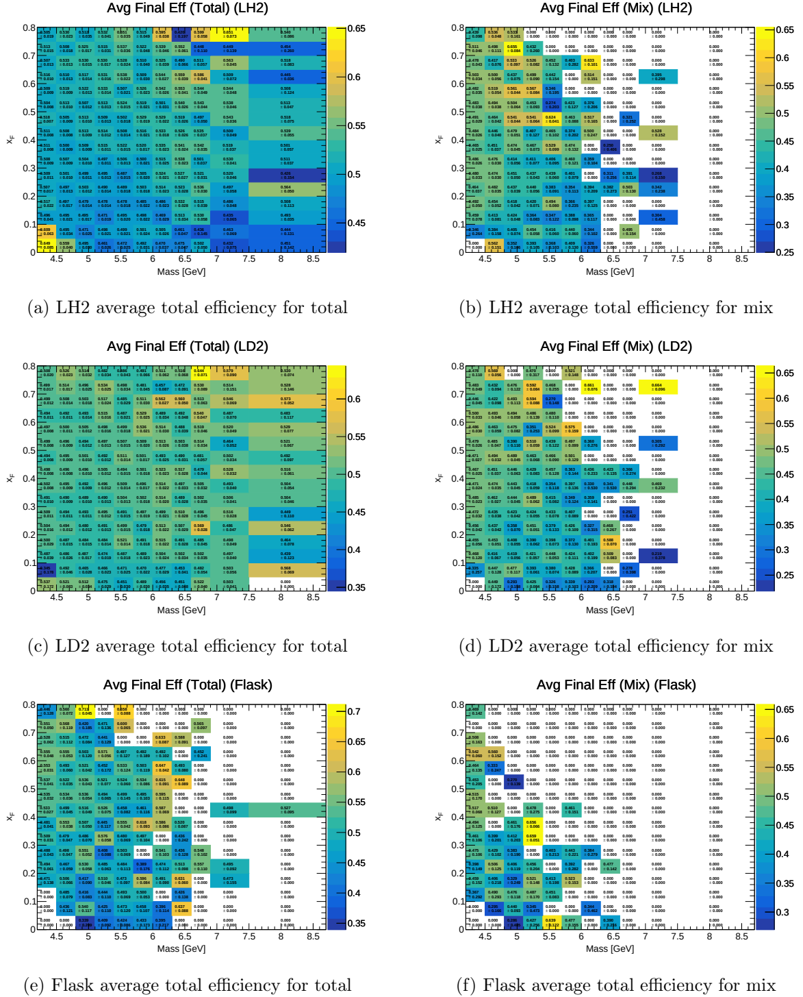
Figure 7: Average total Efficiencies calculated each kinematic bin with the propagated uncertainties.
