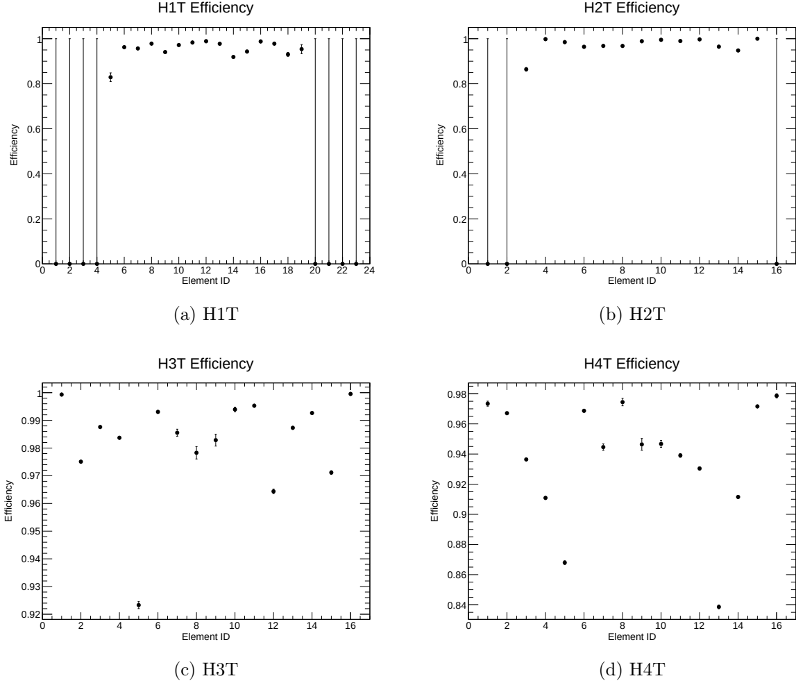
Figure 4: Hodoscope Paddle Efficiencies (Top Planes).
