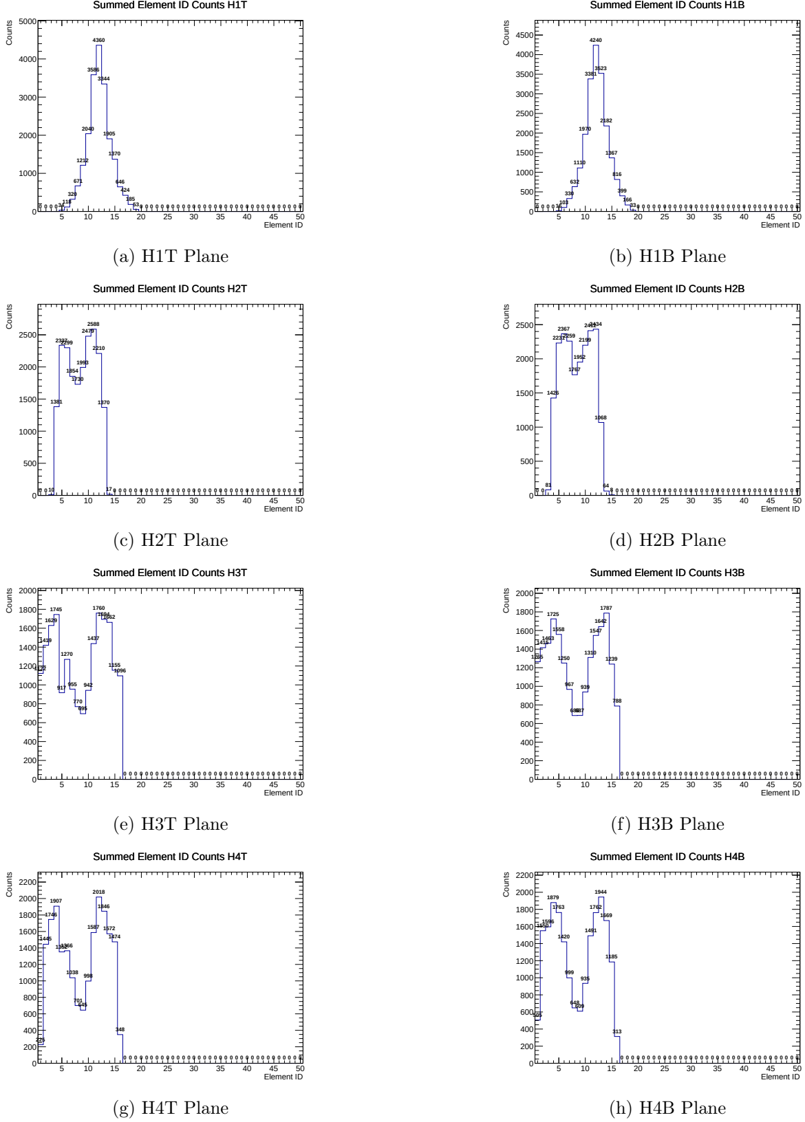
Figure 5: Hodoscope Paddle hit distributions arranged by Plane (Rows 1-4), Top vs Bottom.
