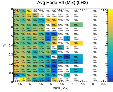
(b) LH2 average hodoscope efficiency for mix
