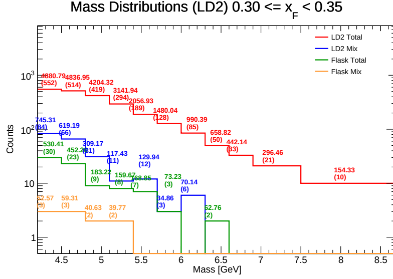
Figure 85: Invariant Mass distributions for LD 2 in the range x_F \in [0.30, 0.35) . Components shown include target total (red), target mix (blue), flask total (green), and flask mix (orange). The values listed above each bin represent the efficiency-weighted corrected mass \sum M/\epsilon and the raw counts ( N ).
