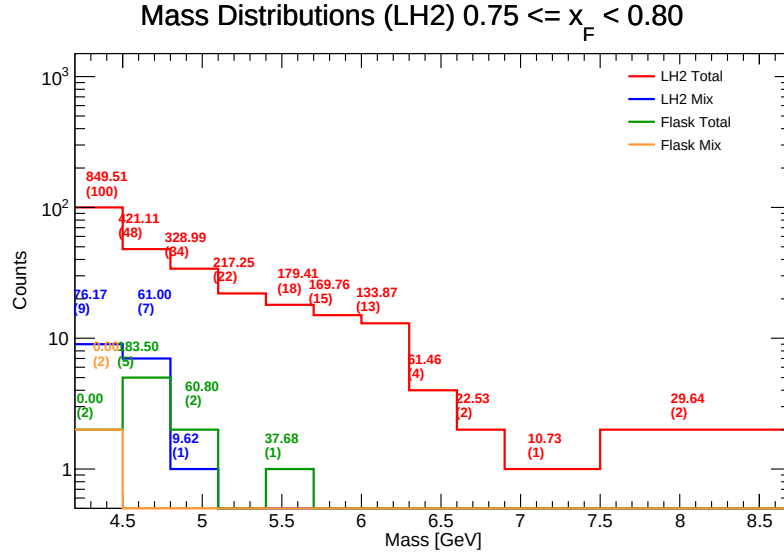
Figure 102: Invariant Mass distributions for LH 2 in the range x_F \in [0.75, 0.80) . Components shown include target total (red), target mix (blue), flask total (green), and flask mix (orange). The values listed above each bin represent the efficiency-weighted corrected mass \sum M/\epsilon and the raw counts ( N ).
