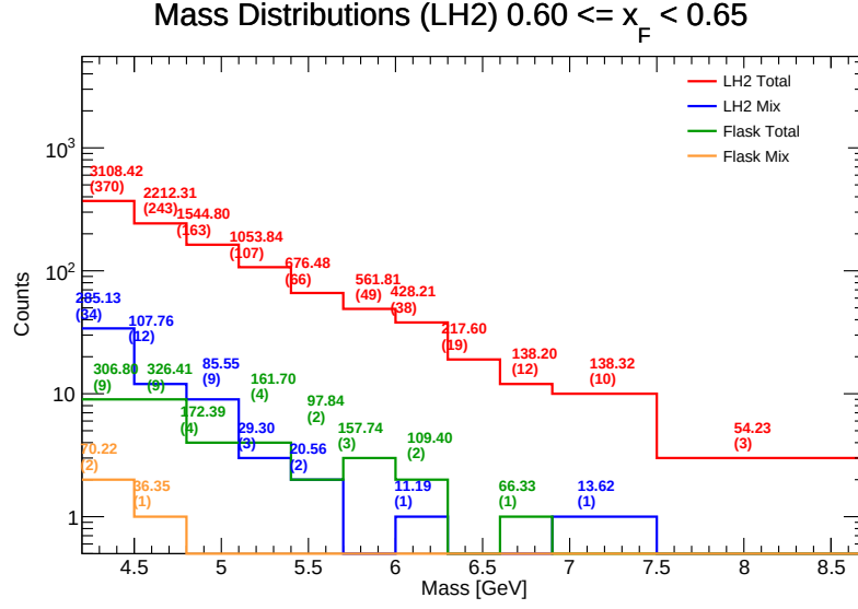
Figure 96: Invariant Mass distributions for LH 2 in the range x_F \in [0.60, 0.65] . Components shown include target total (red), target mix (blue), flask total (green), and flask mix (orange). The values listed above each bin represent the efficiency-weighted corrected mass \sum M/\epsilon and the raw counts ( N ).
