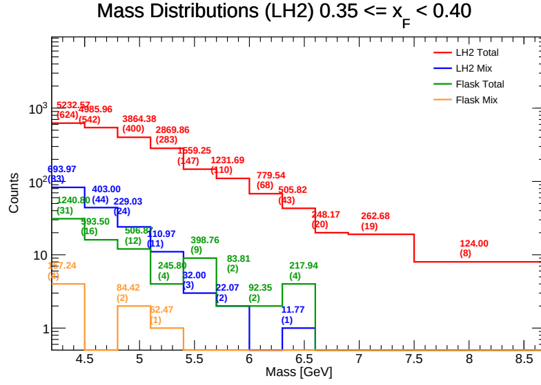
Figure 86: Invariant Mass distributions for LH 2 in the range x_F \in [0.35, 0.40) . Components shown include target total (red), target mix (blue), flask total (green), and flask mix (orange). The values listed above each bin represent the efficiency-weighted corrected mass \sum M/\epsilon and the raw counts ( N ).
