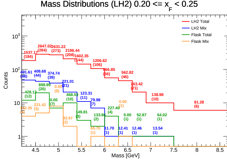
Figure 80: Invariant Mass distributions for LH 2 in the range x_F \in [0.20, 0.25] . Components shown include target total (red), target mix (blue), flask total (green), and flask mix (orange). The values listed above each bin represent the efficiency-weighted corrected mass \sum M/\epsilon and the raw counts ( N ).
