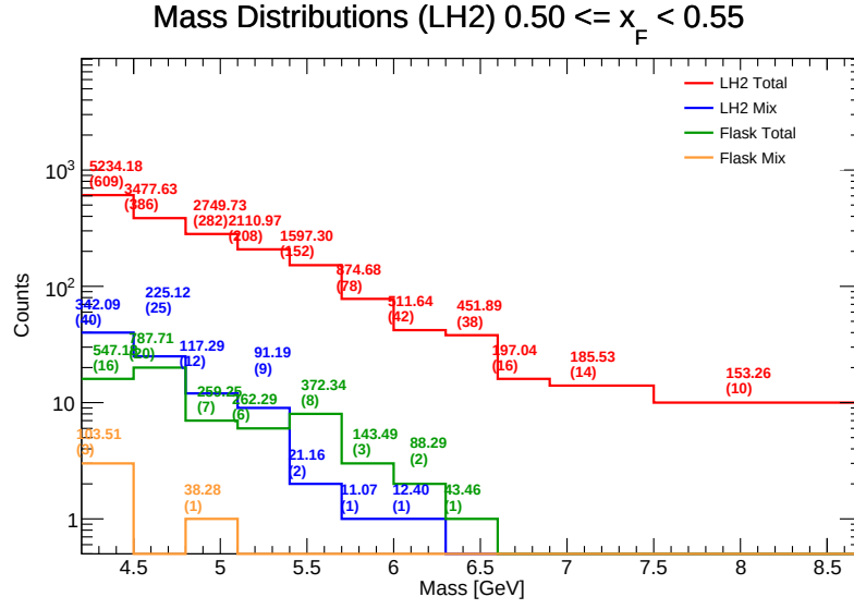
Figure 92: Invariant Mass distributions for LH 2 in the range x_F \in [0.50, 0.55] . Components shown include target total (red), target mix (blue), flask total (green), and flask mix (orange). The values listed above each bin represent the efficiency-weighted corrected mass \sum M/\epsilon and the raw counts ( N ).
