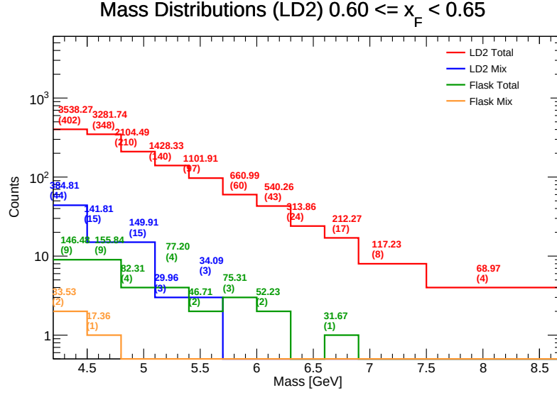
Figure 97: Invariant Mass distributions for LD 2 in the range x_F \in [0.60, 0.65) . Components shown include target total (red), target mix (blue), flask total (green), and flask mix (orange). The values listed above each bin represent the efficiency-weighted corrected mass \sum M/\epsilon and the raw counts ( N ).
