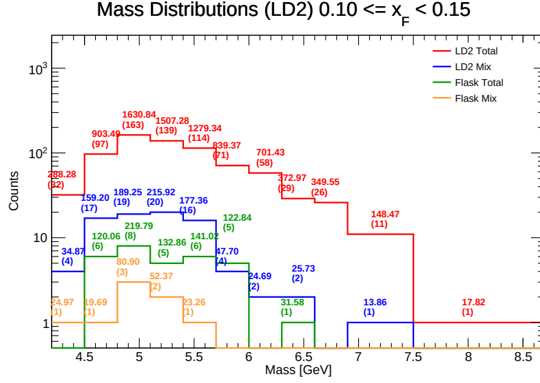
Figure 77: Invariant Mass distributions for LD 2 in the range x_F \in [0.10, 0.15) . Components shown include target total (red), target mix (blue), flask total (green), and flask mix (orange). The values listed above each bin represent the efficiency-weighted corrected mass \sum M/\epsilon and the raw counts ( N ).
