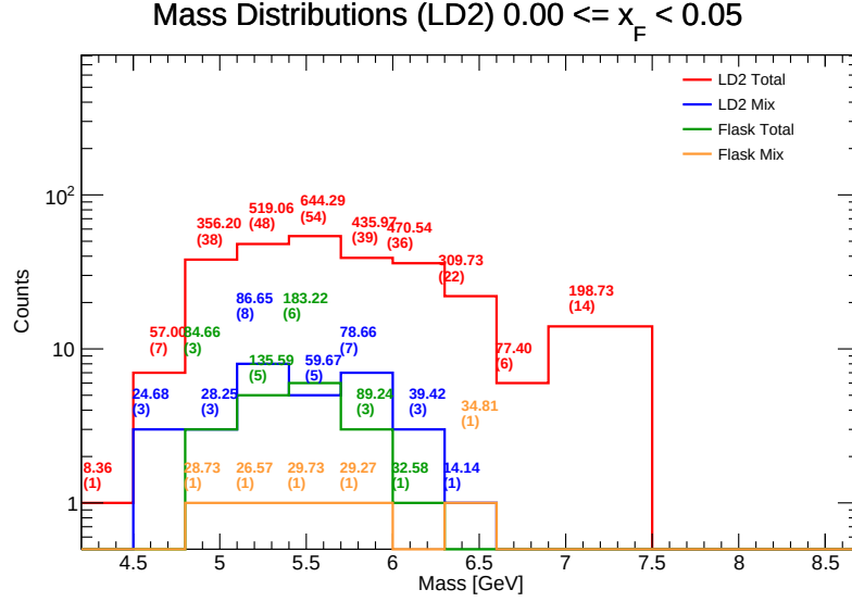
Figure 73: Invariant Mass distributions for LD 2 in the range x_F \in [0.00, 0.05) . Components shown include target total (red), target mix (blue), flask total (green), and flask mix (orange). The values listed above each bin represent the efficiency-weighted corrected mass \sum M/\epsilon and the raw counts ( N ).
