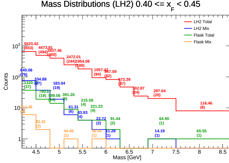
Figure 88: Invariant Mass distributions for LH 2 in the range x_F \in [0.40, 0.45] . Components shown include target total (red), target mix (blue), flask total (green), and flask mix (orange). The values listed above each bin represent the efficiency-weighted corrected mass \sum M/\epsilon and the raw counts ( N ).
