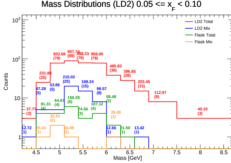
Figure 75: Invariant Mass distributions for LD 2 in the range x_F \in [0.05, 0.10) . Components shown include target total (red), target mix (blue), flask total (green), and flask mix (orange). The values listed above each bin represent the efficiency-weighted corrected mass \sum M/\epsilon and the raw counts ( N ).
