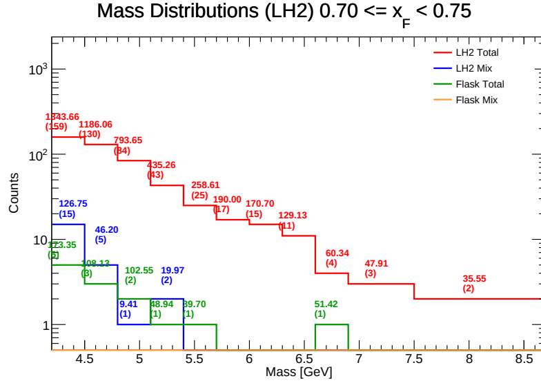
Figure 100: Invariant Mass distributions for LH 2 in the range x_F \in [0.70, 0.75] . Components shown include target total (red), target mix (blue), flask total (green), and flask mix (orange). The values listed above each bin represent the efficiency-weighted corrected mass \sum M/\epsilon and the raw counts ( N ).
