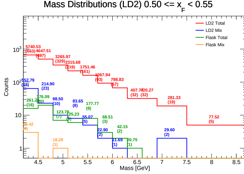
Figure 93: Invariant Mass distributions for LD 2 in the range x_F \in [0.50, 0.55) . Components shown include target total (red), target mix (blue), flask total (green), and flask mix (orange). The values listed above each bin represent the efficiency-weighted corrected mass \sum M/\epsilon and the raw counts ( N ).
