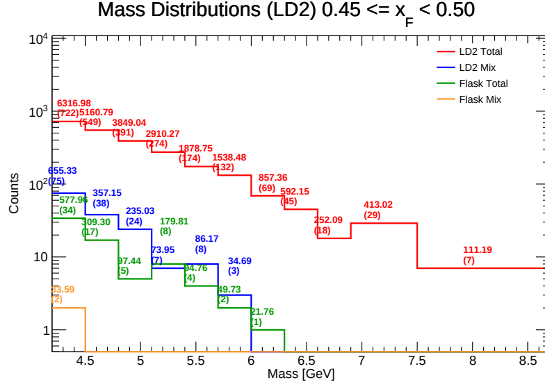
Figure 91: Invariant Mass distributions for LD 2 in the range x_F \in [0.45, 0.50] . Components shown include target total (red), target mix (blue), flask total (green), and flask mix (orange). The values listed above each bin represent the efficiency-weighted corrected mass \sum M/\epsilon and the raw counts ( N ).
