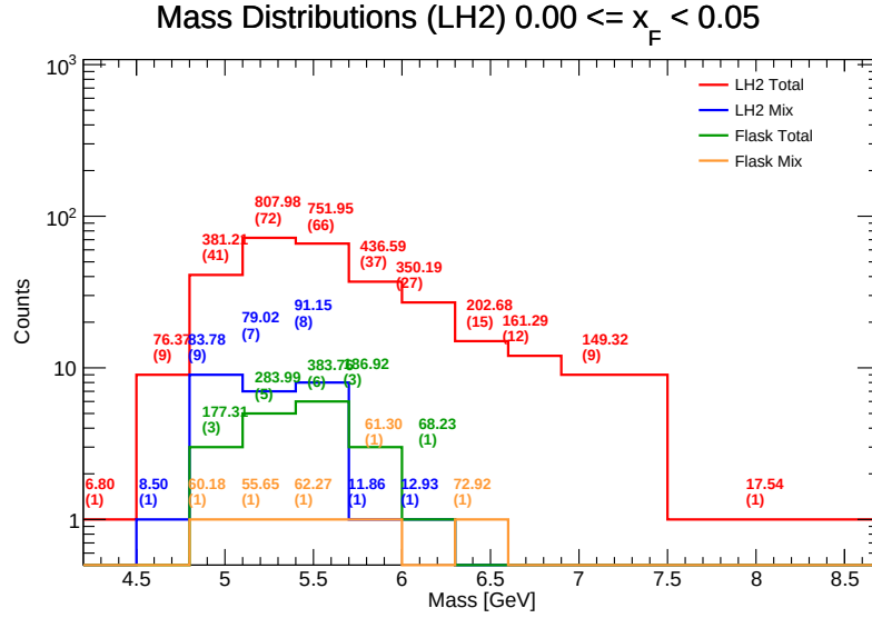
Figure 72: Invariant Mass distributions for LH 2 in the range x_F \in [0.00, 0.05) . Components shown include target total (red), target mix (blue), flask total (green), and flask mix (orange). The values listed above each bin represent the efficiency-weighted corrected mass \sum M/\epsilon and the raw counts ( N ).
