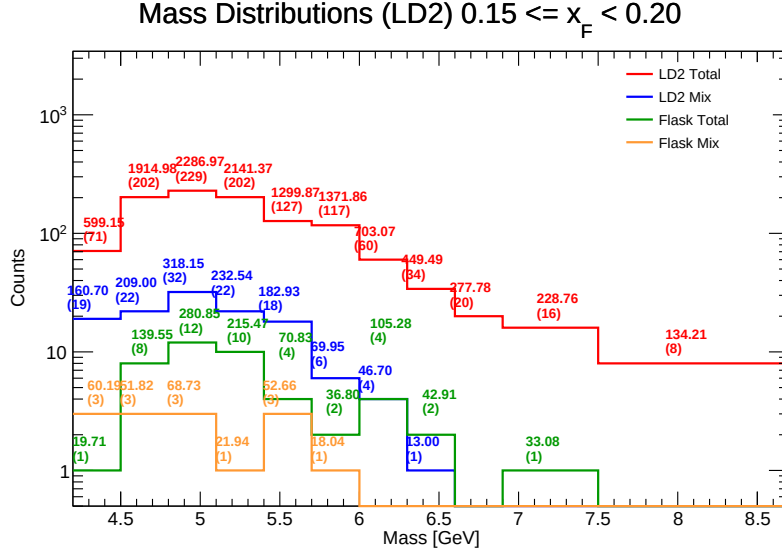
Figure 79: Invariant Mass distributions for LD 2 in the range x_F \in [0.15, 0.20) . Components shown include target total (red), target mix (blue), flask total (green), and flask mix (orange). The values listed above each bin represent the efficiency-weighted corrected mass \sum M/\epsilon and the raw counts ( N ).
