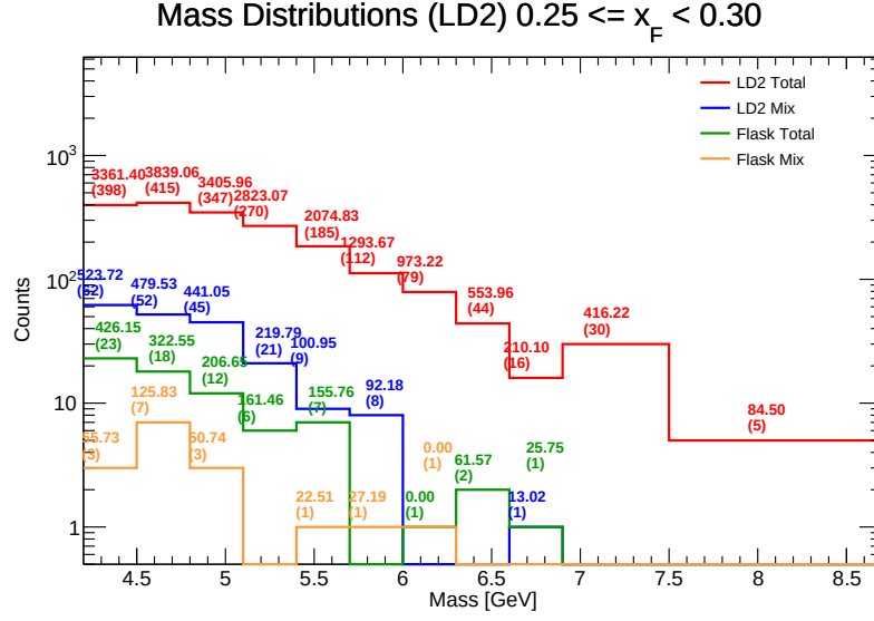
Figure 83: Invariant Mass distributions for LD 2 in the range x_F \in [0.25, 0.30) . Components shown include target total (red), target mix (blue), flask total (green), and flask mix (orange). The values listed above each bin represent the efficiency-weighted corrected mass \sum M/\epsilon and the raw counts ( N ).
