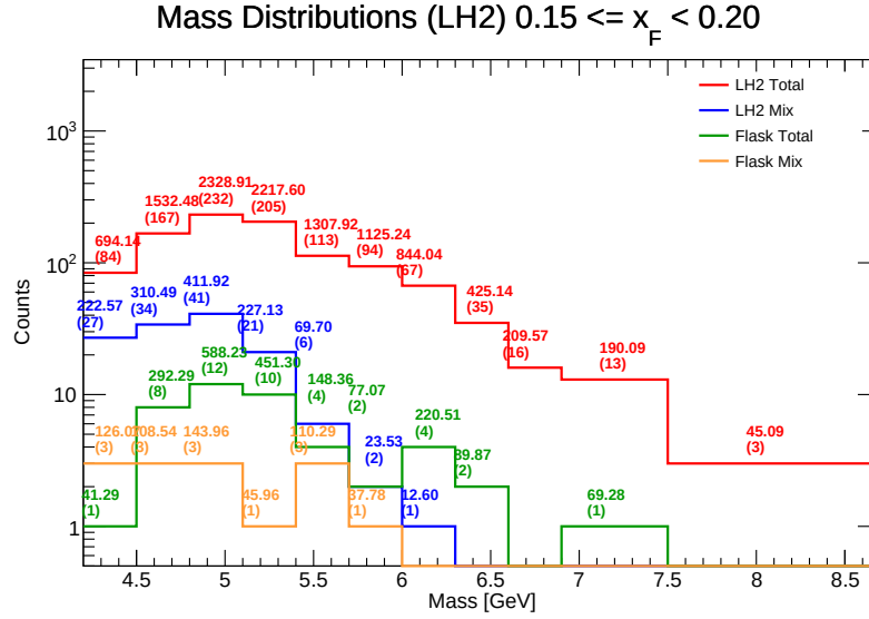
Figure 78: Invariant Mass distributions for LH 2 in the range x_F \in [0.15, 0.20] . Components shown include target total (red), target mix (blue), flask total (green), and flask mix (orange). The values listed above each bin represent the efficiency-weighted corrected mass \sum M/\epsilon and the raw counts ( N ).
