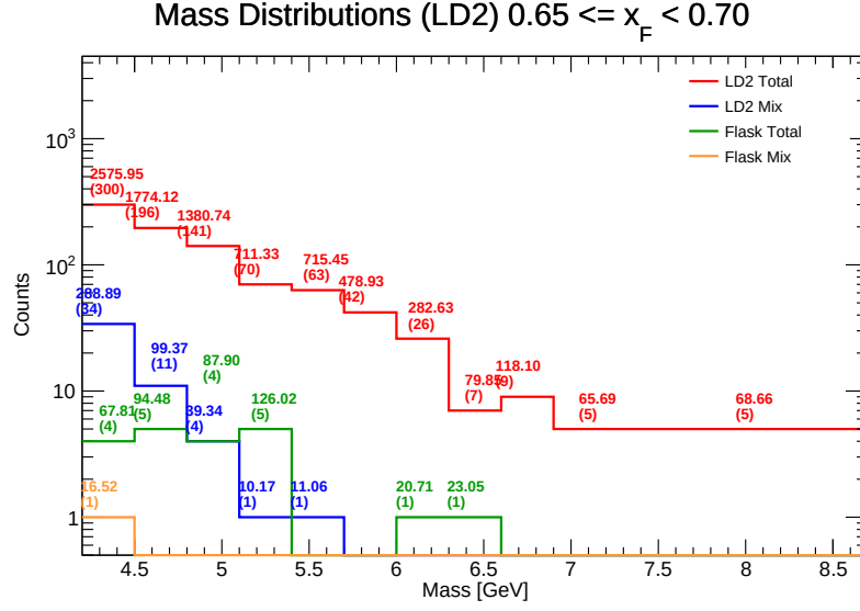
Figure 99: Invariant Mass distributions for LD 2 in the range x_F \in [0.65, 0.70) . Components shown include target total (red), target mix (blue), flask total (green), and flask mix (orange). The values listed above each bin represent the efficiency-weighted corrected mass \sum M/\epsilon and the raw counts ( N ).
