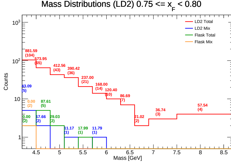
Figure 103: Invariant Mass distributions for LD 2 in the range x_F \in [0.75, 0.80) . Components shown include target total (red), target mix (blue), flask total (green), and flask mix (orange). The values listed above each bin represent the efficiency-weighted corrected mass \sum M/\epsilon and the raw counts ( N ).
