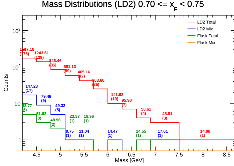
Figure 101: Invariant Mass distributions for LD 2 in the range x_F \in [0.70, 0.75) . Components shown include target total (red), target mix (blue), flask total (green), and flask mix (orange). The values listed above each bin represent the efficiency-weighted corrected mass \sum M/\epsilon and the raw counts ( N ).
