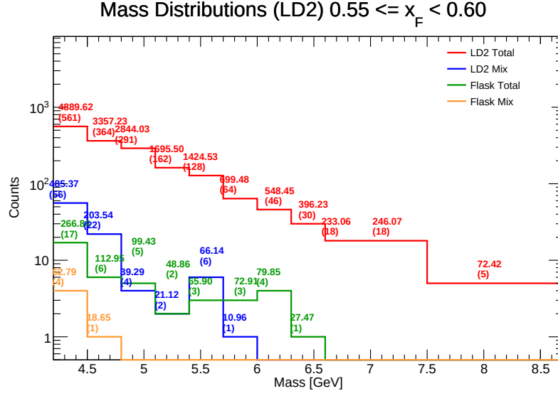
Figure 95: Invariant Mass distributions for LD 2 in the range x_F \in [0.55, 0.60) . Components shown include target total (red), target mix (blue), flask total (green), and flask mix (orange). The values listed above each bin represent the efficiency-weighted corrected mass \sum M/\epsilon and the raw counts ( N ).
