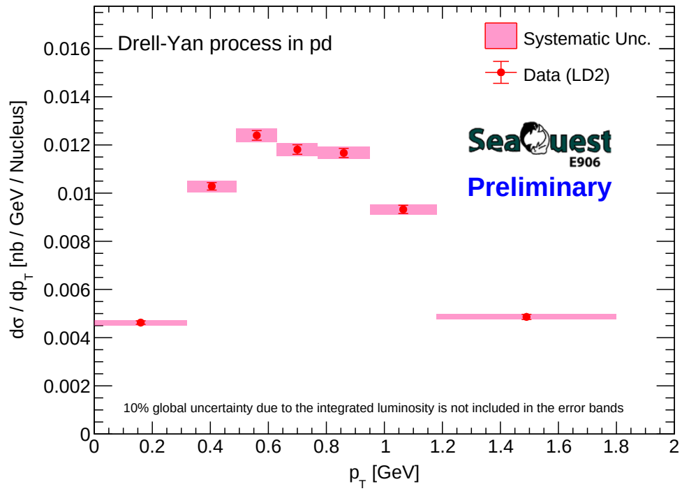
Figure 31: CrossSection_LD2_vs_pT_with_logo
