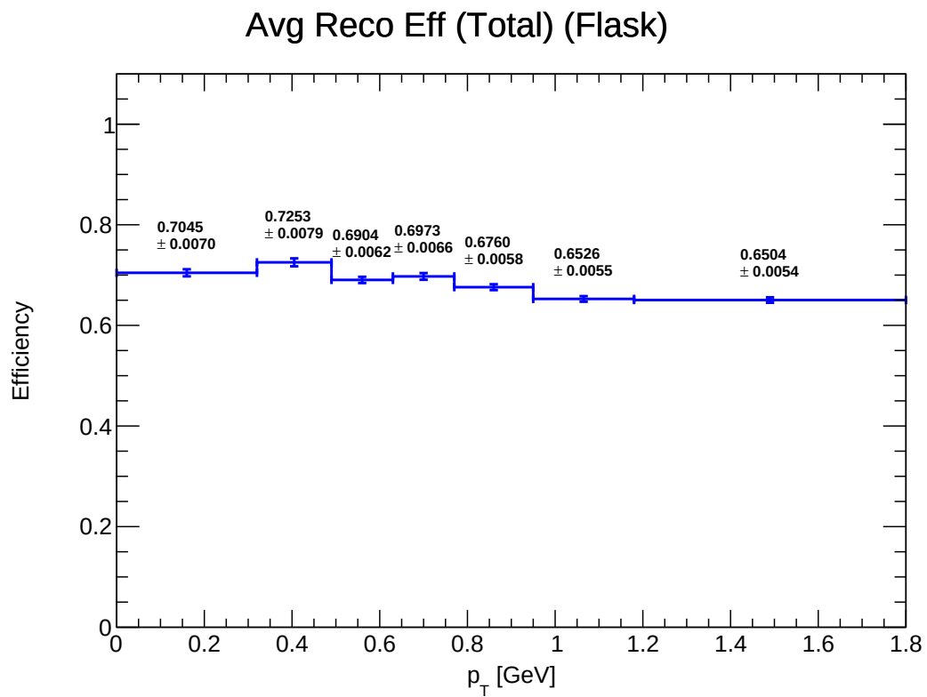
Figure 11: E_total_reco_Flask
