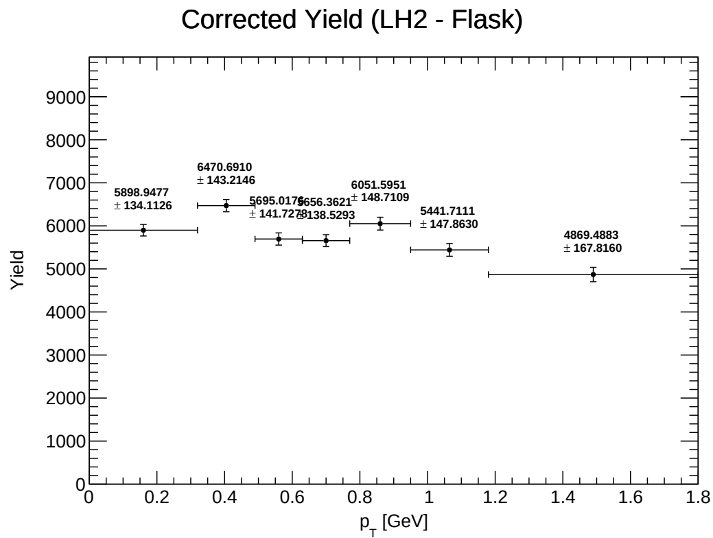
Figure 28: Y_{\text{corrected\_Subtracted\_LH2}}
