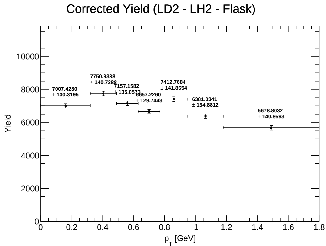
Figure 29: Y_corrected_Subtracted_LD2
