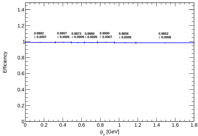
Avg Hodo Eff (Total) (Flask)
