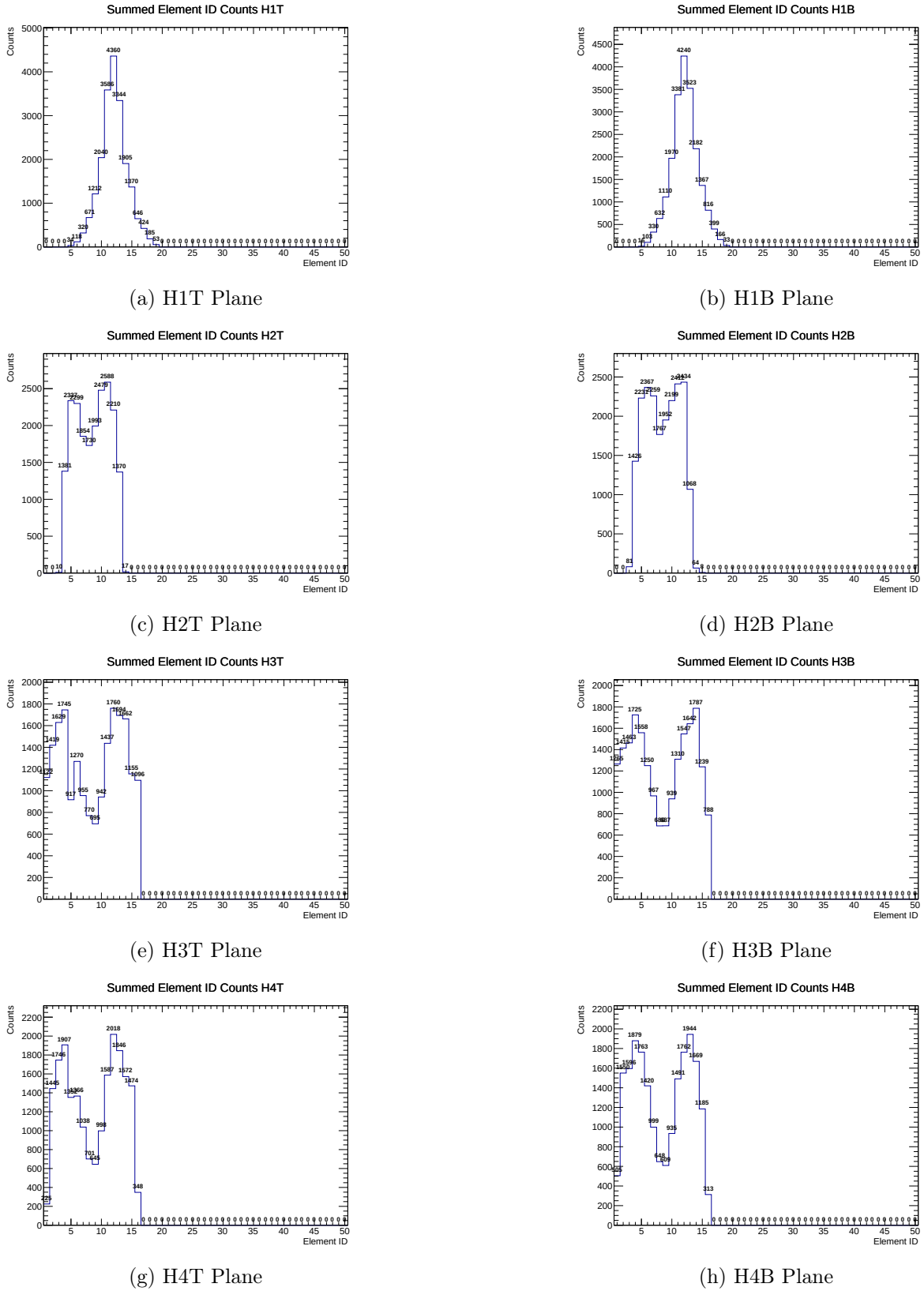
Figure 7: Hodoscope Paddle hit distributions arranged by Plane (Rows 1-4), Top vs Bottom.
