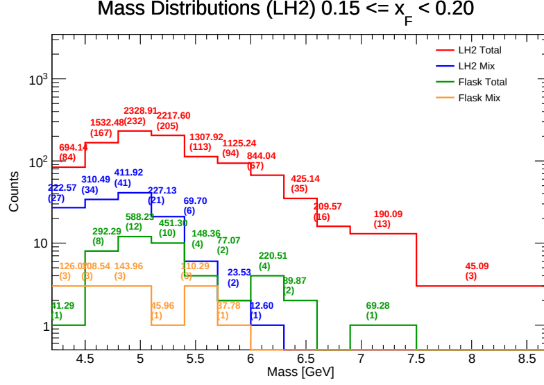
Figure 85: Invariant Mass distributions for LH 2 in the range x_F \in [0.15, 0.20] . Components shown include target total (red), target mix (blue), flask total (green), and flask mix (orange). The values listed above each bin represent the efficiency-weighted corrected mass \sum M/\epsilon and the raw counts ( N ).
