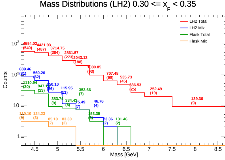
Figure 91: Invariant Mass distributions for LH 2 in the range x_F \in [0.30, 0.35] . Components shown include target total (red), target mix (blue), flask total (green), and flask mix (orange). The values listed above each bin represent the efficiency-weighted corrected mass \sum M/\epsilon and the raw counts ( N ).
