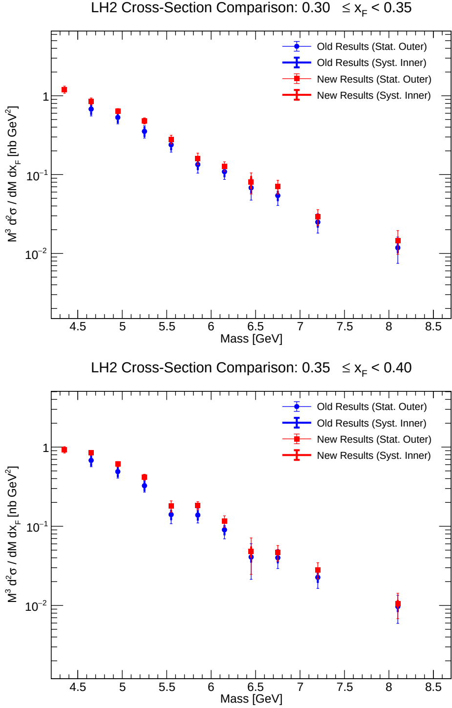
Figure 54: Comparison of double-differential cross-section for LH2 ( x_F bins 0.30-0.40).
