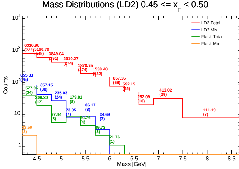
Figure 98: Invariant Mass distributions for LD 2 in the range x_F \in [0.45, 0.50] . Components shown include target total (red), target mix (blue), flask total (green), and flask mix (orange). The values listed above each bin represent the efficiency-weighted corrected mass \sum M/\epsilon and the raw counts ( N ).
