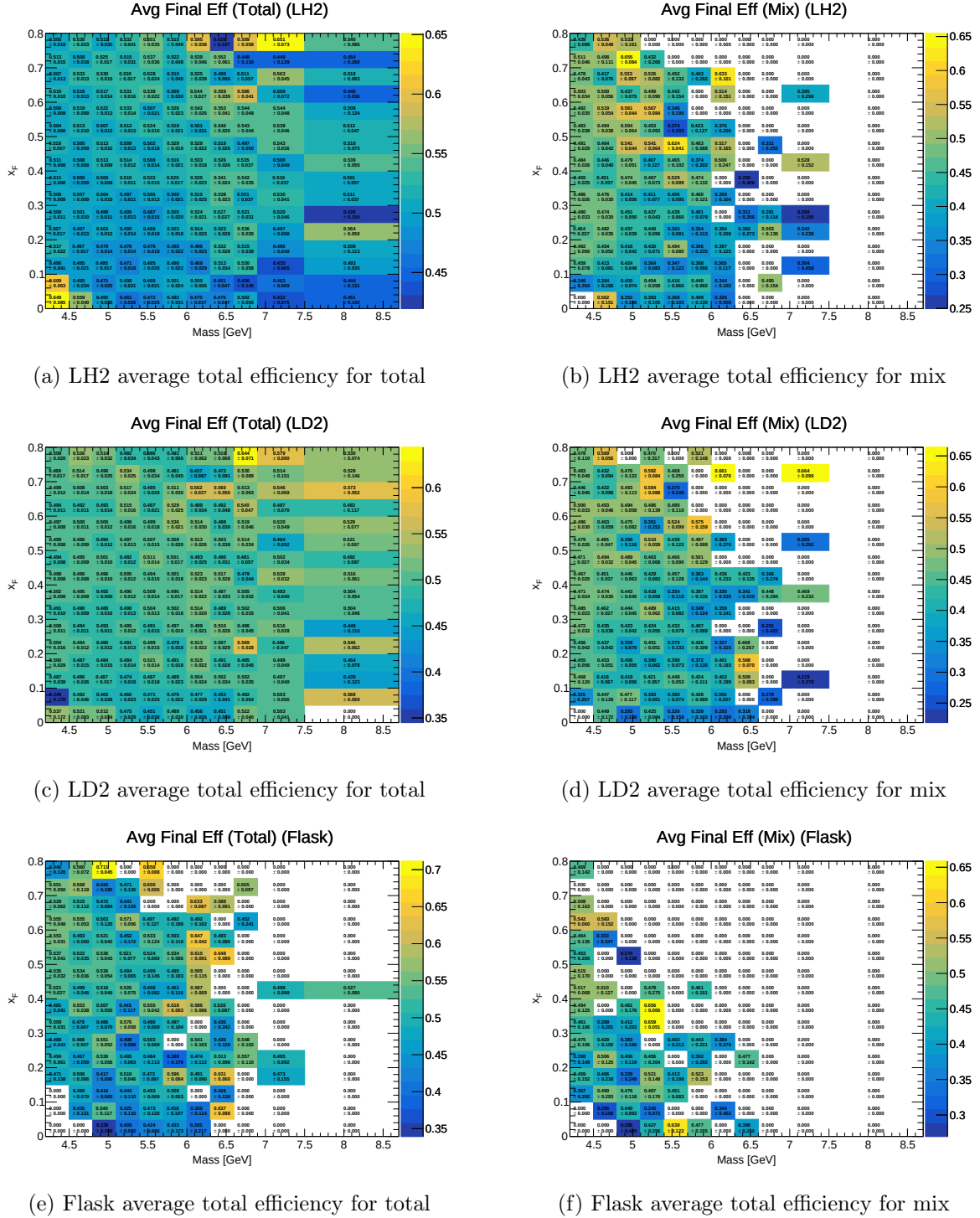
Figure 10: Average total Efficiencies calculated each kinematic bin with the propagated uncertainties.
