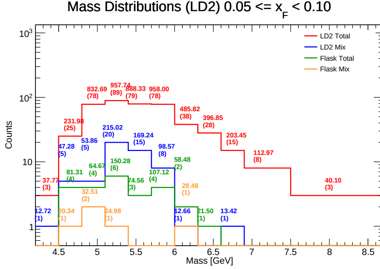
Figure 82: Invariant Mass distributions for LD 2 in the range x_F \in [0.05, 0.10) . Components shown include target total (red), target mix (blue), flask total (green), and flask mix (orange). The values listed above each bin represent the efficiency-weighted corrected mass \sum M/\epsilon and the raw counts ( N ).
