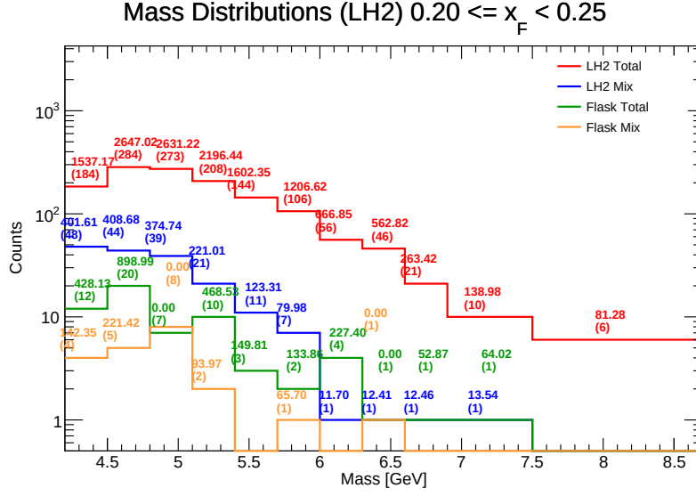
Figure 87: Invariant Mass distributions for LH 2 in the range x_F \in [0.20, 0.25] . Components shown include target total (red), target mix (blue), flask total (green), and flask mix (orange). The values listed above each bin represent the efficiency-weighted corrected mass \sum M/\epsilon and the raw counts ( N ).
