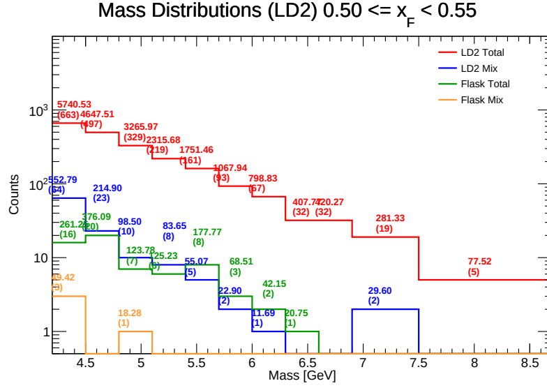
Figure 100: Invariant Mass distributions for LD 2 in the range x_F \in [0.50, 0.55) . Components shown include target total (red), target mix (blue), flask total (green), and flask mix (orange). The values listed above each bin represent the efficiency-weighted corrected mass \sum M/\epsilon and the raw counts ( N ).
