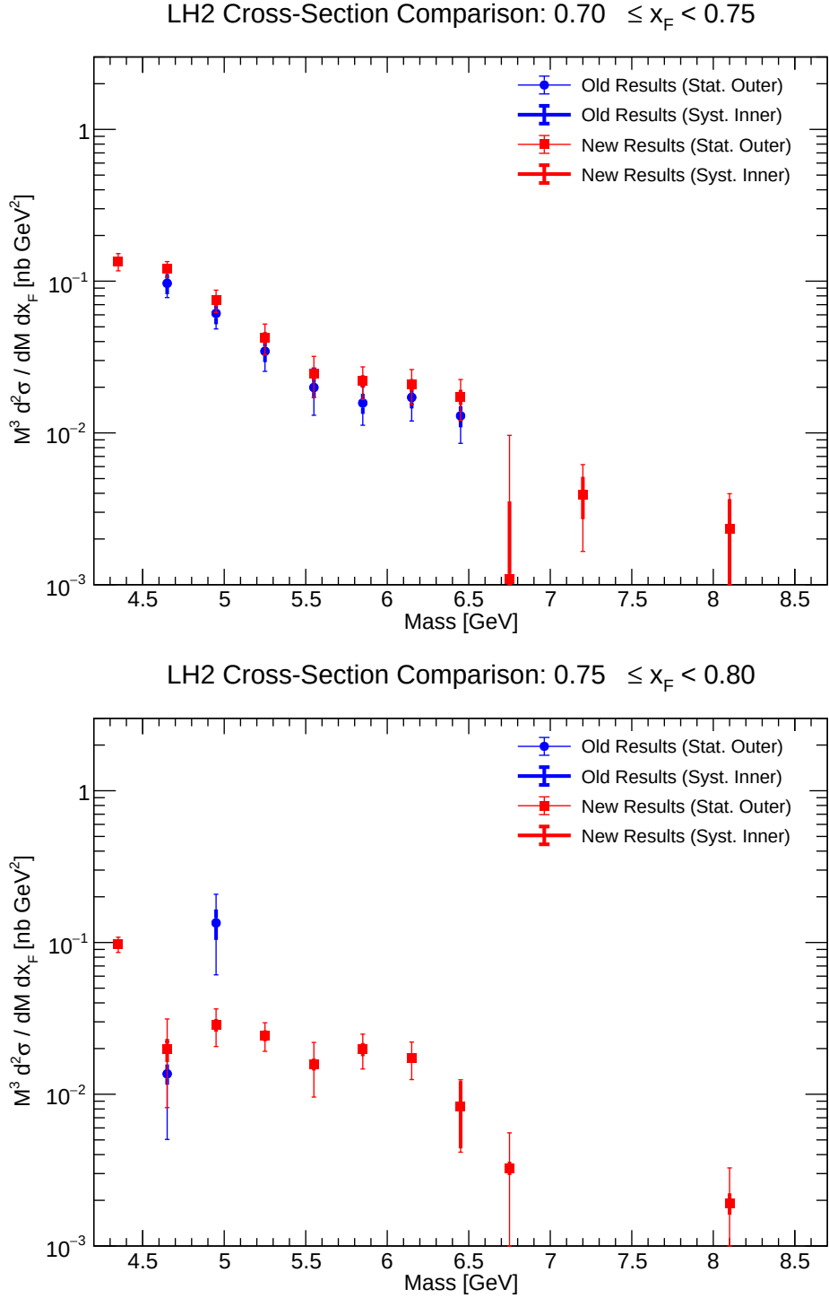
Figure 58: Comparison of double-differential cross-section for LH2 ( x_F bins 0.70-0.80).
