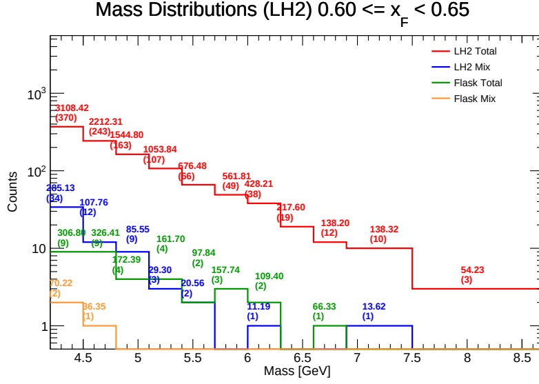
Figure 103: Invariant Mass distributions for LH 2 in the range x_F \in [0.60, 0.65] . Components shown include target total (red), target mix (blue), flask total (green), and flask mix (orange). The values listed above each bin represent the efficiency-weighted corrected mass \sum M/\epsilon and the raw counts ( N ).
