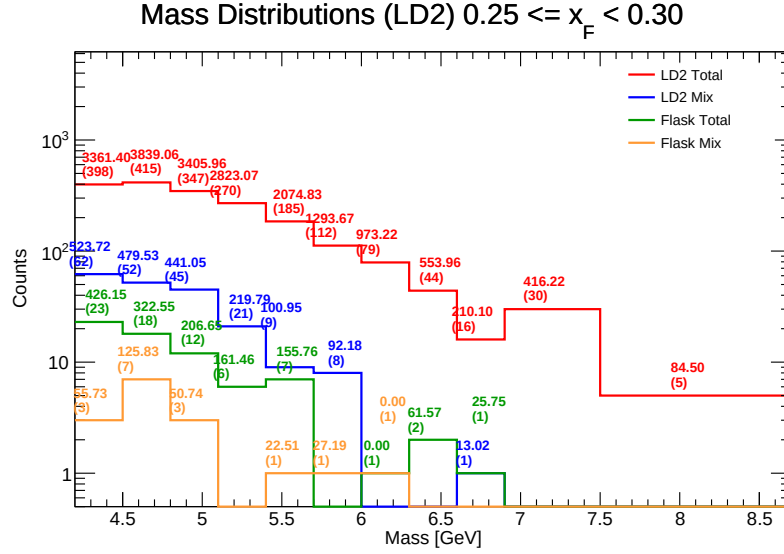
Figure 90: Invariant Mass distributions for LD 2 in the range x_F \in [0.25, 0.30) . Components shown include target total (red), target mix (blue), flask total (green), and flask mix (orange). The values listed above each bin represent the efficiency-weighted corrected mass \sum M/\epsilon and the raw counts ( N ).
