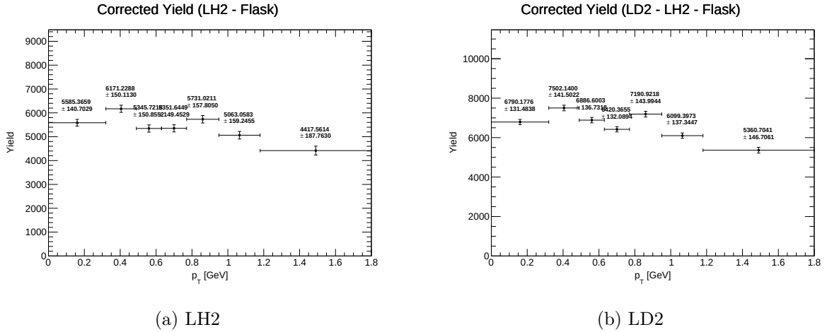
Figure 15: Corrected yields for LH2 (a) and LD2 (b) after correcting for efficiencies, with propagated uncertainties.
