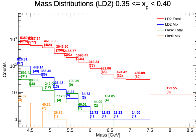
Figure 94: Invariant Mass distributions for LD 2 in the range x_F \in [0.35, 0.40) . Components shown include target total (red), target mix (blue), flask total (green), and flask mix (orange). The values listed above each bin represent the efficiency-weighted corrected mass \sum M/\epsilon and the raw counts ( N ).
