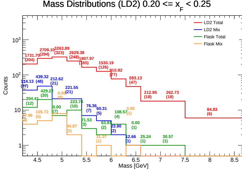
Figure 88: Invariant Mass distributions for LD 2 in the range x_F \in [0.20, 0.25] . Components shown include target total (red), target mix (blue), flask total (green), and flask mix (orange). The values listed above each bin represent the efficiency-weighted corrected mass \sum M/\epsilon and the raw counts ( N ).
