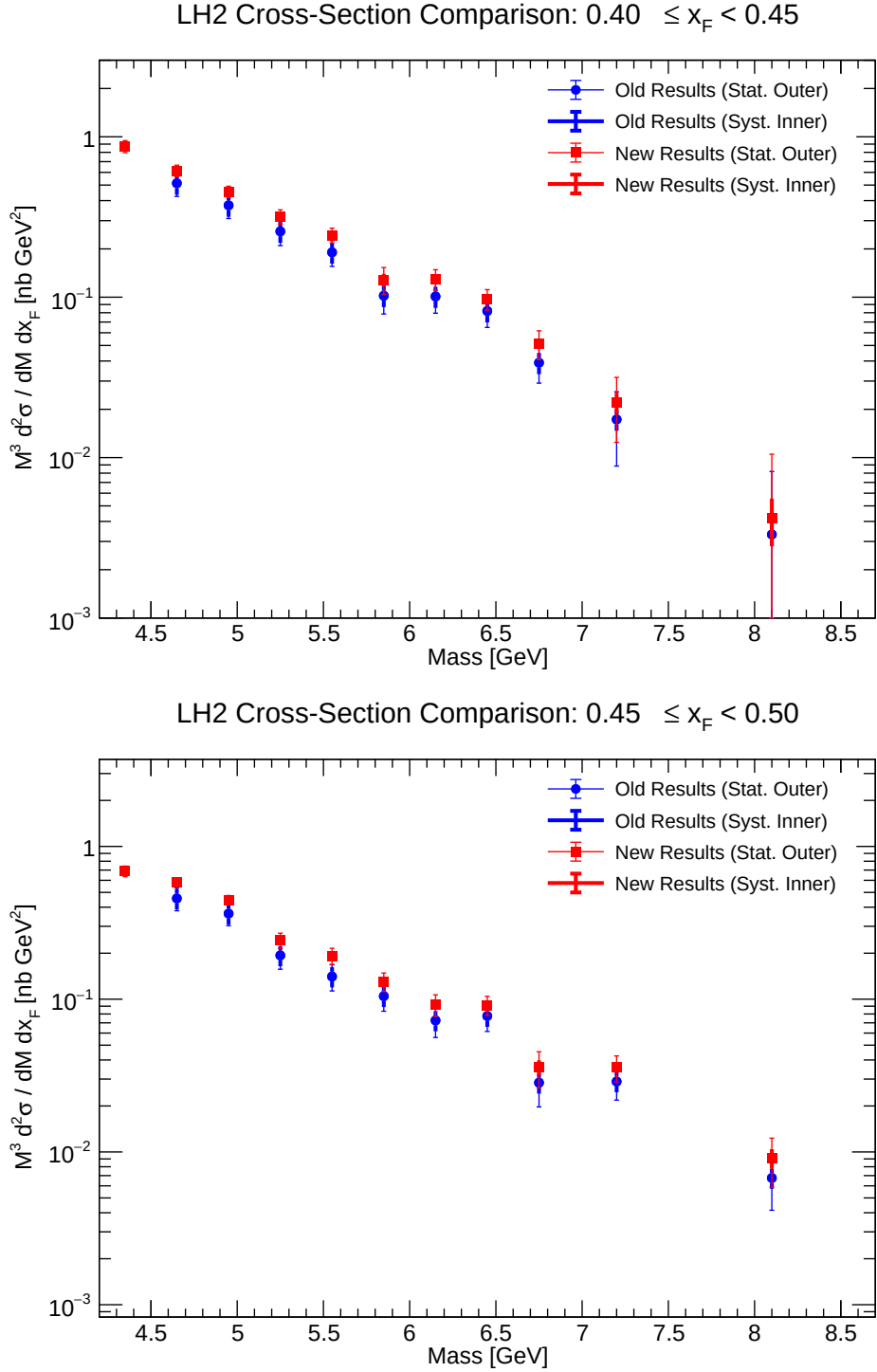
Figure 55: Comparison of double-differential cross-section for LH2 ( x_F bins 0.40-0.50).
