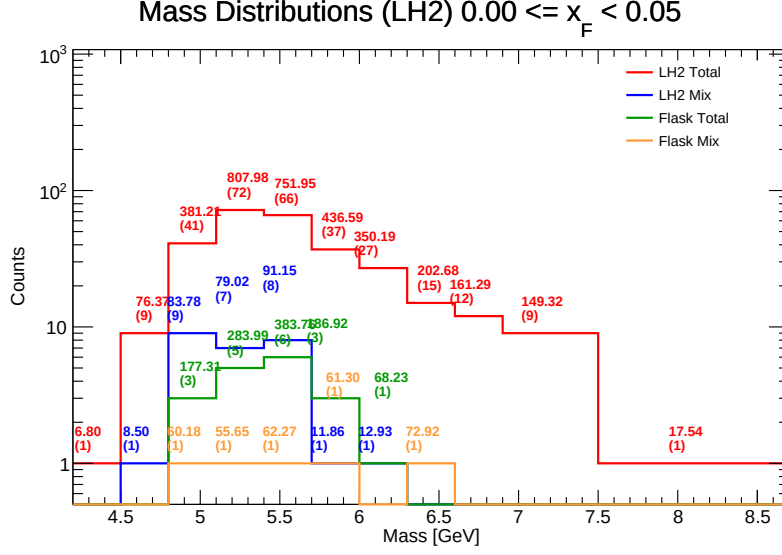
Figure 79: Invariant Mass distributions for LH 2 in the range x_F \in [0.00, 0.05) . Components shown include target total (red), target mix (blue), flask total (green), and flask mix (orange). The values listed above each bin represent the efficiency-weighted corrected mass \sum M/\epsilon and the raw counts ( N ).
