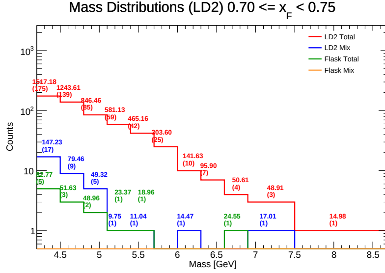
Figure 108: Invariant Mass distributions for LD 2 in the range x_F \in [0.70, 0.75] . Components shown include target total (red), target mix (blue), flask total (green), and flask mix (orange). The values listed above each bin represent the efficiency-weighted corrected mass \sum M/\epsilon and the raw counts ( N ).
