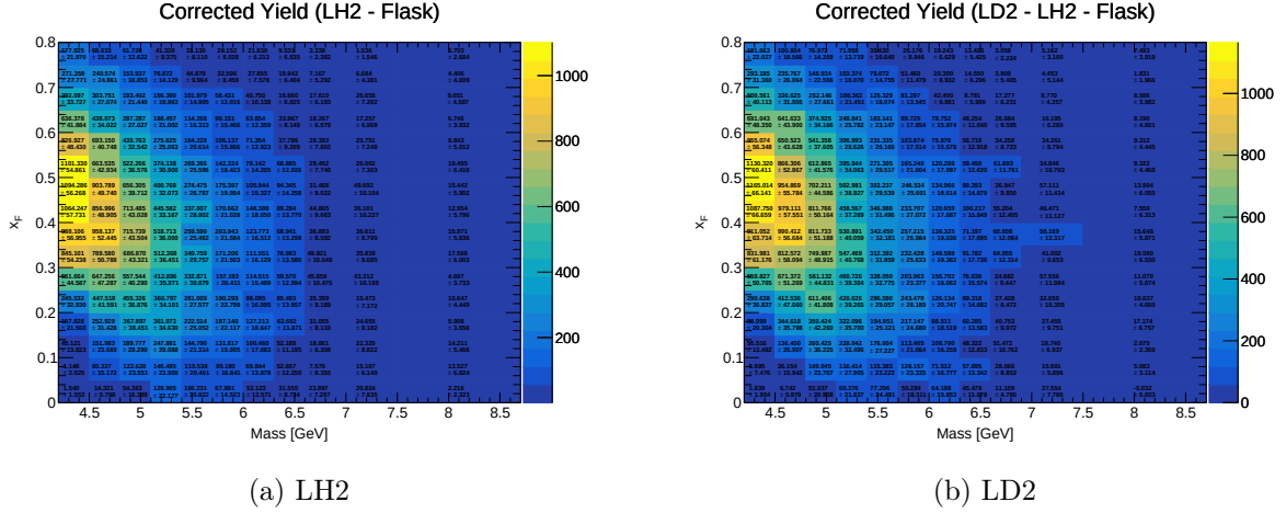
Figure 14: Corrected yields for LH2 (a) and LD2 (b) after correcting for efficiencies, with propagated uncertainties.
