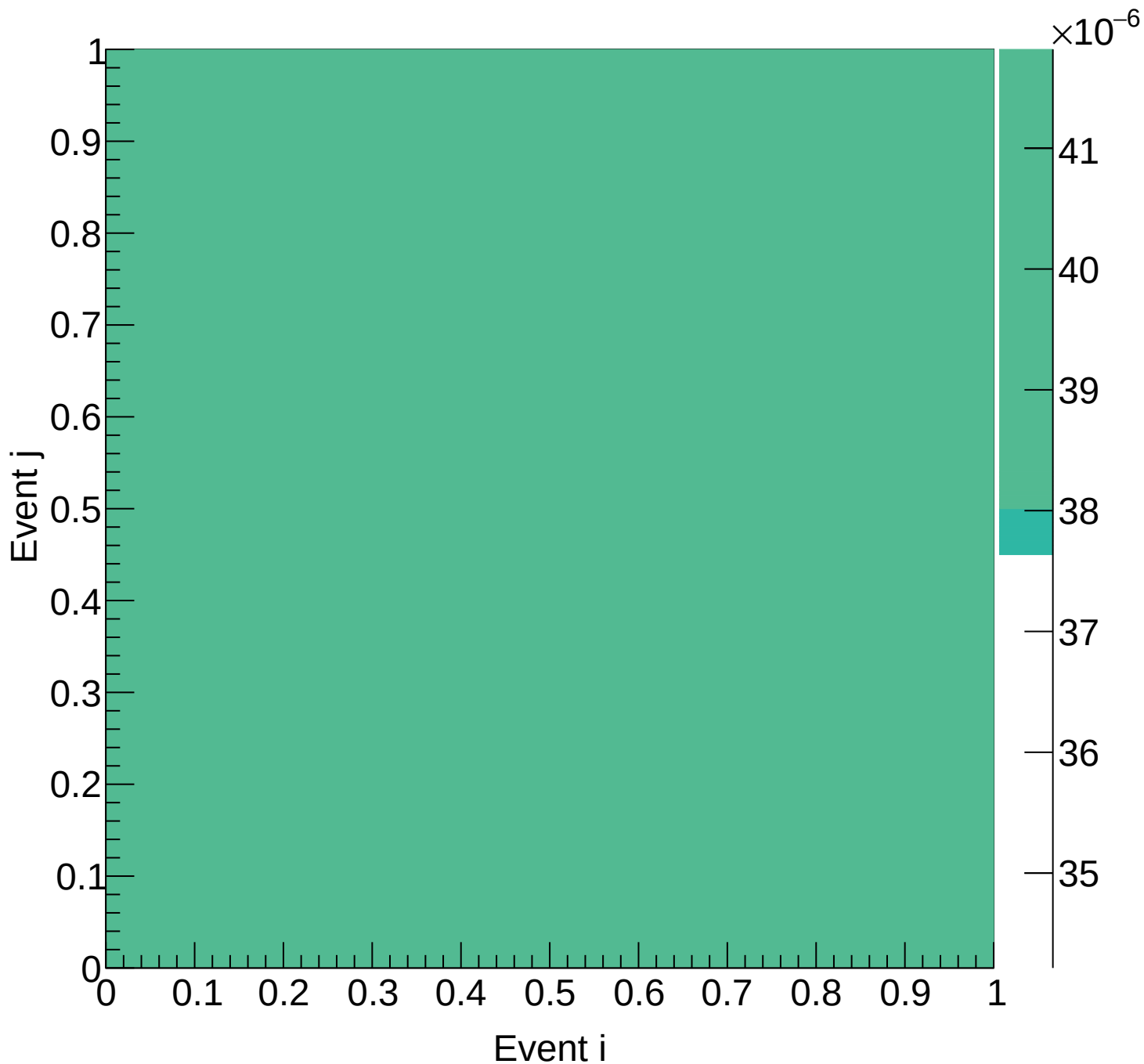
Flask (mix) Covariance | M: [6.3, 6.6) xF: [0.00, 0.05)
