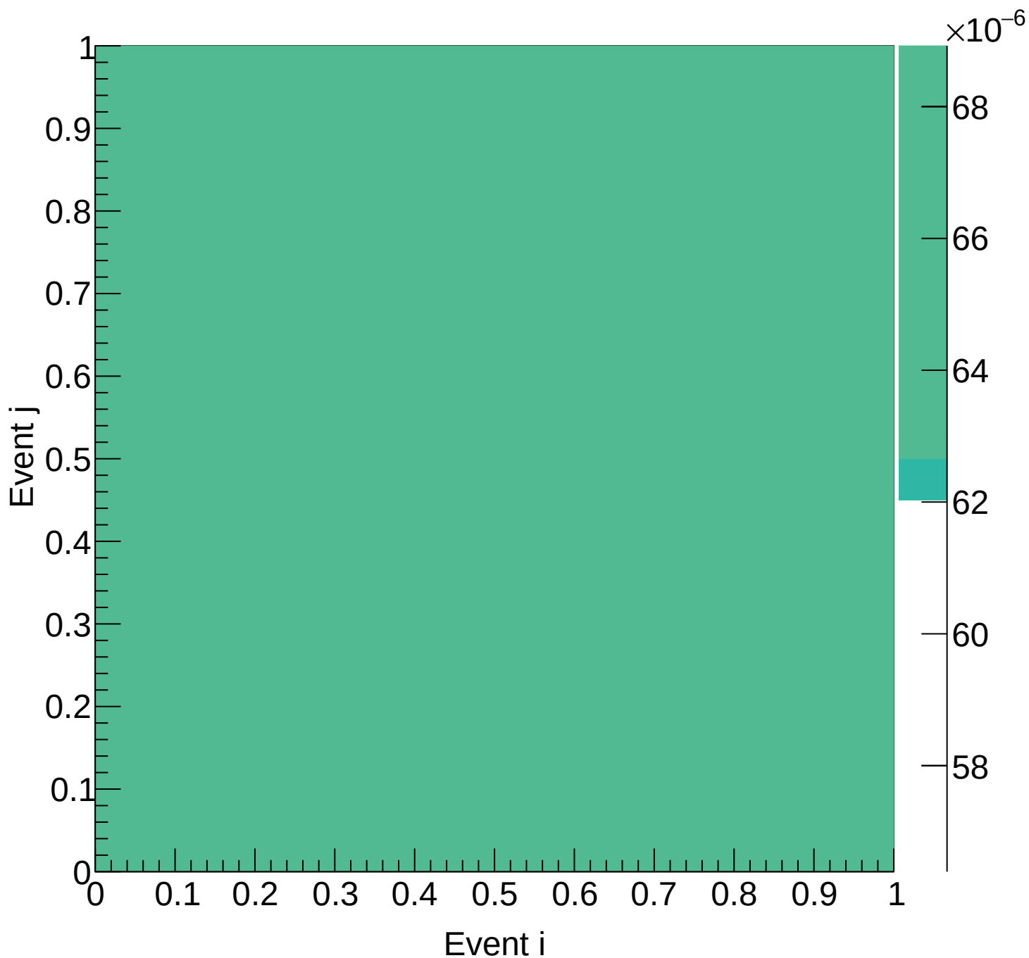
Flask (mix) Covariance | M: [4.8, 5.1) xF: [0.50, 0.55)
