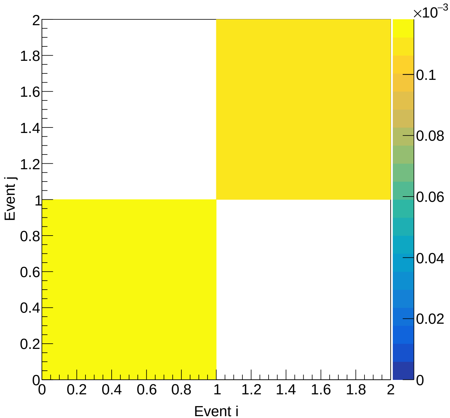
Flask (mix) Covariance | M: [3.9, 4.2) xF: [0.60, 0.65)
