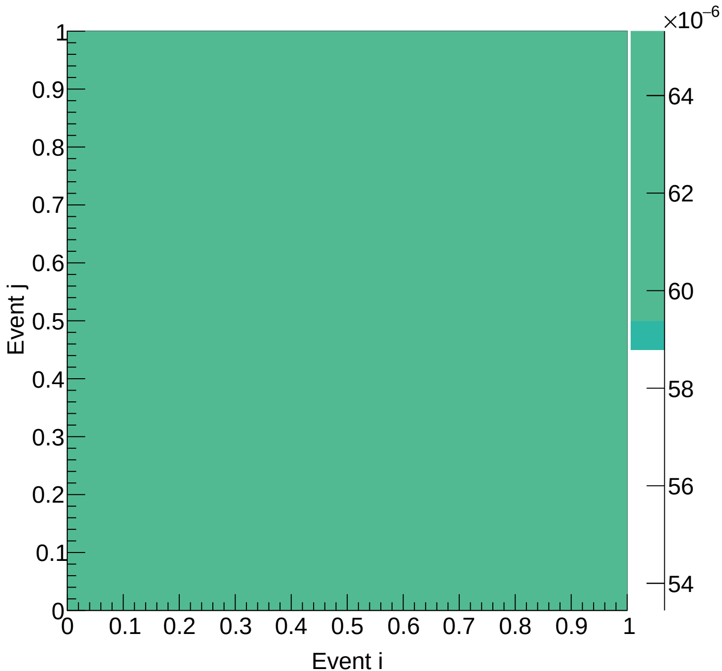
Flask (mix) Covariance | M: [3.9, 4.2) xF: [0.70, 0.75)
