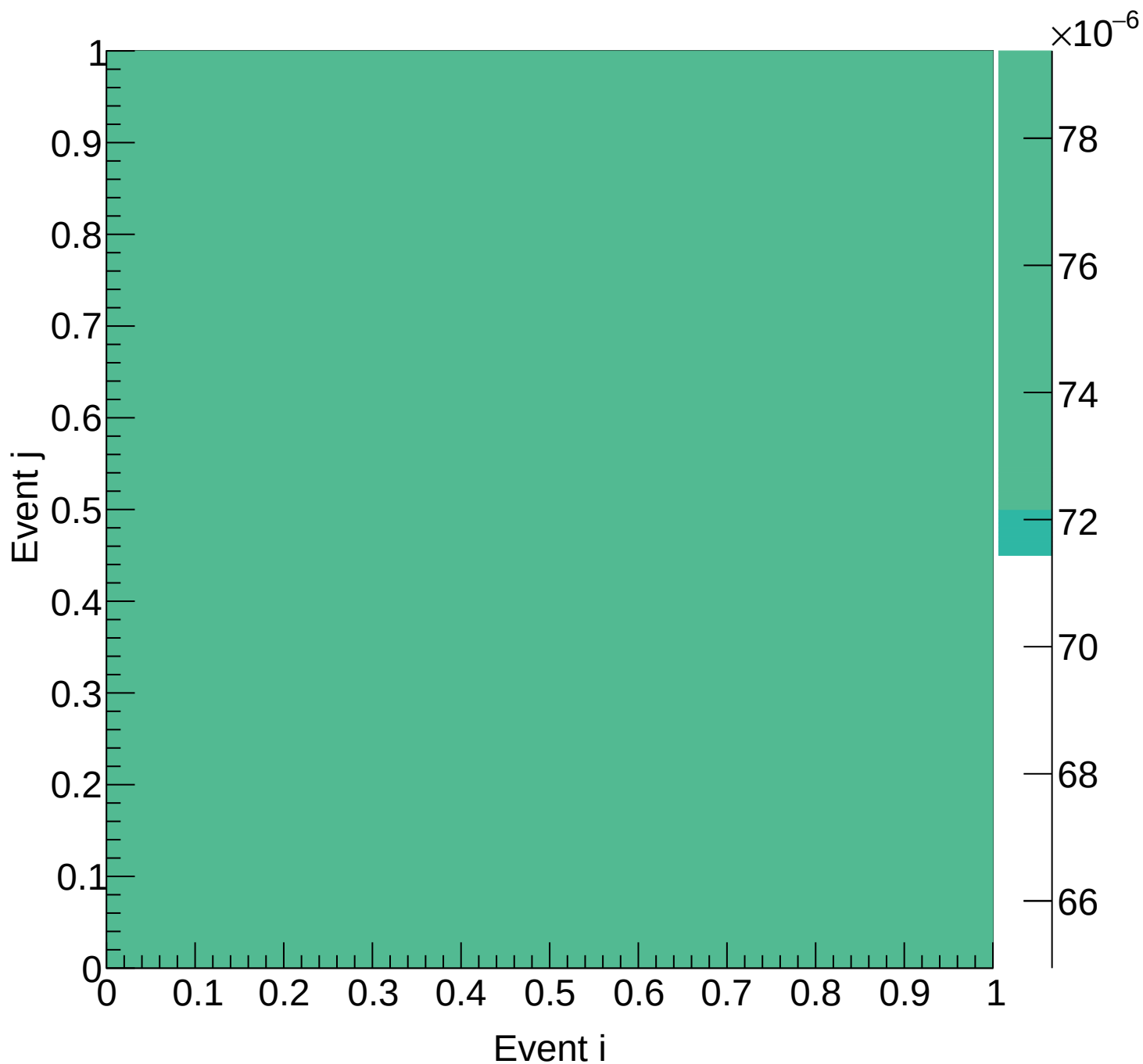
Flask (mix) Covariance | M: [4.5, 4.8) xF: [0.05, 0.10)
