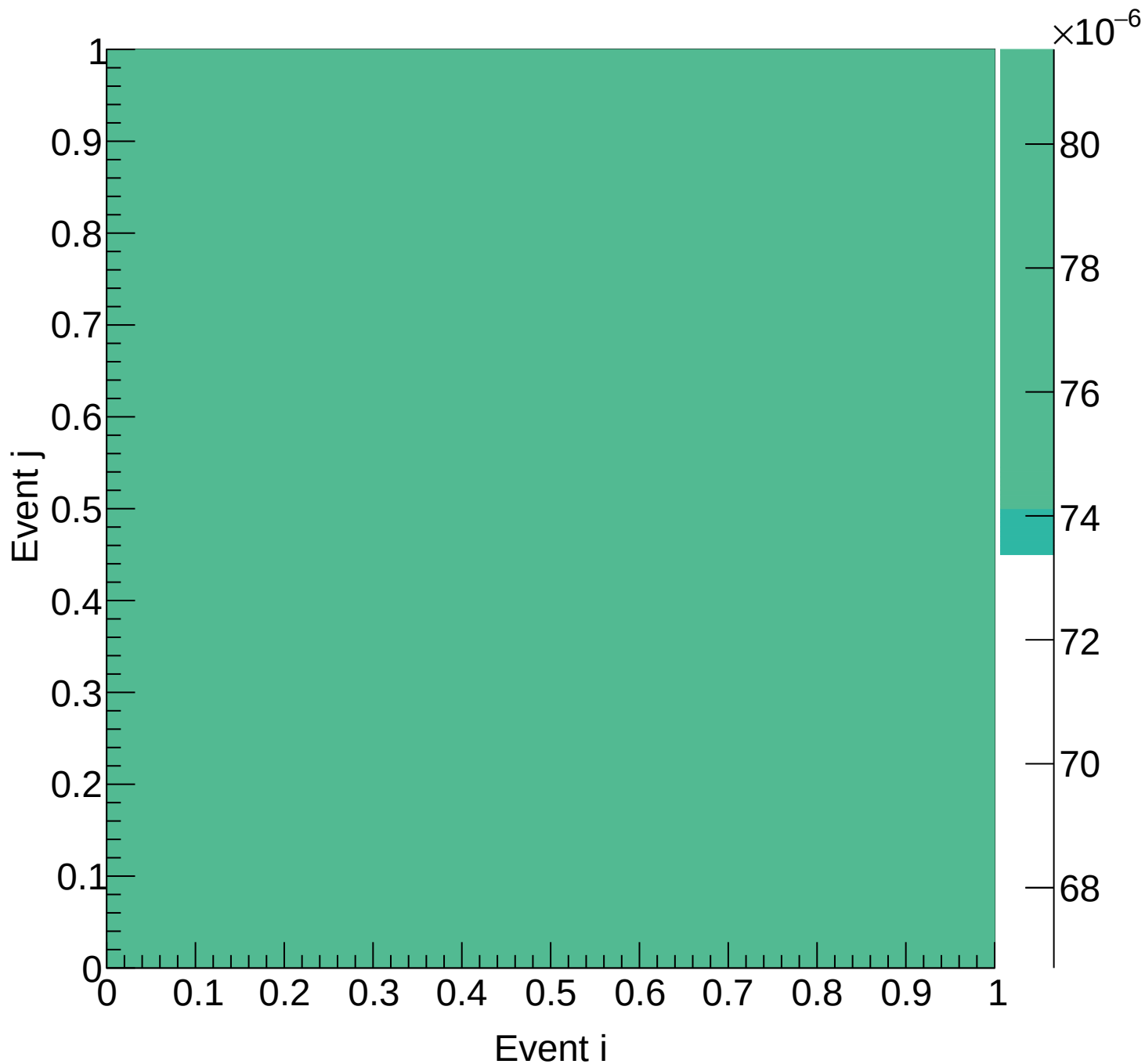
Flask (mix) Covariance | M: [5.4, 5.7) xF: [0.10, 0.15)
