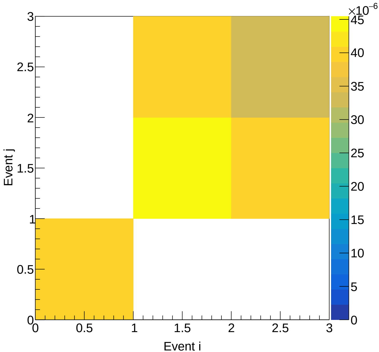
Flask (mix) Covariance | M: [4.5, 4.8) xF: [0.15, 0.20)
