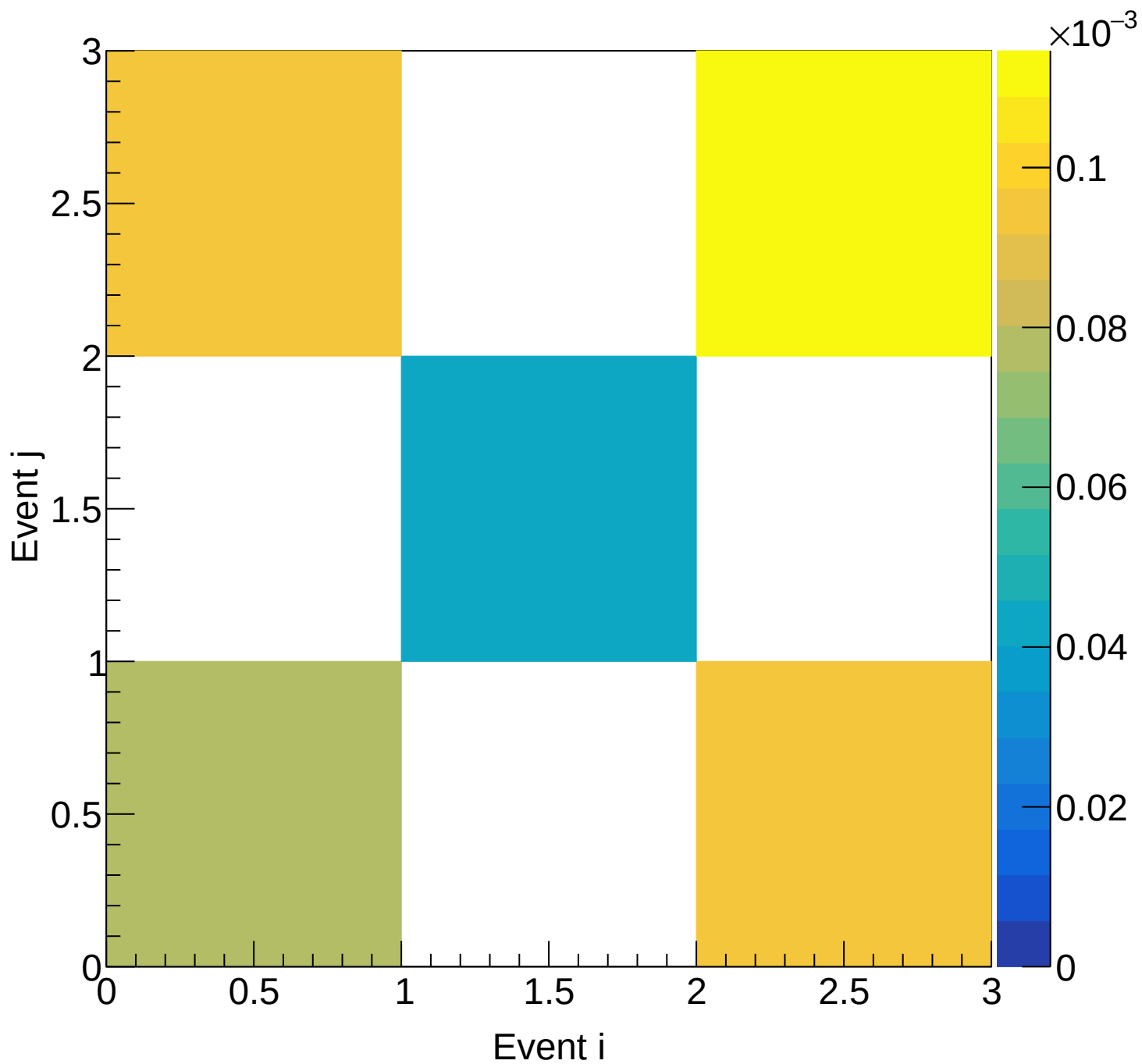
Flask (mix) Covariance | M: [4.8, 5.1) xF: [0.15, 0.20)
