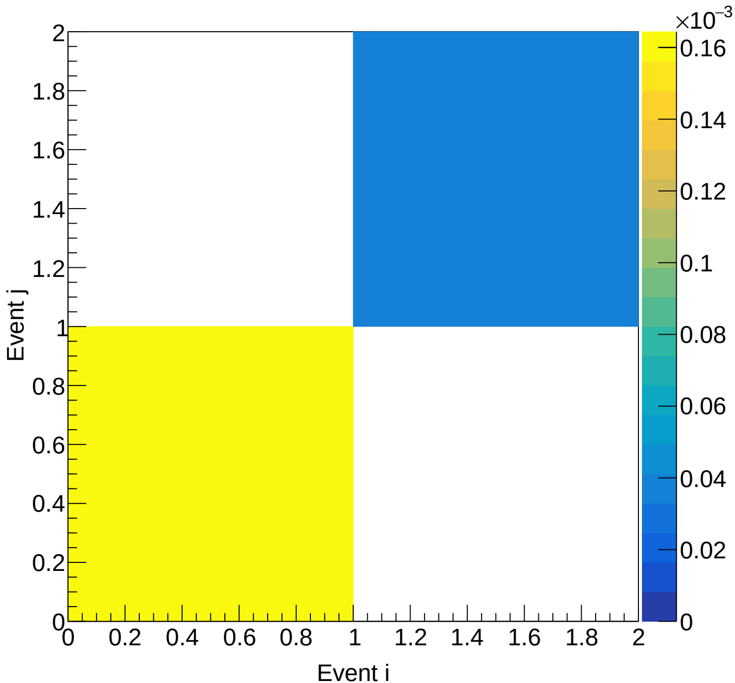
Flask (mix) Covariance | M: [5.1, 5.4) xF: [0.20, 0.25)
