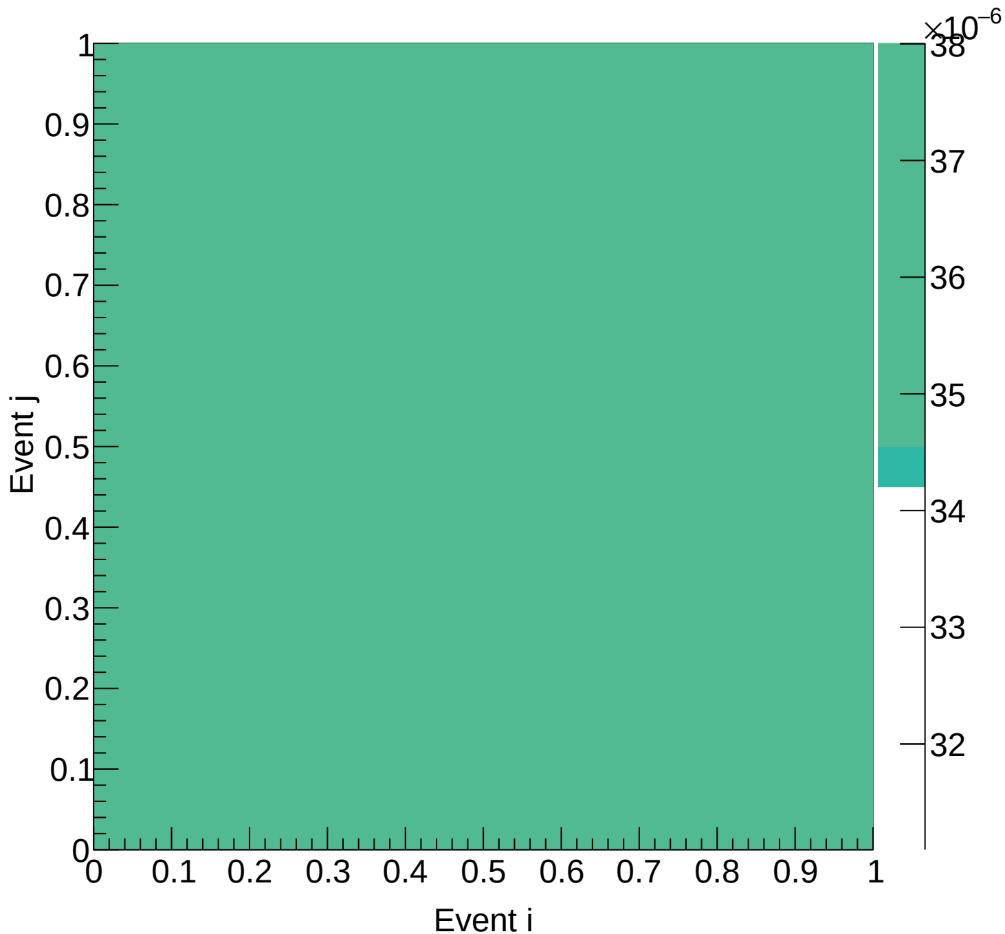
Flask (mix) Covariance | M: [5.7, 6.0) xF: [0.20, 0.25)
