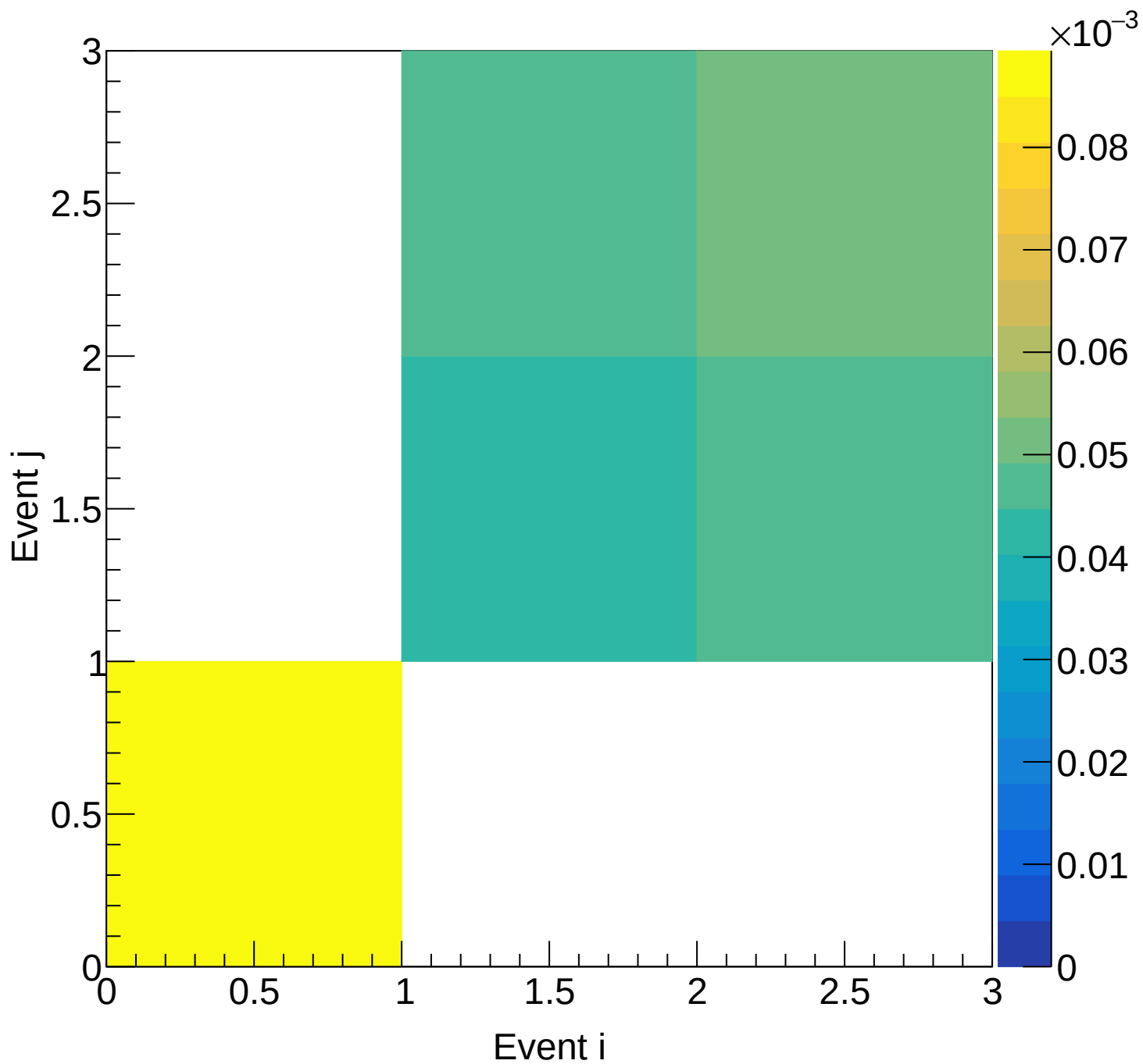
Flask (mix) Covariance | M: [3.9, 4.2) xF: [0.25, 0.30)
