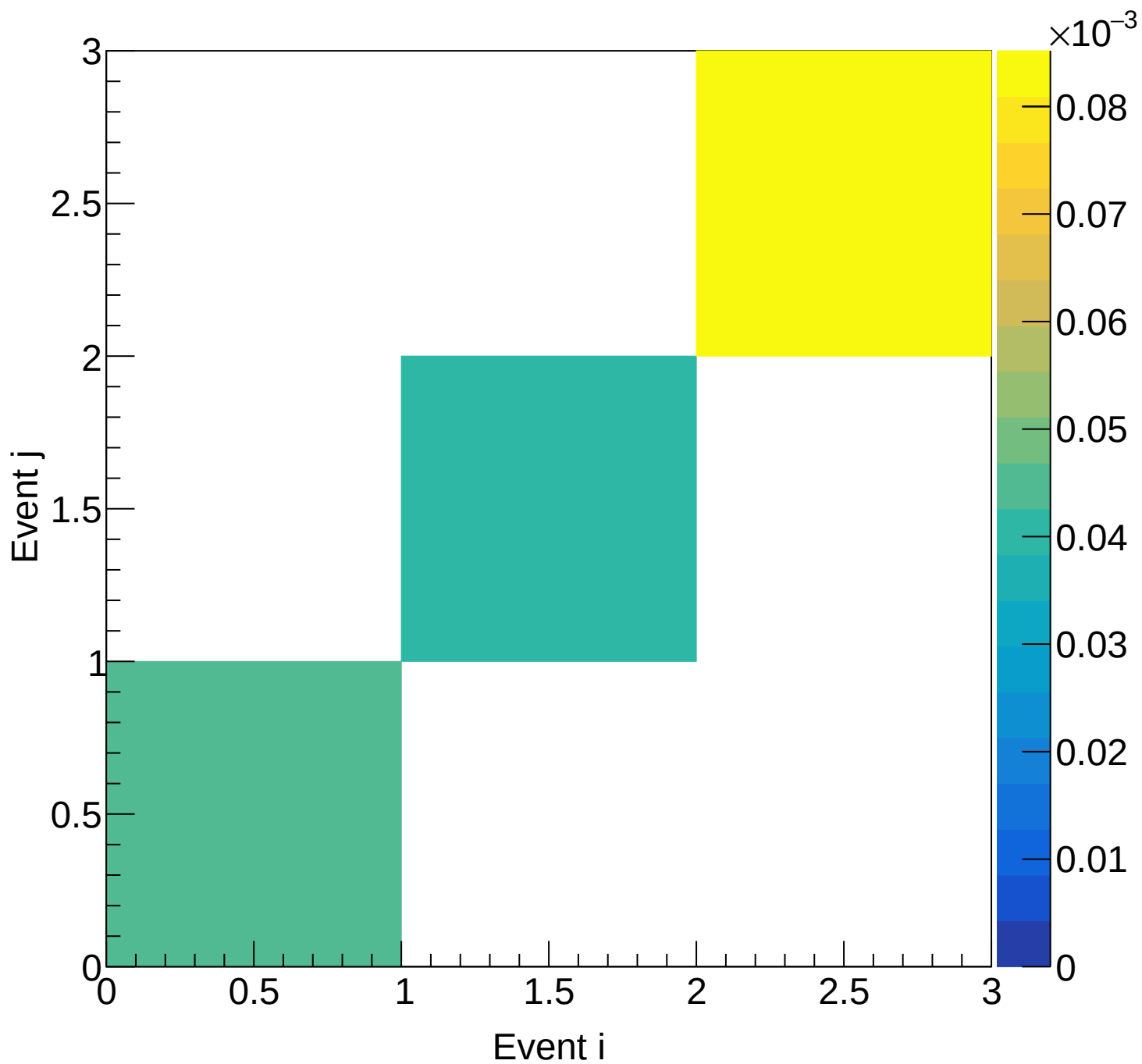
Flask (mix) Covariance | M: [4.8, 5.1) xF: [0.25, 0.30)
