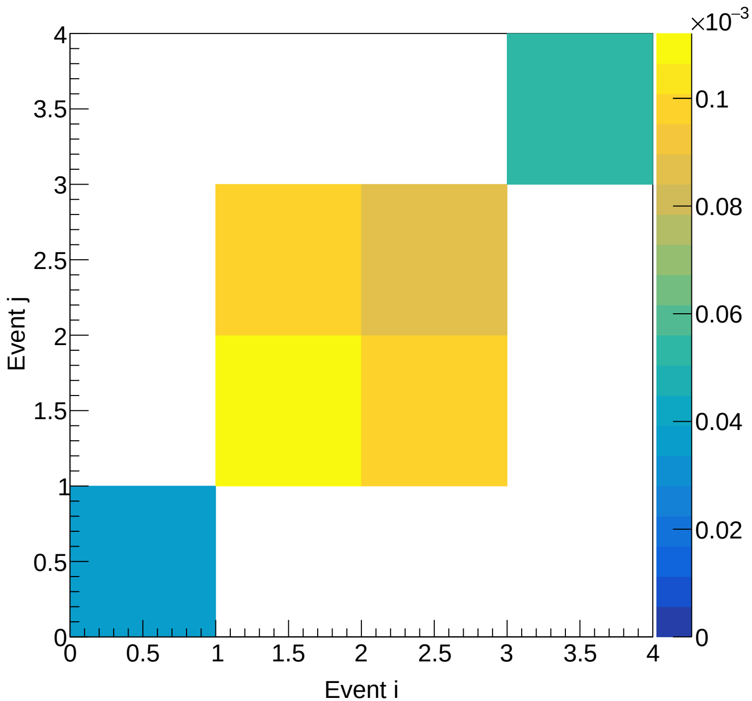
Flask (mix) Covariance | M: [4.2, 4.5) xF: [0.35, 0.40)
