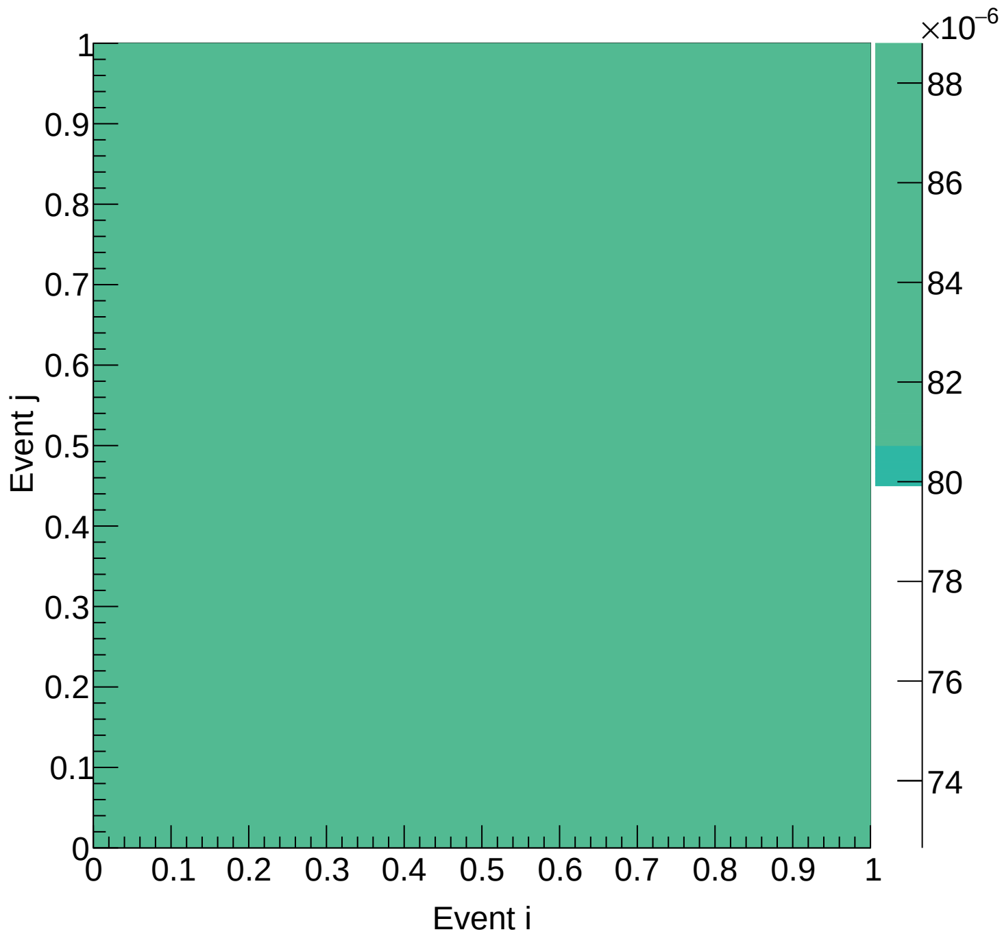
Flask (mix) Covariance | M: [5.7, 6.0) xF: [0.40, 0.45)
