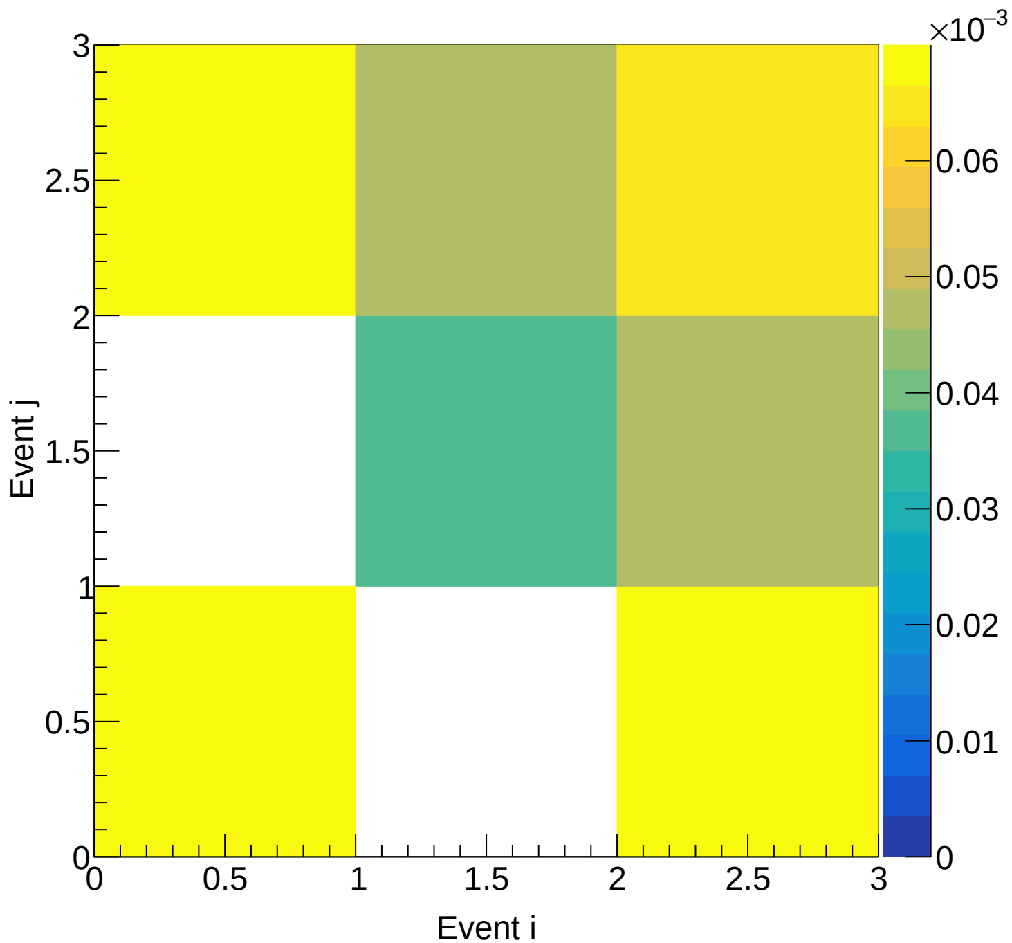
Flask (total) Covariance | M: [4.8, 5.1) xF: [0.00, 0.05)
