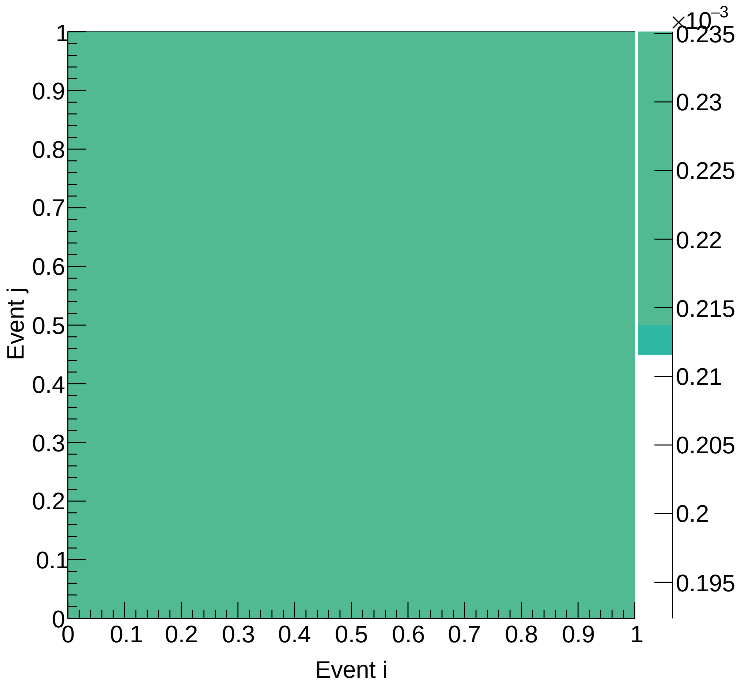
Flask (total) Covariance | M: [4.8, 5.1) xF: [-0.05, 0.00)
