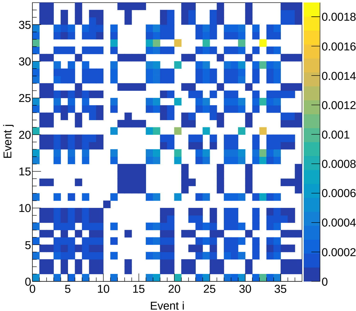
Flask (total) Covariance | M: [3.9, 4.2) xF: [0.45, 0.50)
