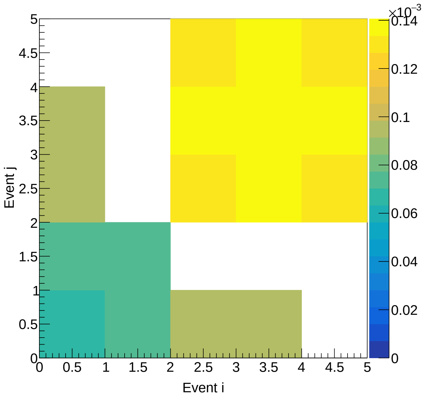
Flask (total) Covariance | M: [4.8, 5.1) xF: [0.45, 0.50)
