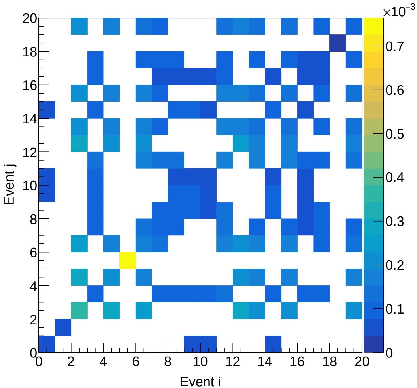
Flask (total) Covariance | M: [4.5, 4.8) xF: [0.50, 0.55)
