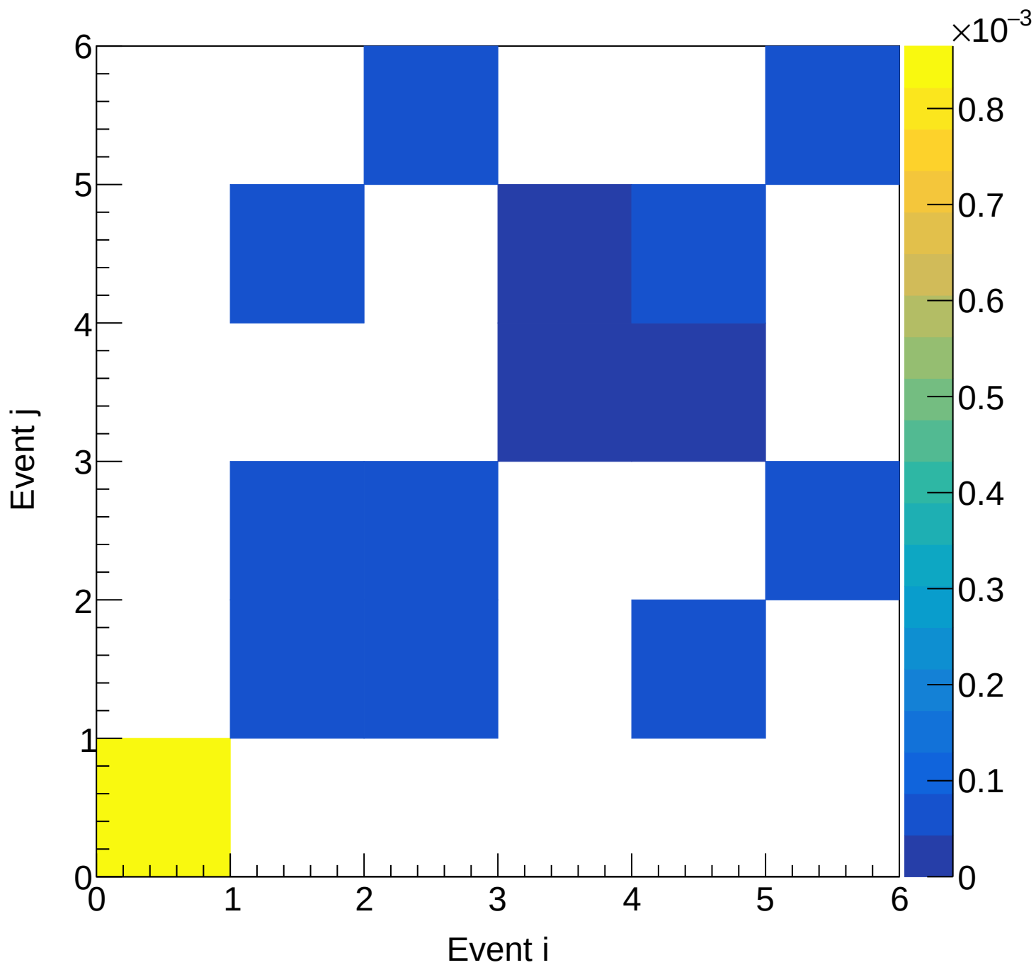
Flask (total) Covariance | M: [5.1, 5.4] xF: [0.50, 0.55)
