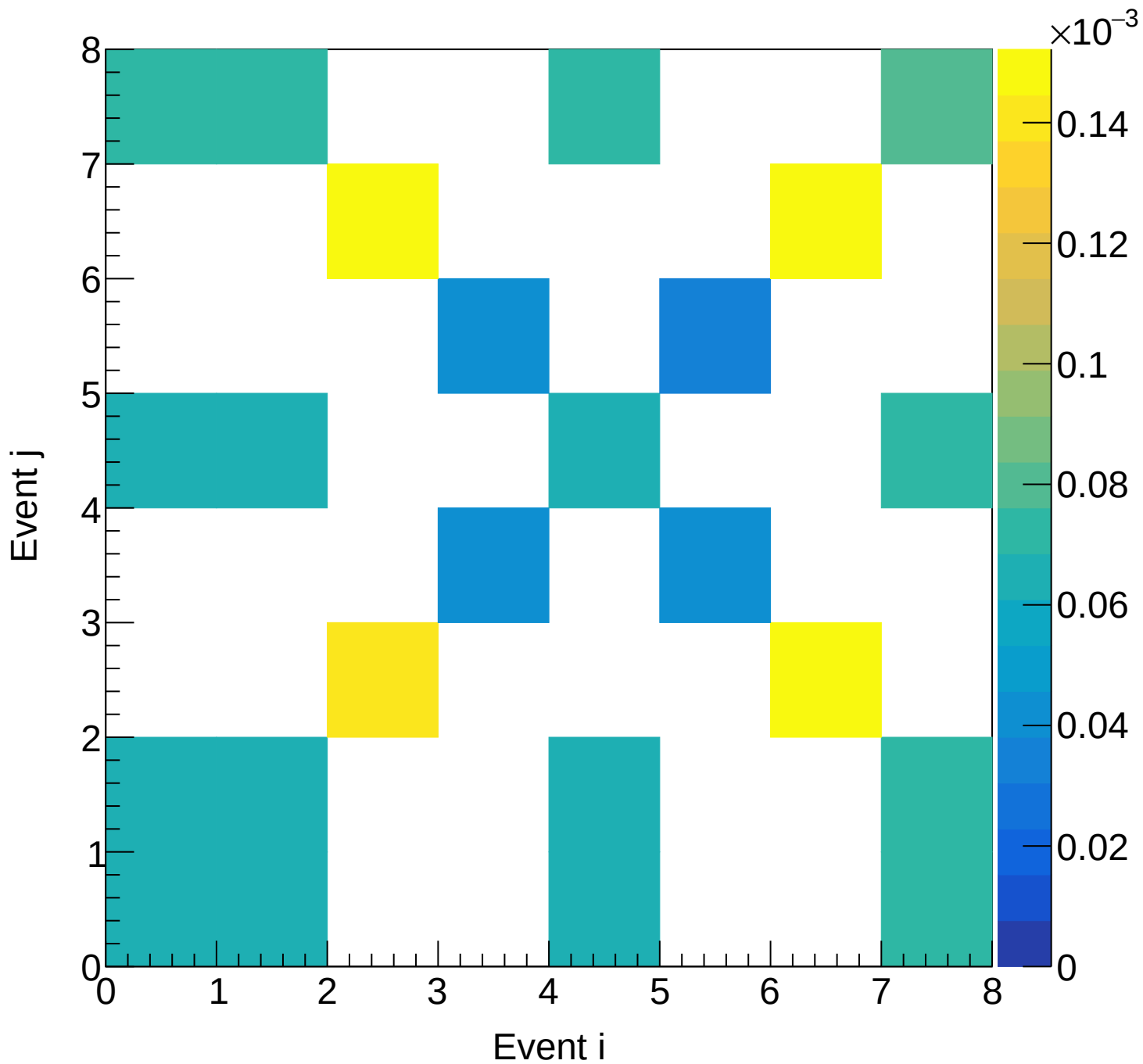
Flask (total) Covariance | M: [5.4, 5.7) xF: [0.50, 0.55)
