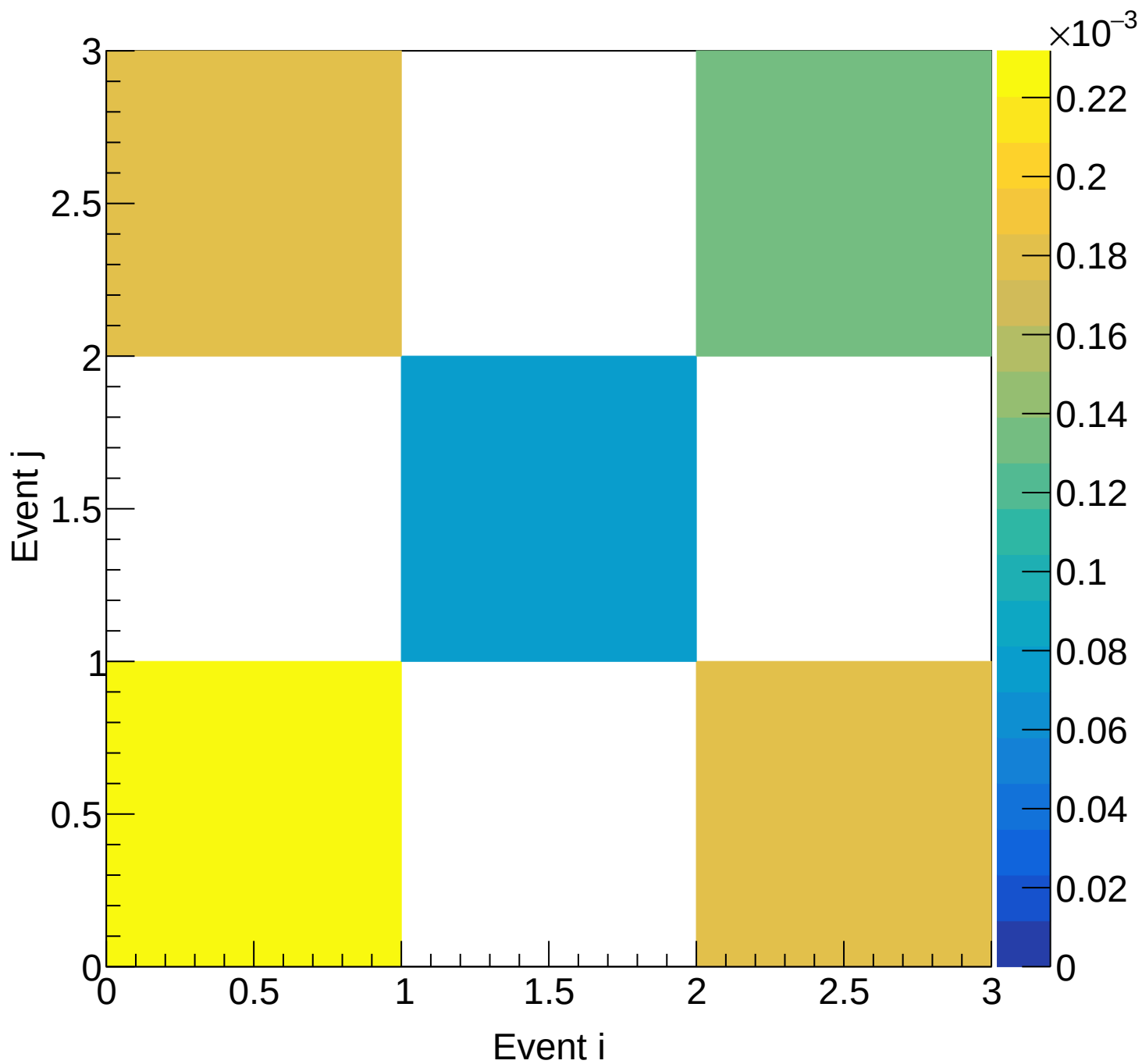
Flask (total) Covariance | M: [5.7, 6.0) xF: [0.50, 0.55)
