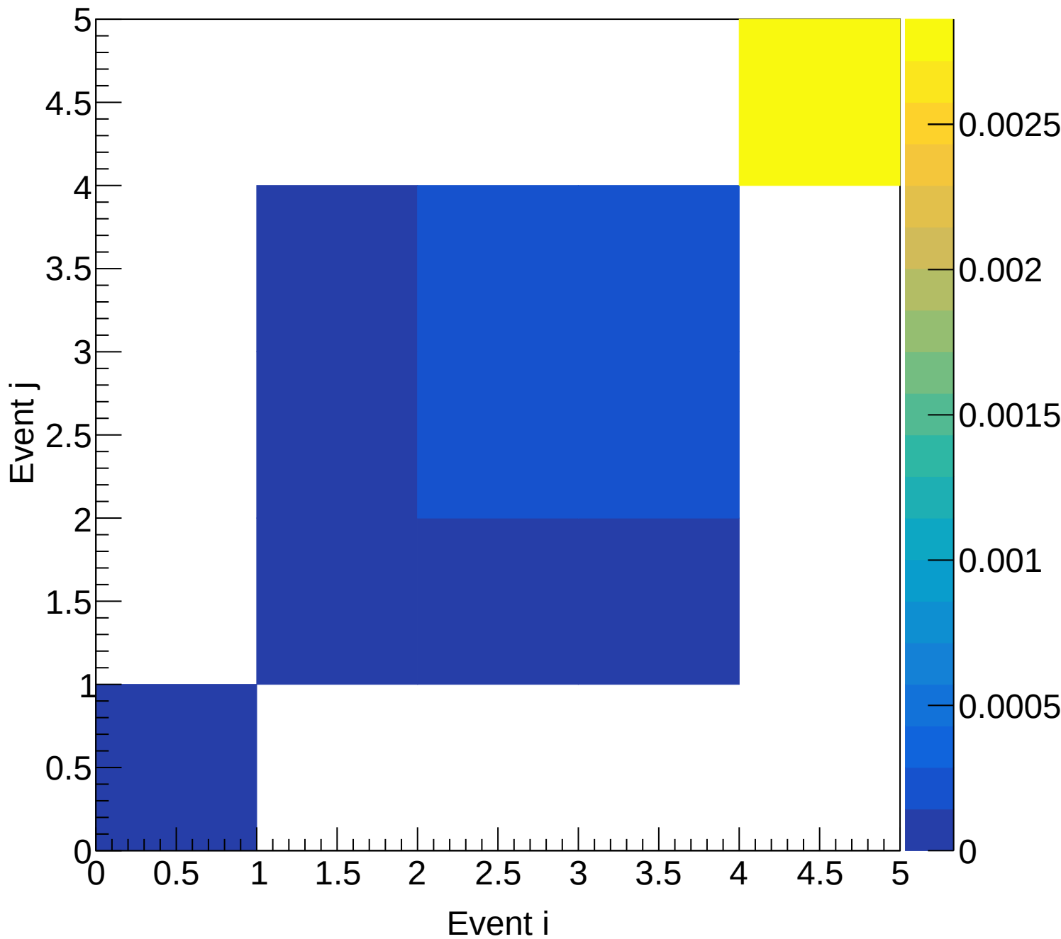
Flask (total) Covariance | M: [4.8, 5.1) xF: [0.55, 0.60)
