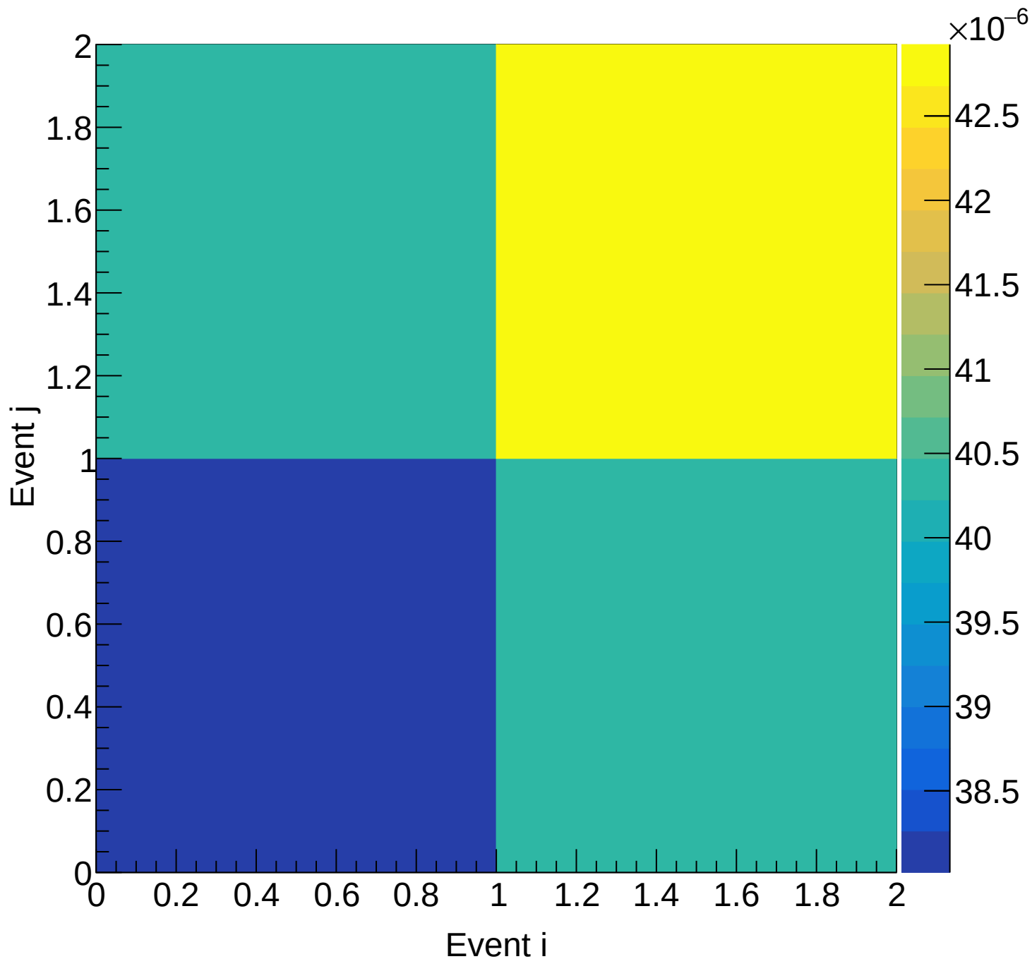
Flask (total) Covariance | M: [5.1, 5.4) xF: [0.55, 0.60)
