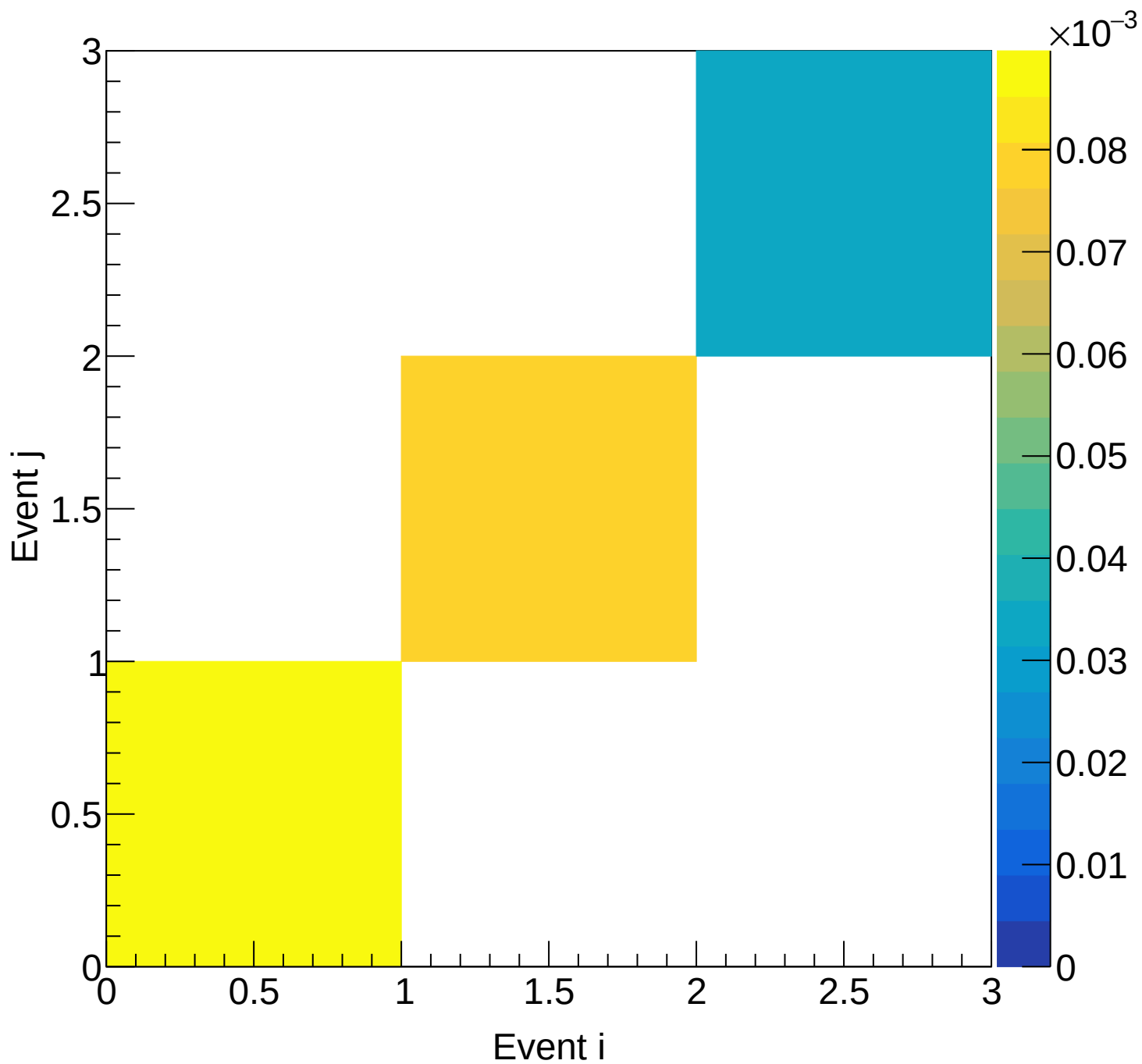
Flask (total) Covariance | M: [5.4, 5.7) xF: [0.55, 0.60)
