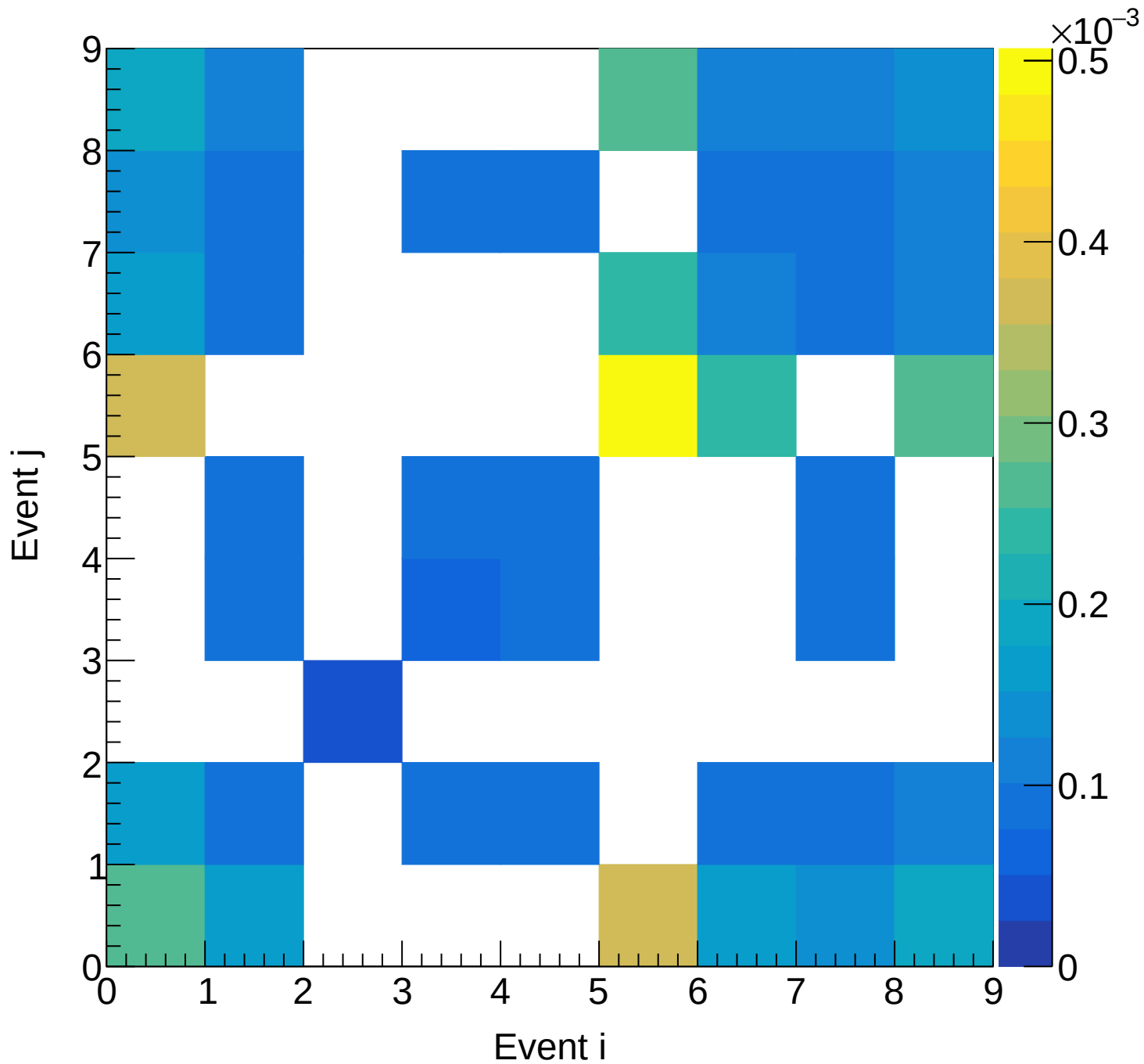
Flask (total) Covariance | M: [4.2, 4.5) xF: [0.60, 0.65)
