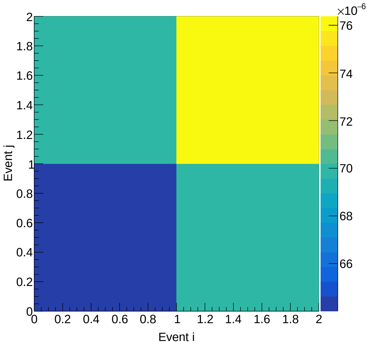
Flask (total) Covariance | M: [6.0, 6.3) xF: [0.60, 0.65)
